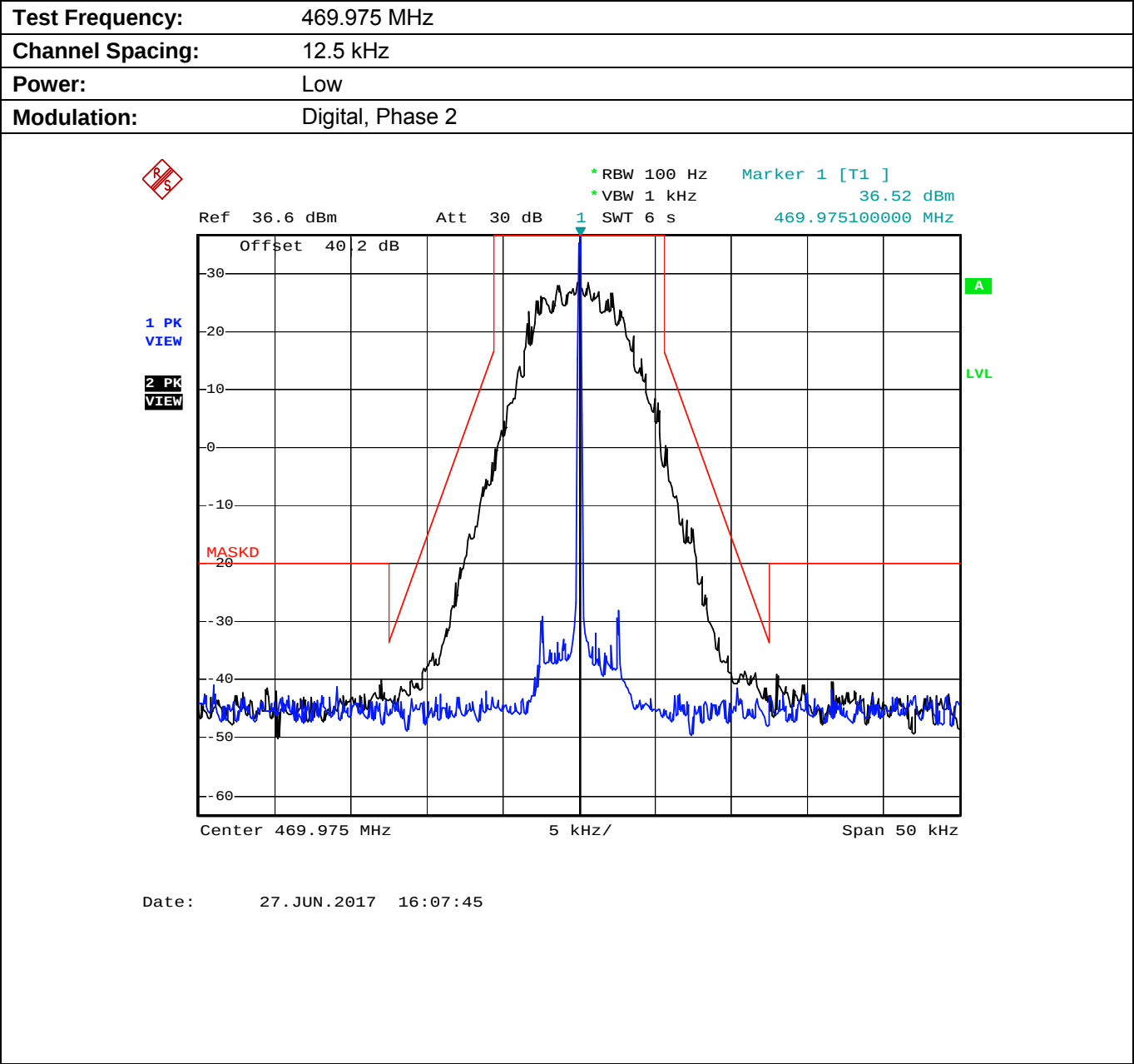
Plot 5.8.4.2.18. Emission Mask D, Low Power
