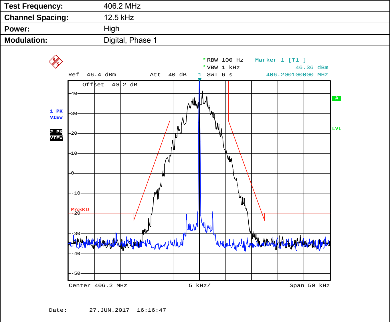
Plot 5.8.4.2.7. Emission Mask D, High Power
