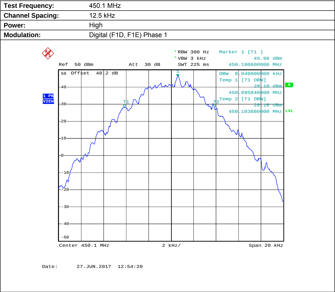
Plot 5.8.4.1.8. Occupied Bandwidth
