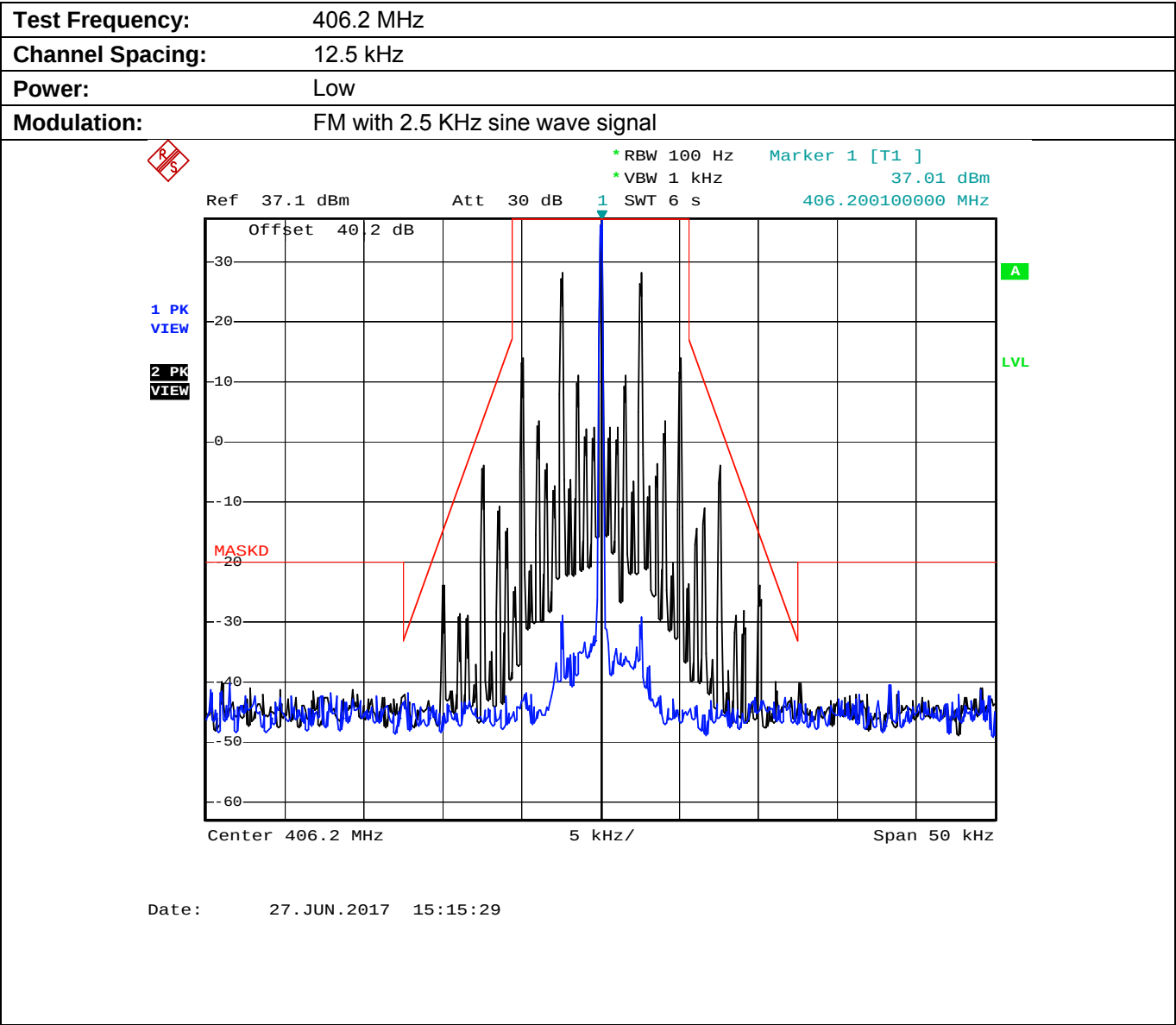
Plot 5.8.4.2.4. Emission Mask D, Low Power
