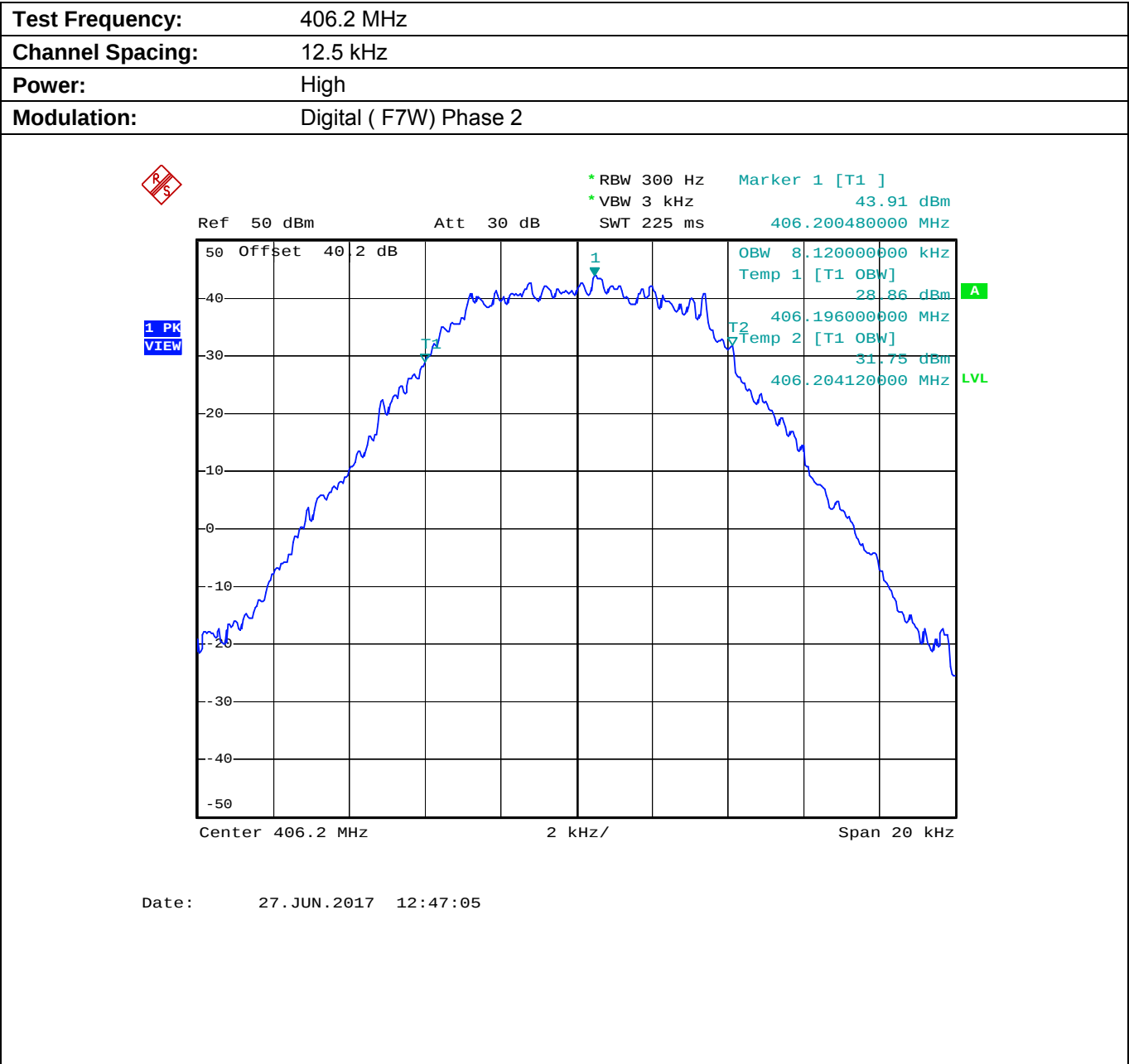
Plot 5.8.4.1.10. Occupied Bandwidth
