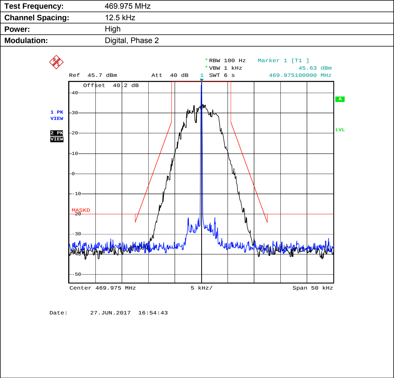
Plot 5.8.4.2.15. Emission Mask D, High Power
