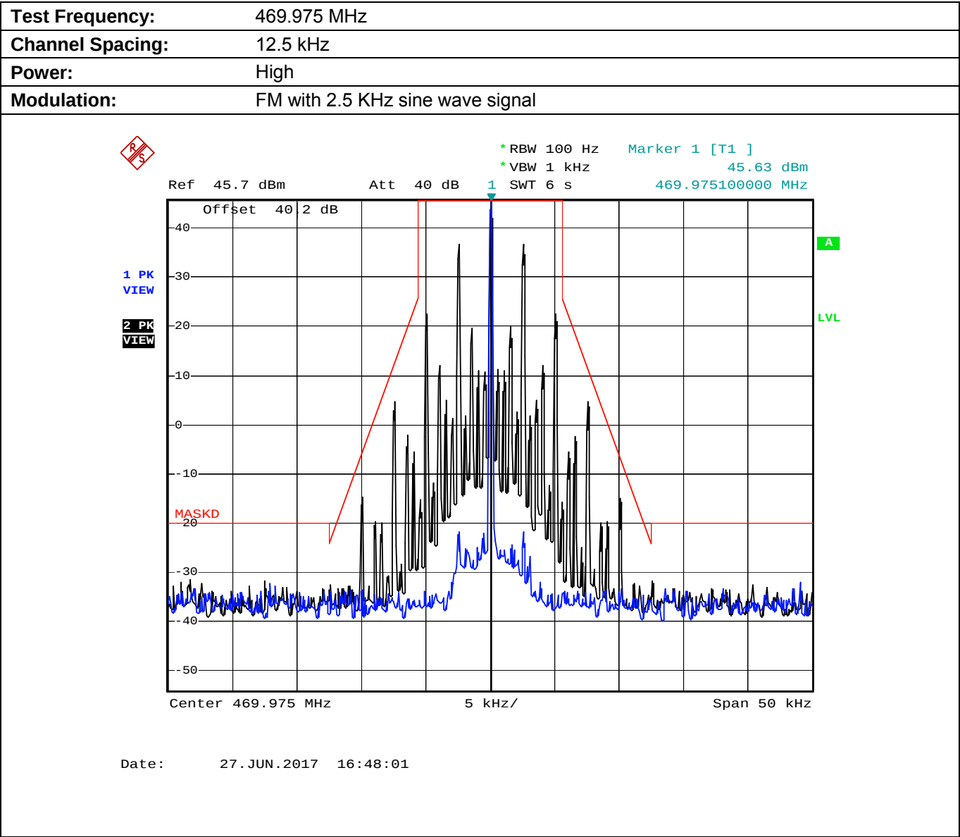
Plot 5.8.4.2.3. Emission Mask D, High Power
