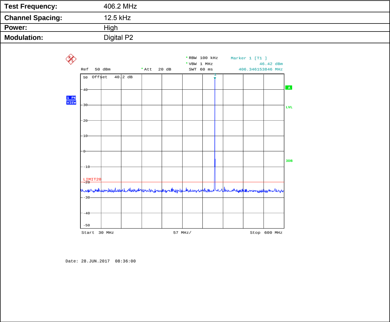
Plot 5.9.4.1.1. Conducted Transmitter Spurious Emissions for 406.2 MHz, High Power,
