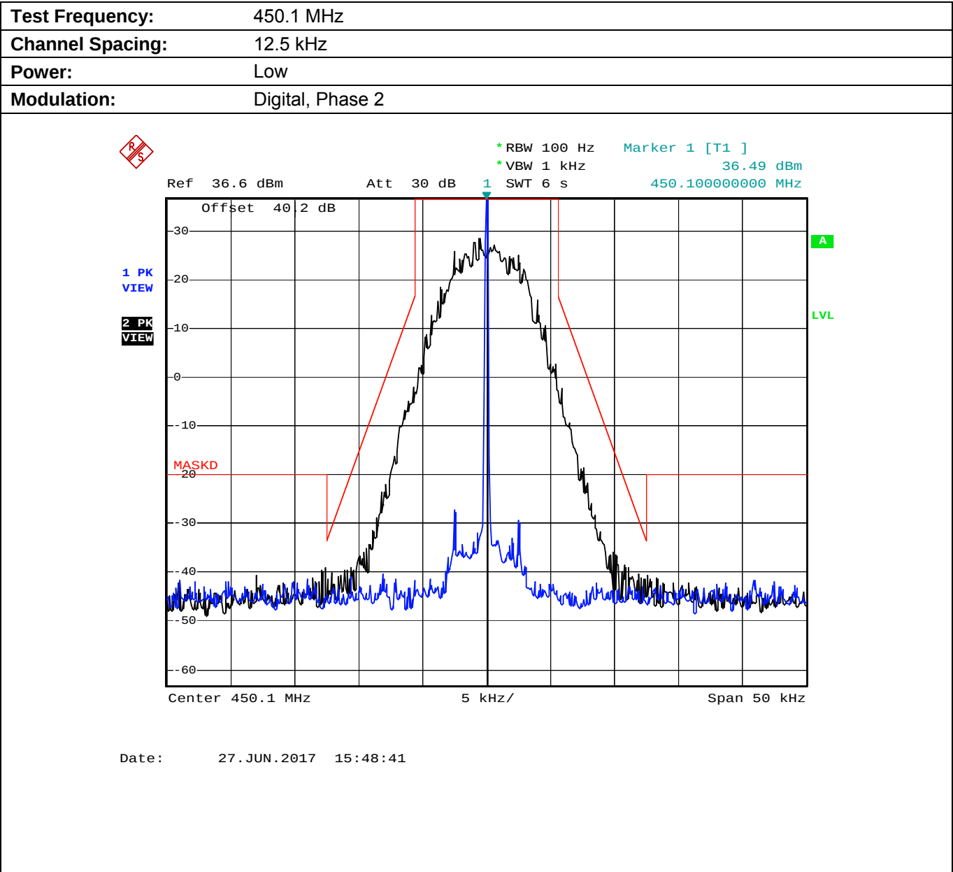
Plot 5.8.4.2.17. Emission Mask D, Low Power
