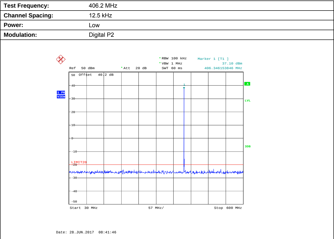
Plot 5.9.4.1.2. Conducted Transmitter Spurious Emissions for 406.2 MHz, Low Power
