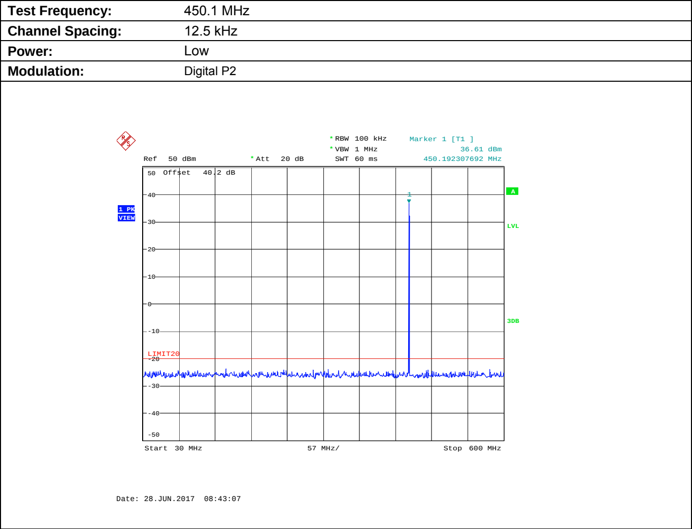
Plot 5.9.4.2.2. Conducted Transmitter Spurious Emissions for 450.1 MHz, Low Power
