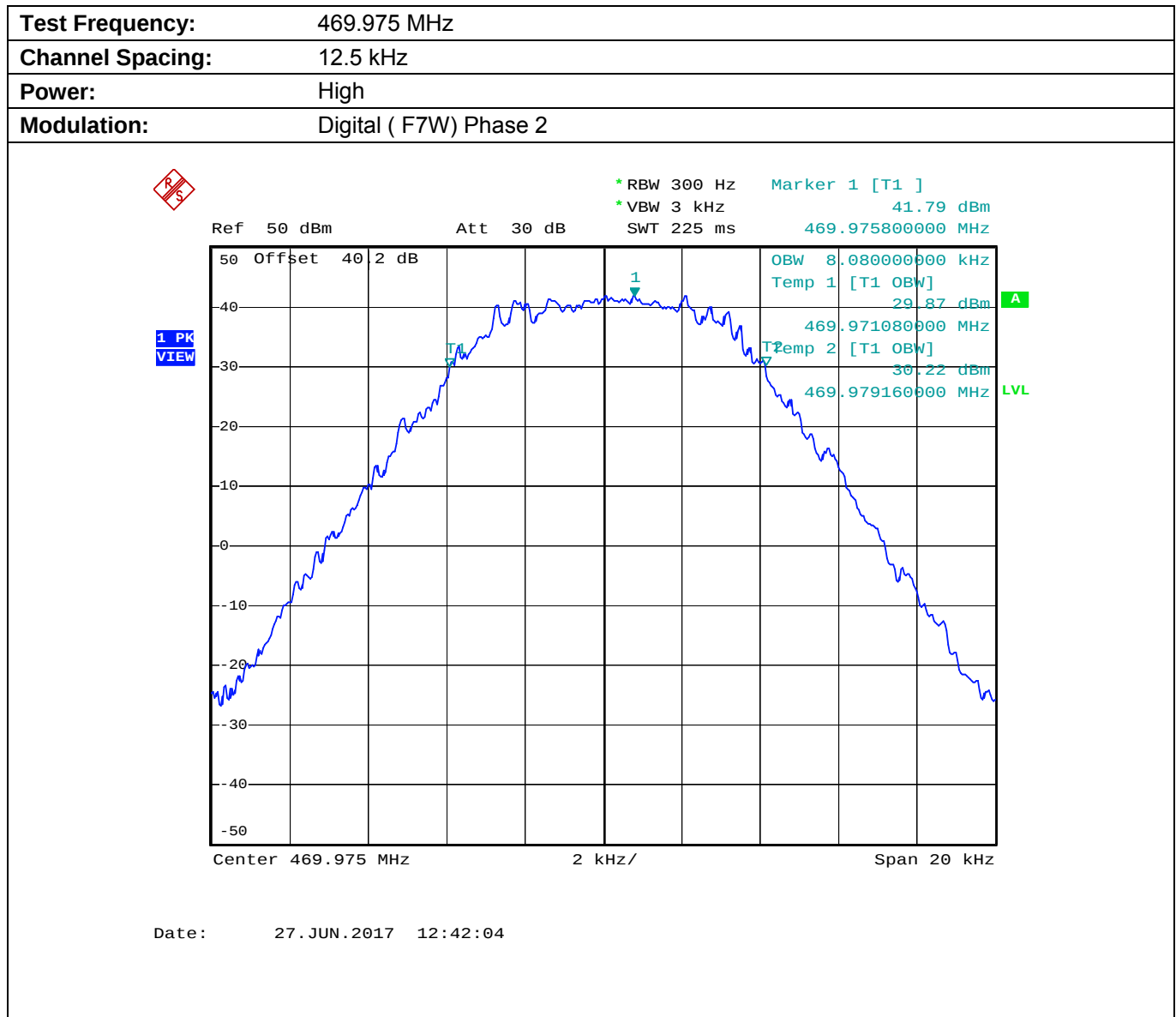
Plot 5.8.4.1.12. Occupied Bandwidth
