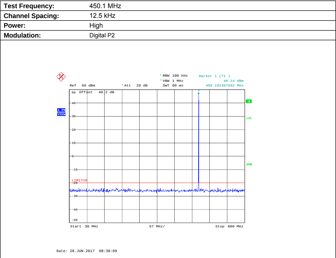
Plot 5.9.4.2.1. Conducted Transmitter Spurious Emissions for 450.1 MHz, High Power
