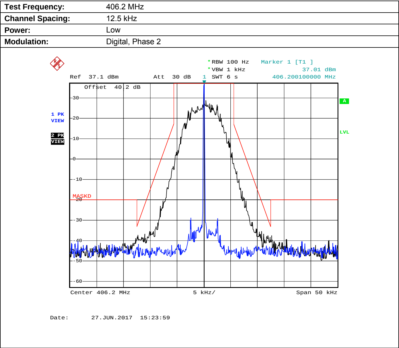
Plot 5.8.4.2.16. Emission Mask D, Low Power
