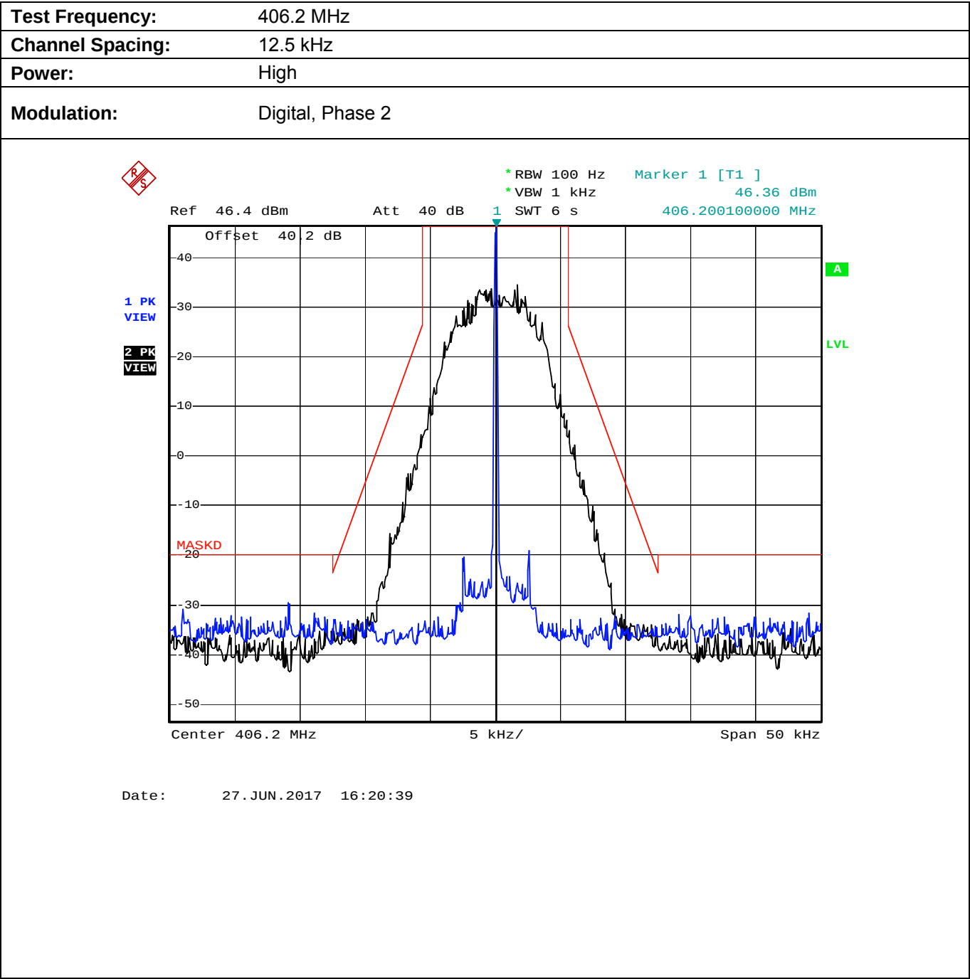
Plot 5.8.4.2.13. Emission Mask D, High Power
