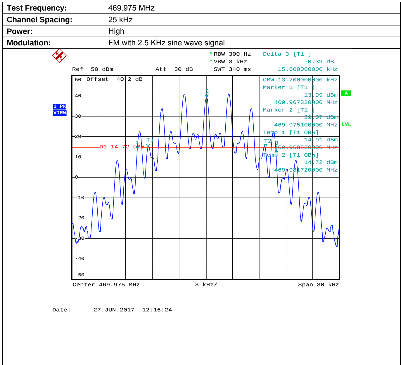
Plot 5.8.4.1.3. Occupied Bandwidth
