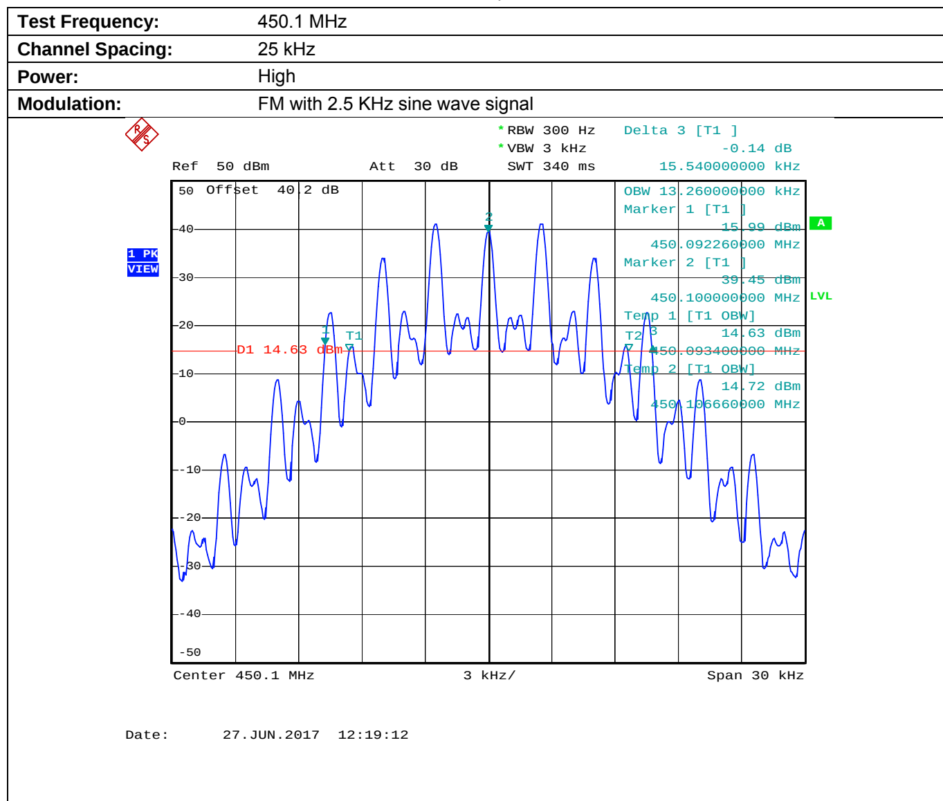
Plot 5.8.4.1.2. Occupied Bandwidth
