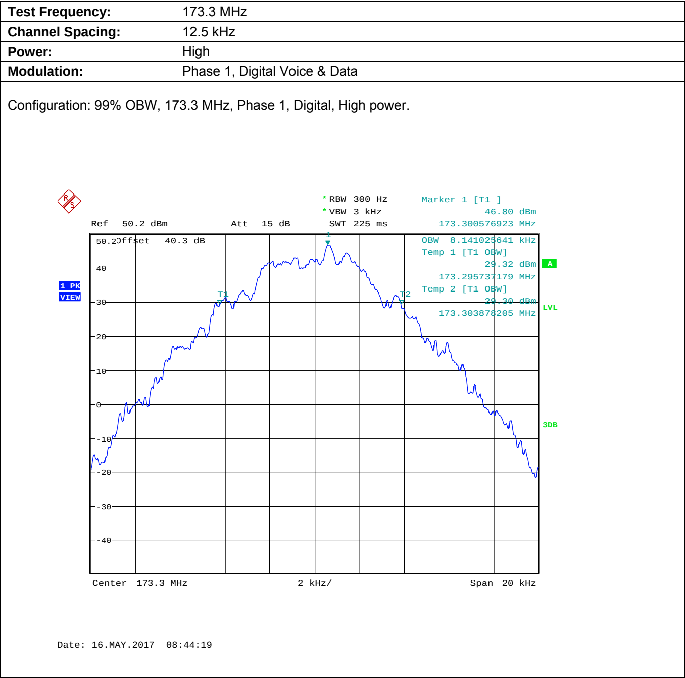
Plot 5.8.4.1.9. Occupied Bandwidth
