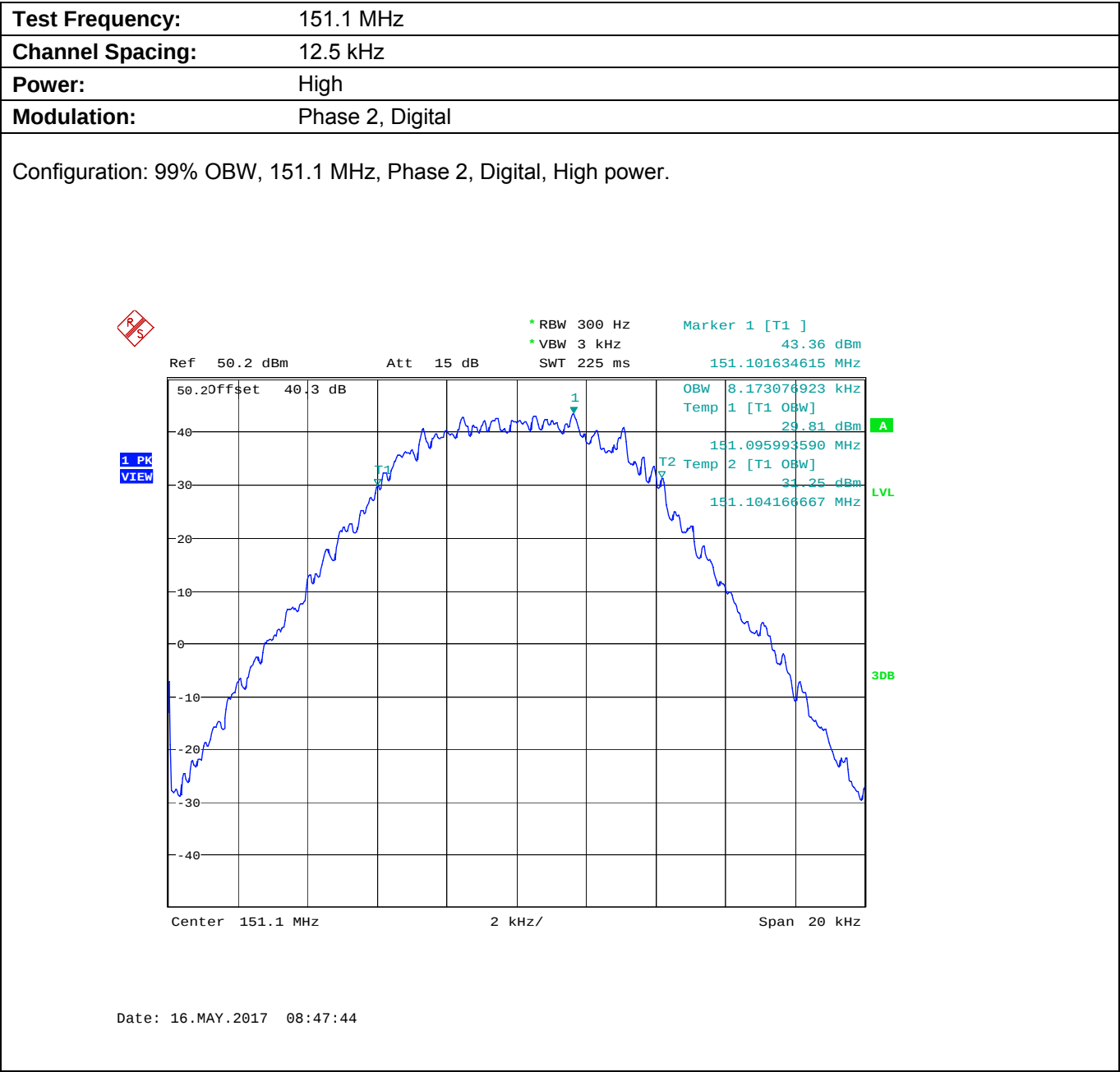
Plot 5.8.4.1.11. Occupied Bandwidth
