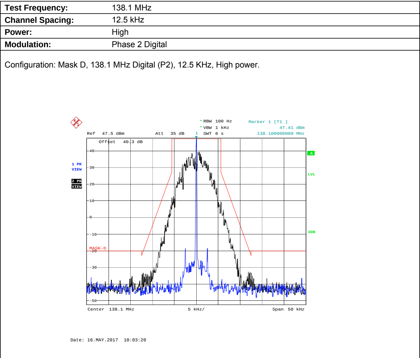
Plot 5.8.4.2.13. Emission Mask D, High Power
