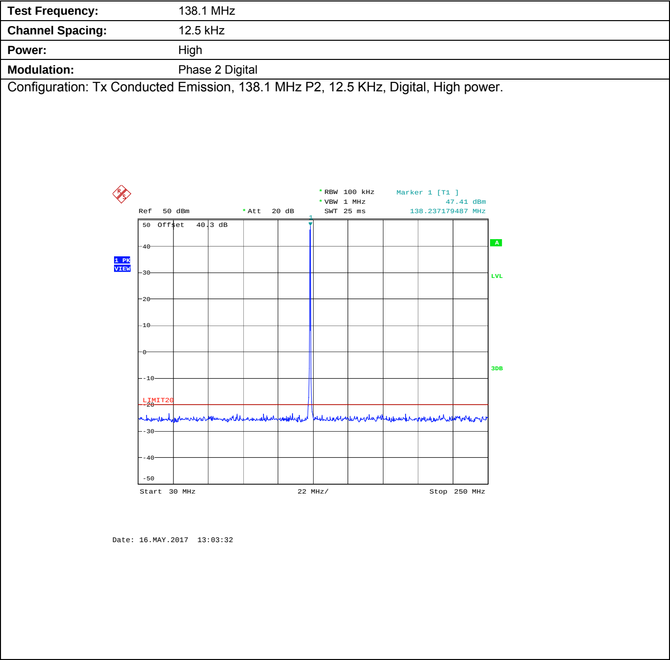
Plot 5.9.4.1.1. Conducted Transmitter Spurious Emissions for 138.1 MHz, High Power
