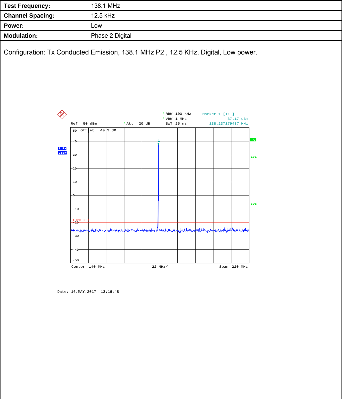
Plot 5.9.4.1.2. Conducted Transmitter Spurious Emissions for 138.1 MHz, Low Power
