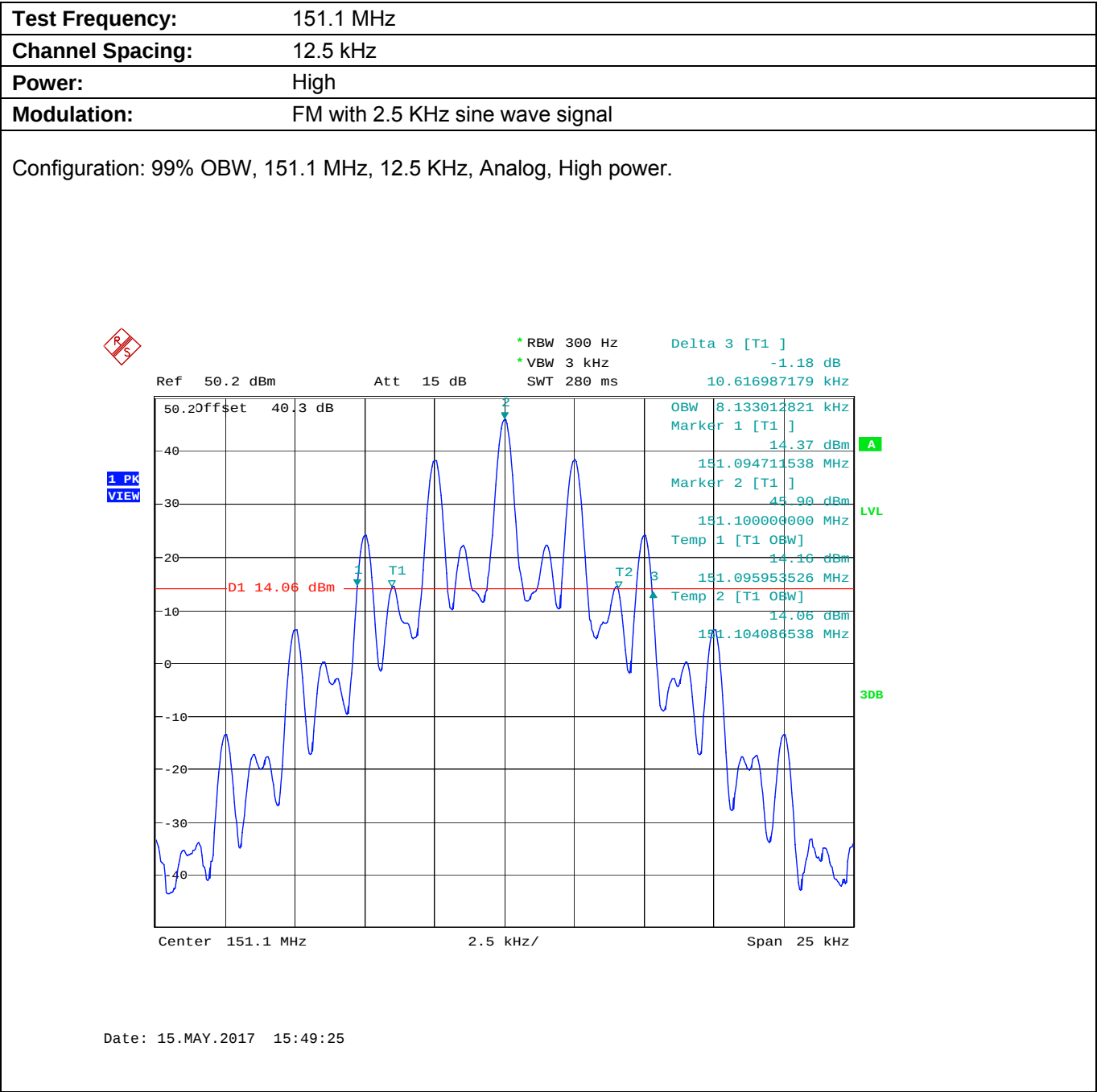
Plot 5.8.4.1.5. Occupied Bandwidth
