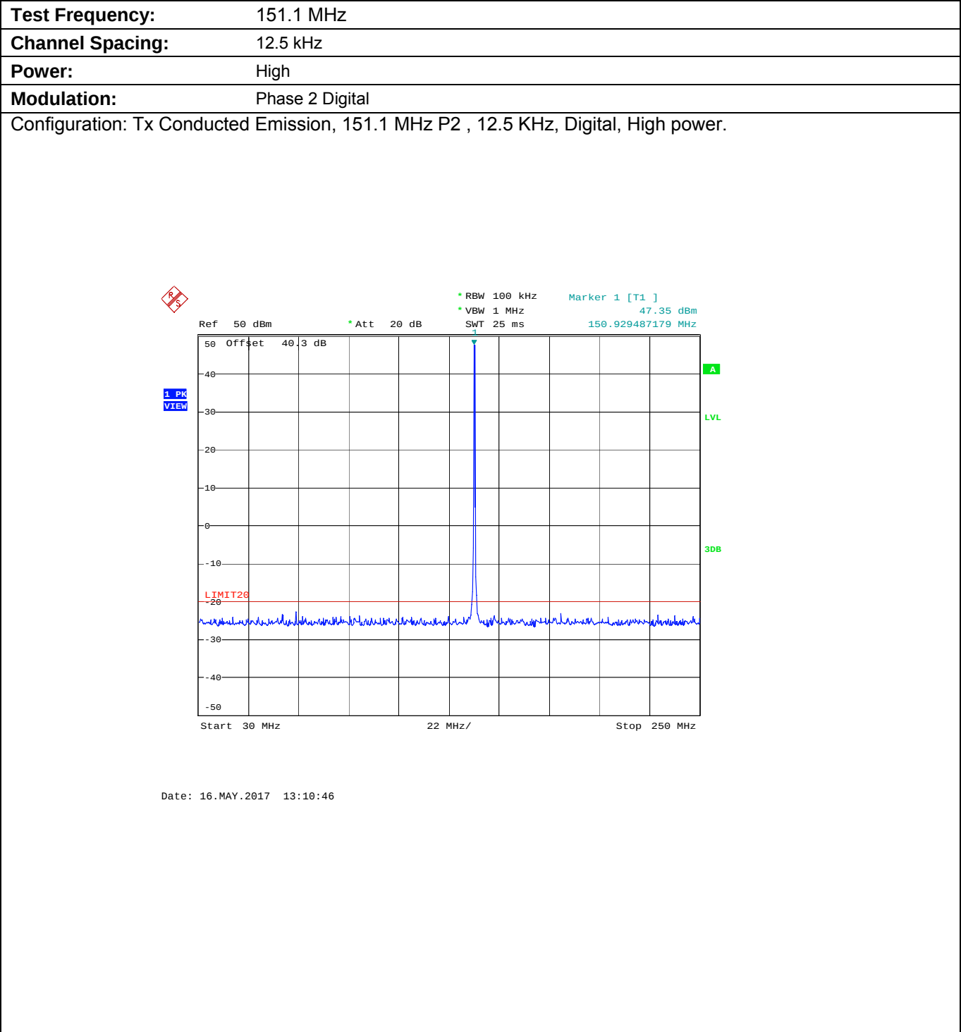
Plot 5.9.4.2.1. Conducted Transmitter Spurious Emissions for 151.1 MHz, High Power
