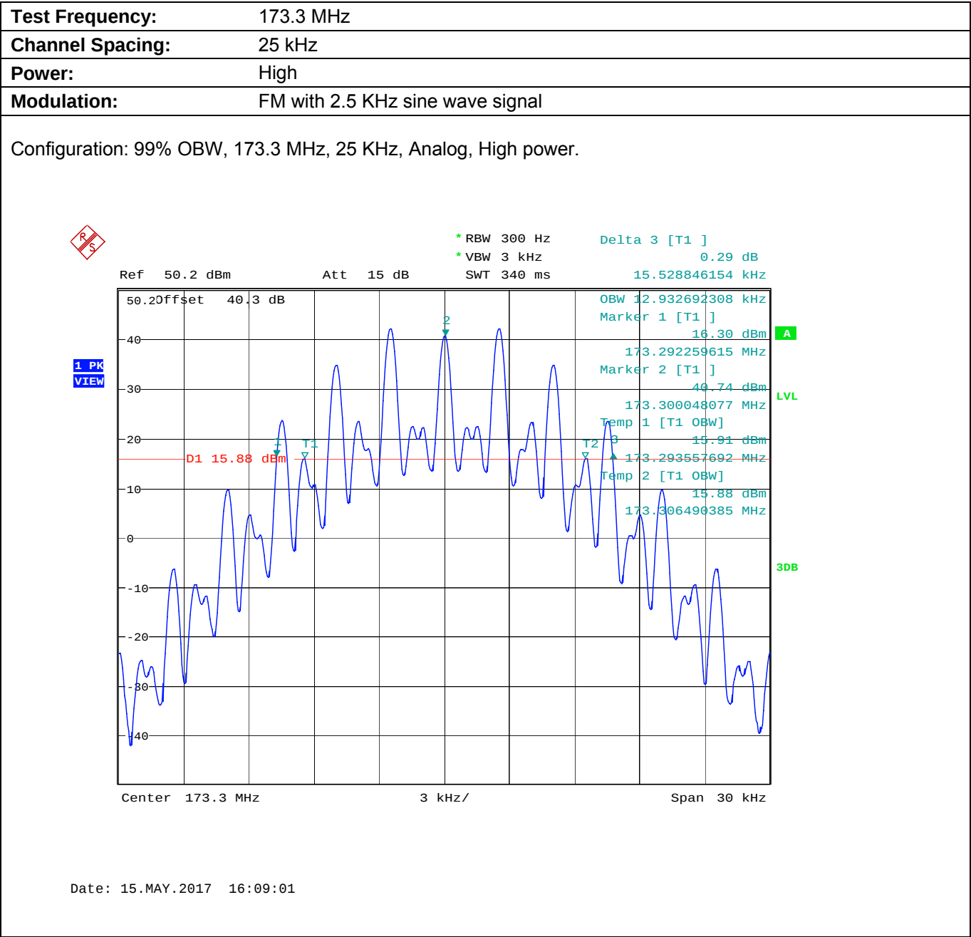
Plot 5.8.4.1.3. Occupied Bandwidth
