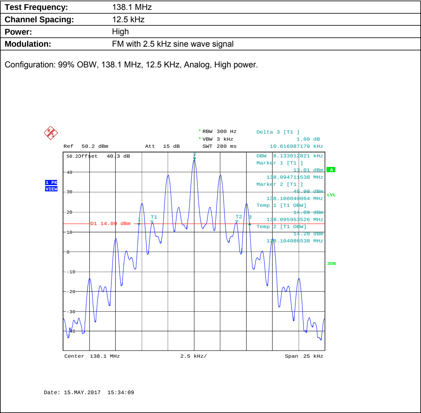
Plot 5.8.4.1.4. Occupied Bandwidth
