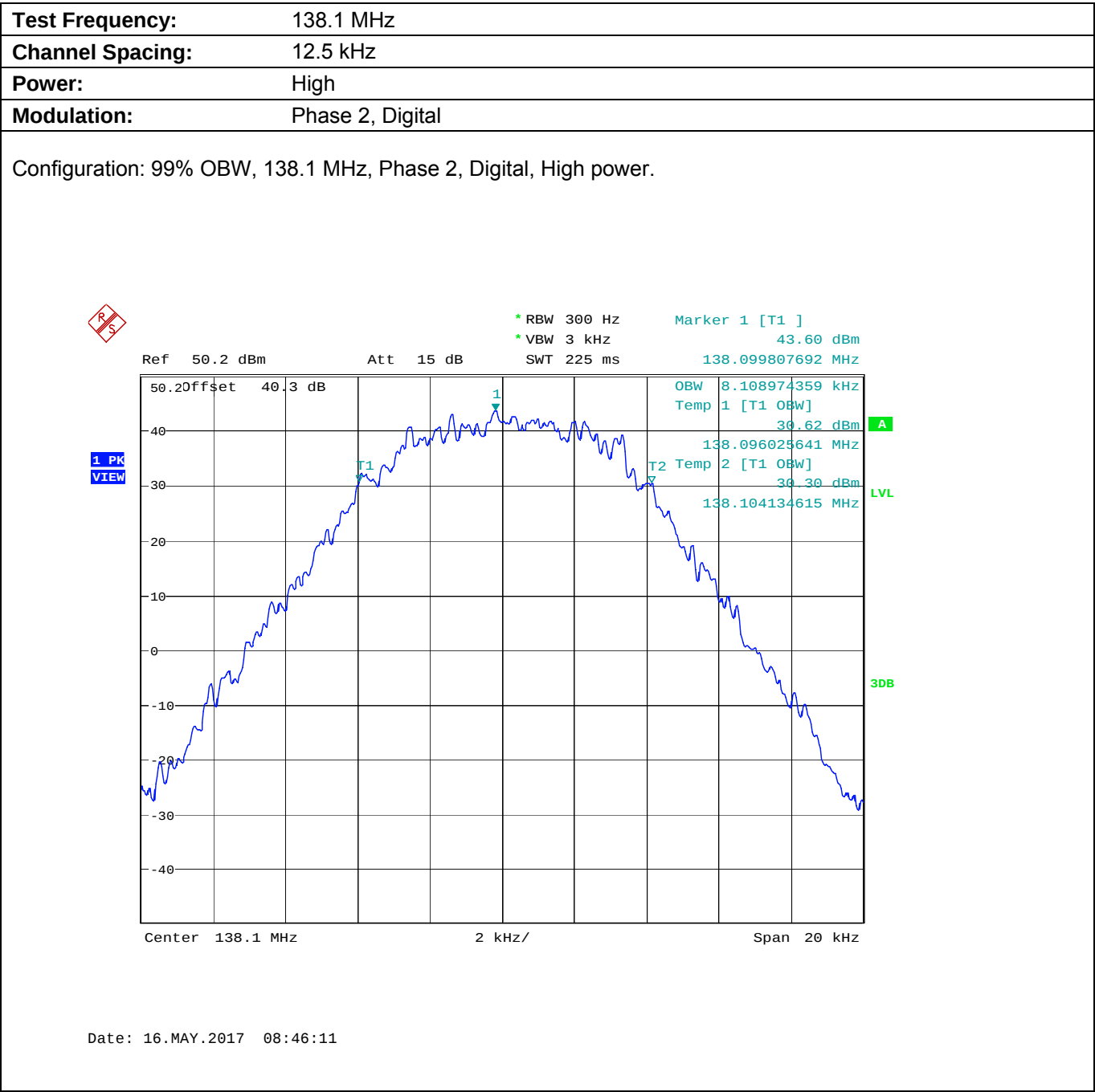
Plot 5.8.4.1.10. Occupied Bandwidth
