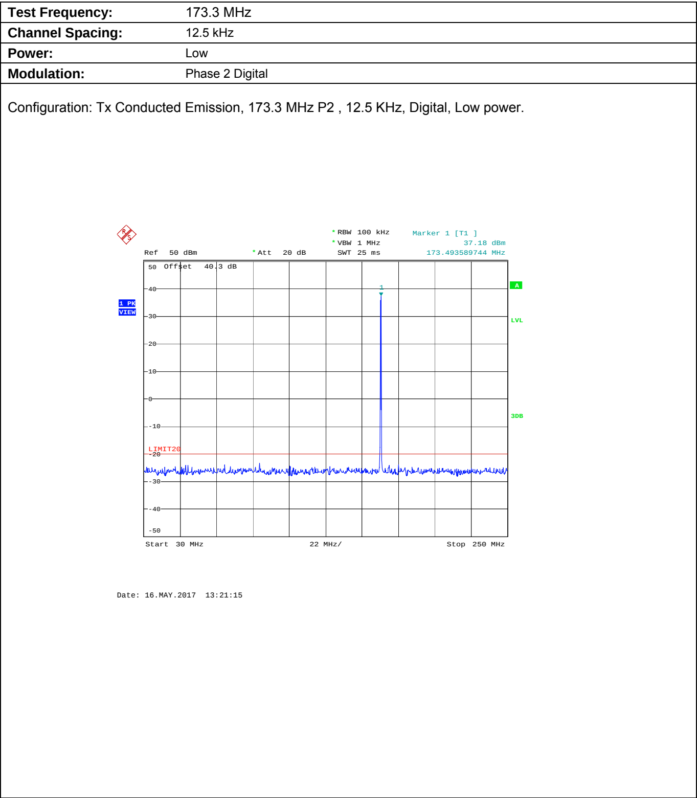
Plot 5.9.4.3.2. Conducted Transmitter Spurious Emissions for 173.3 MHz, Low Power, 30 MHz - 250 MHz
