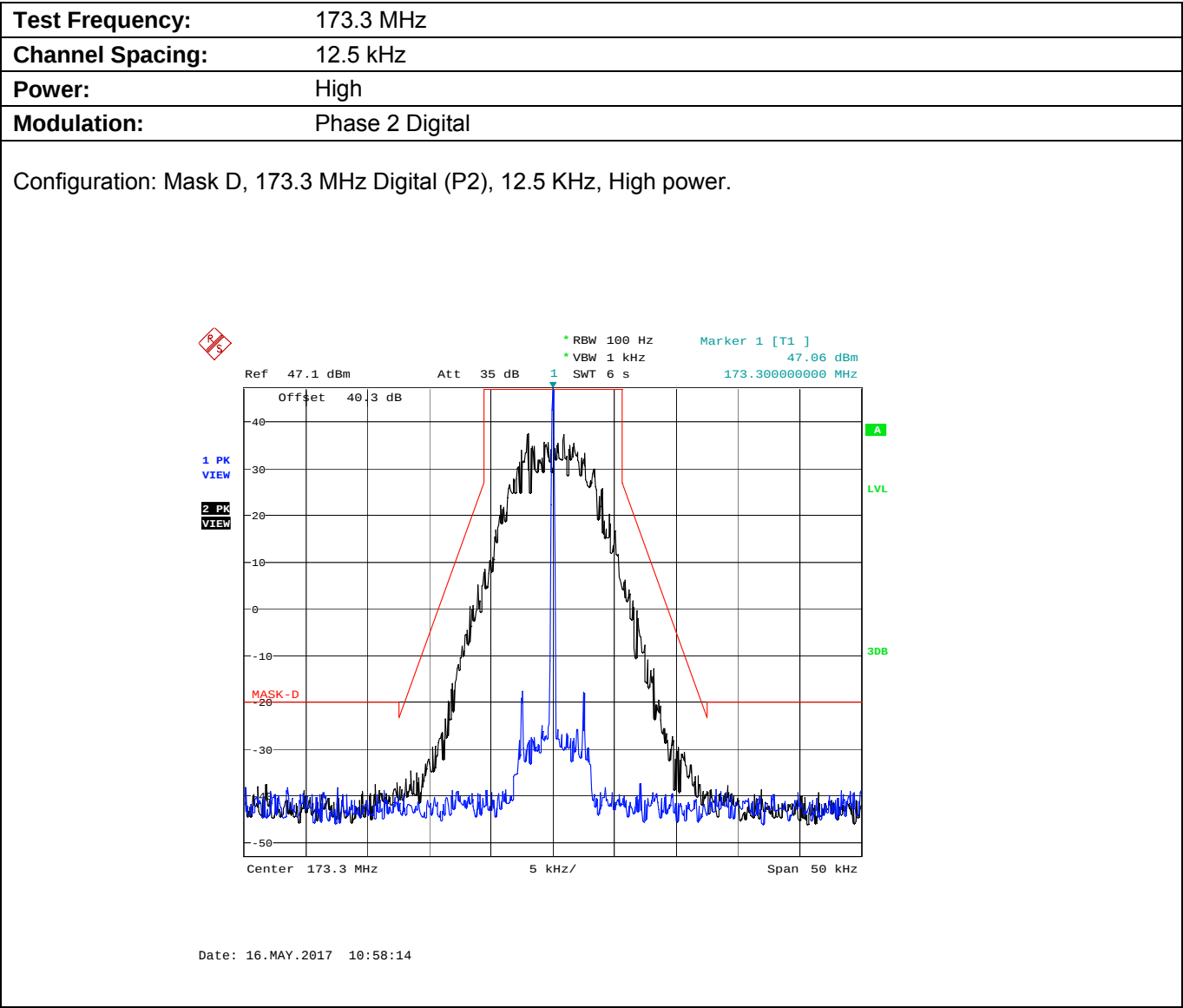
Plot 5.8.4.2.15. Emission Mask D, High Power
