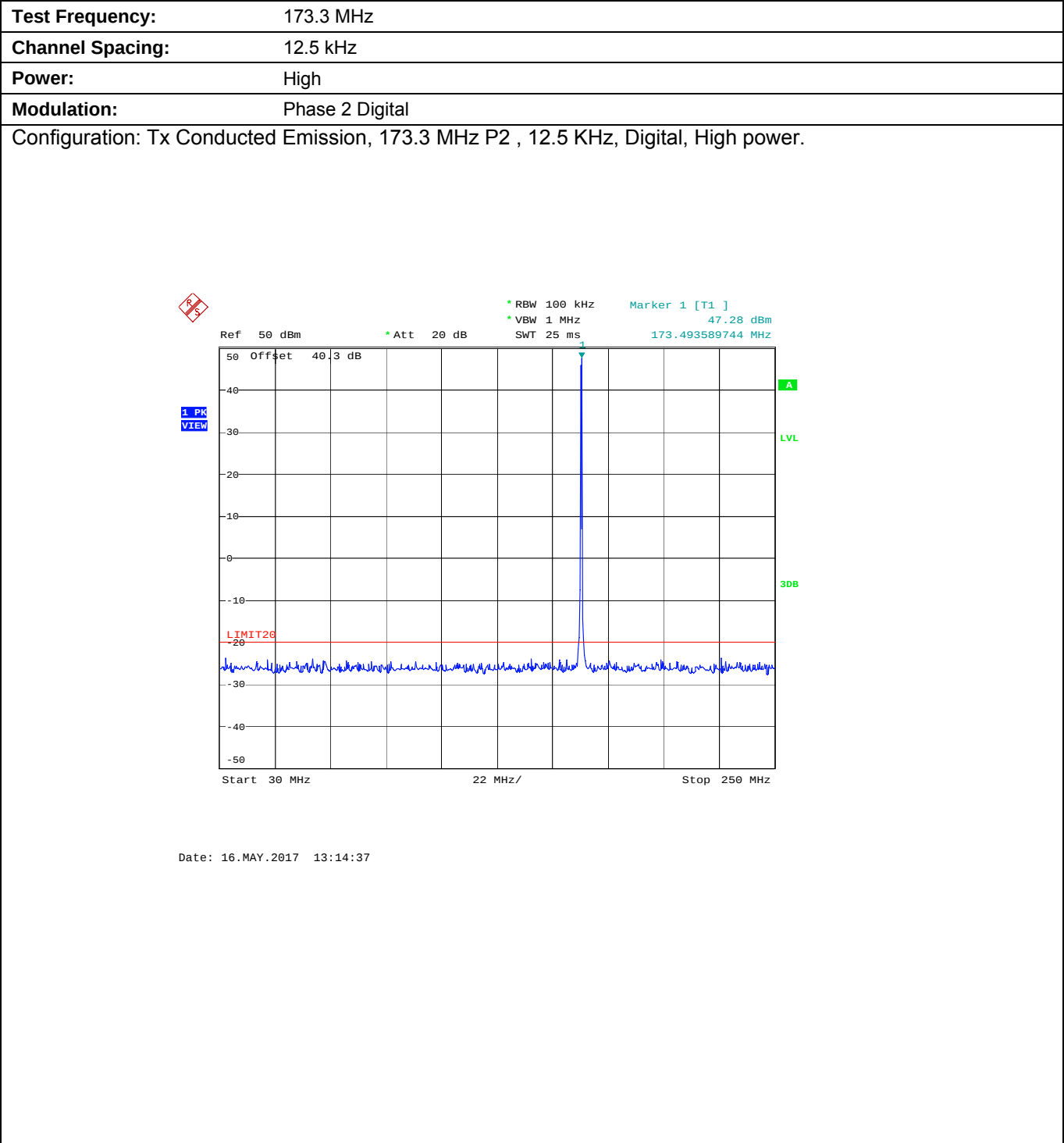
Plot 5.9.4.3.1. Conducted Transmitter Spurious Emissions for 173.3 MHz, High Power, 30 MHz - 250 MHz
