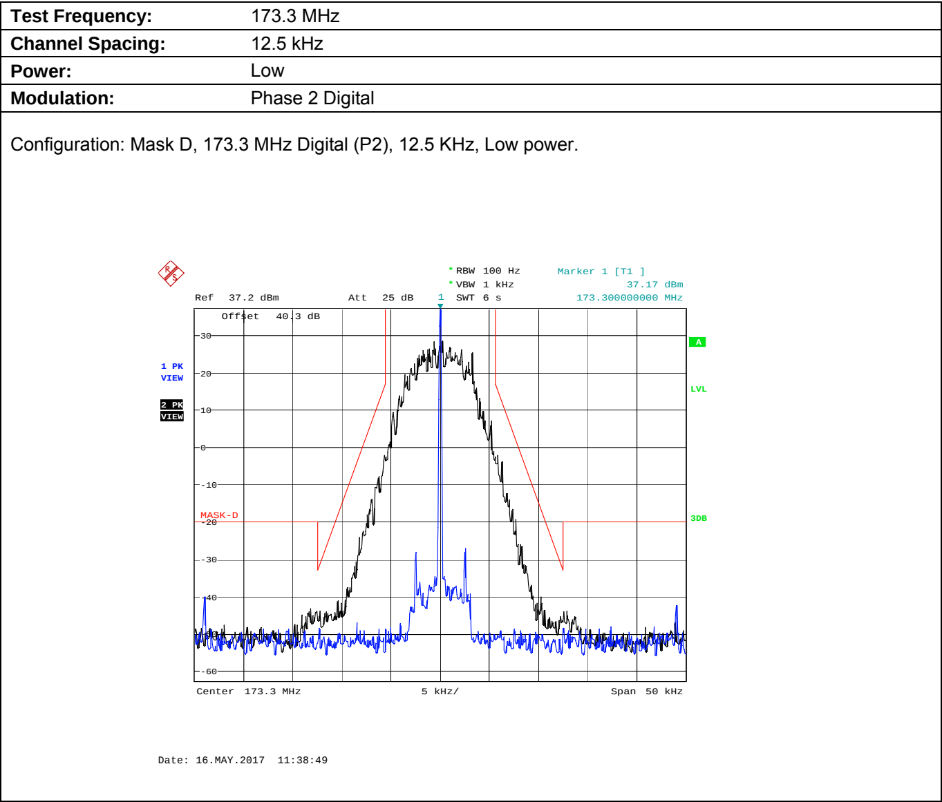
Plot 5.8.4.2.18. Emission Mask D, Low Power
