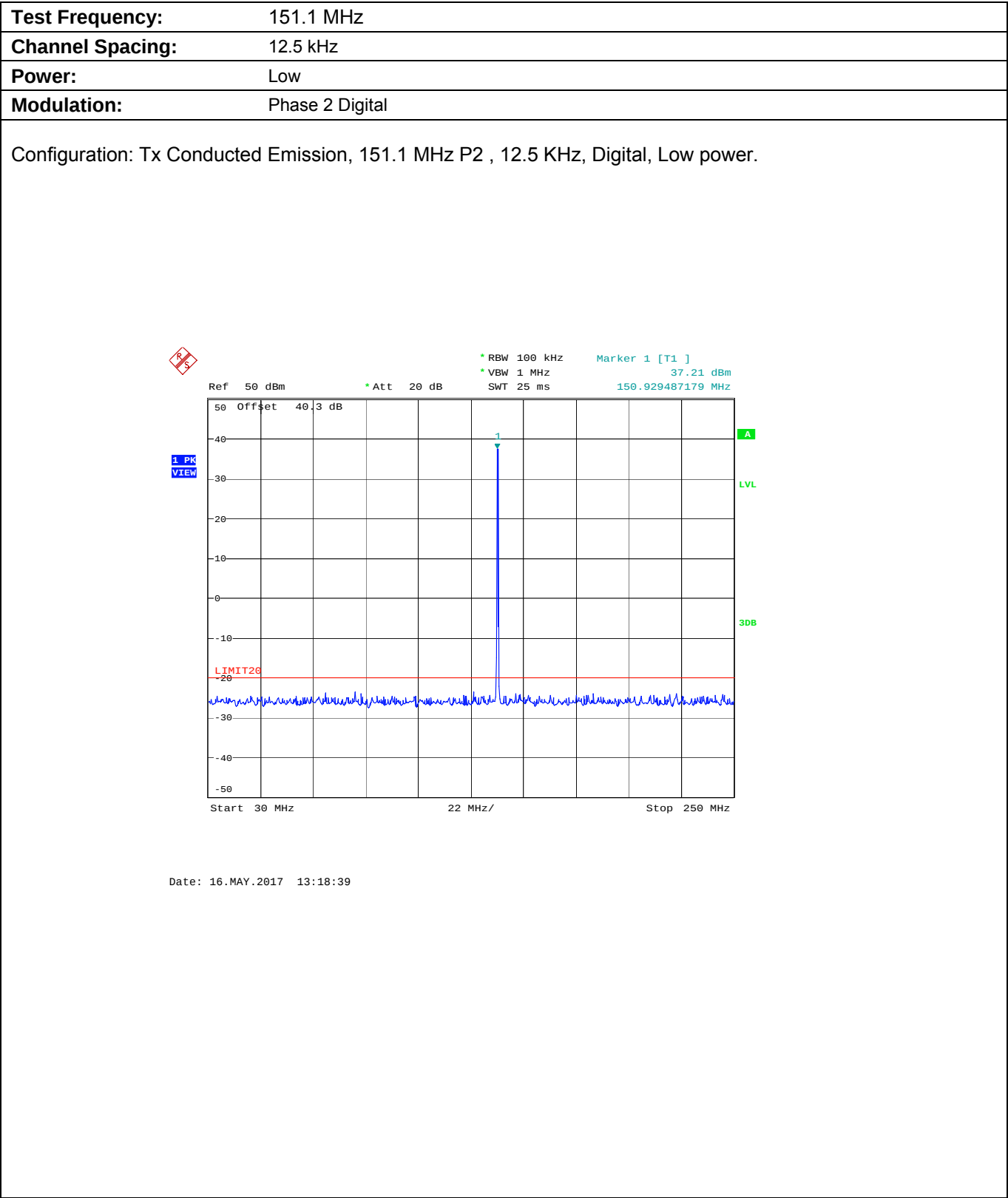
Plot 5.9.4.2.2. Conducted Transmitter Spurious Emissions for 151.1 MHz, Low Power
