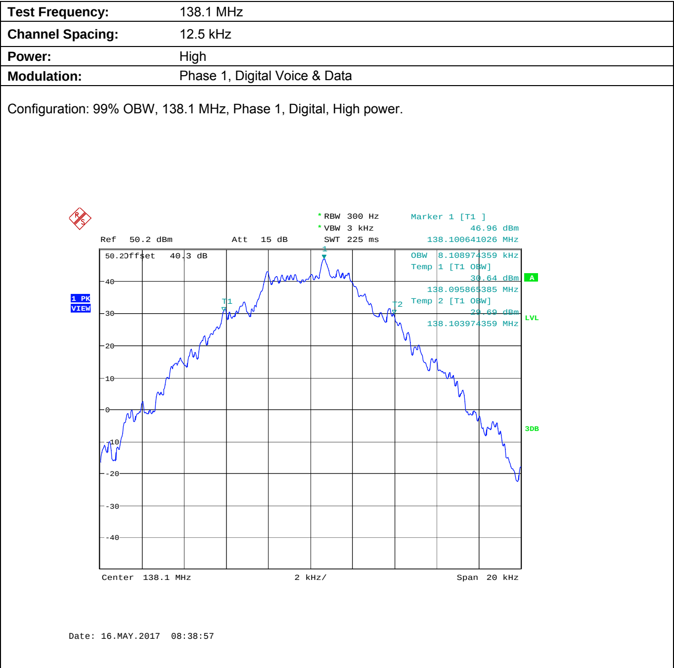
Plot 5.8.4.1.7. Occupied Bandwidth
