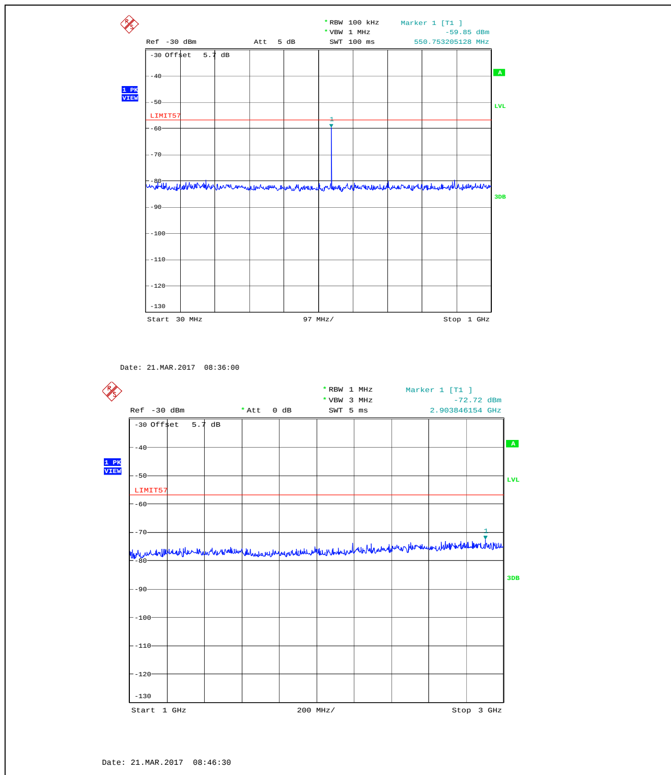
Plot 5.2.4.6. Receiver Antenna Power Conducted Emissions, 550 MHz
