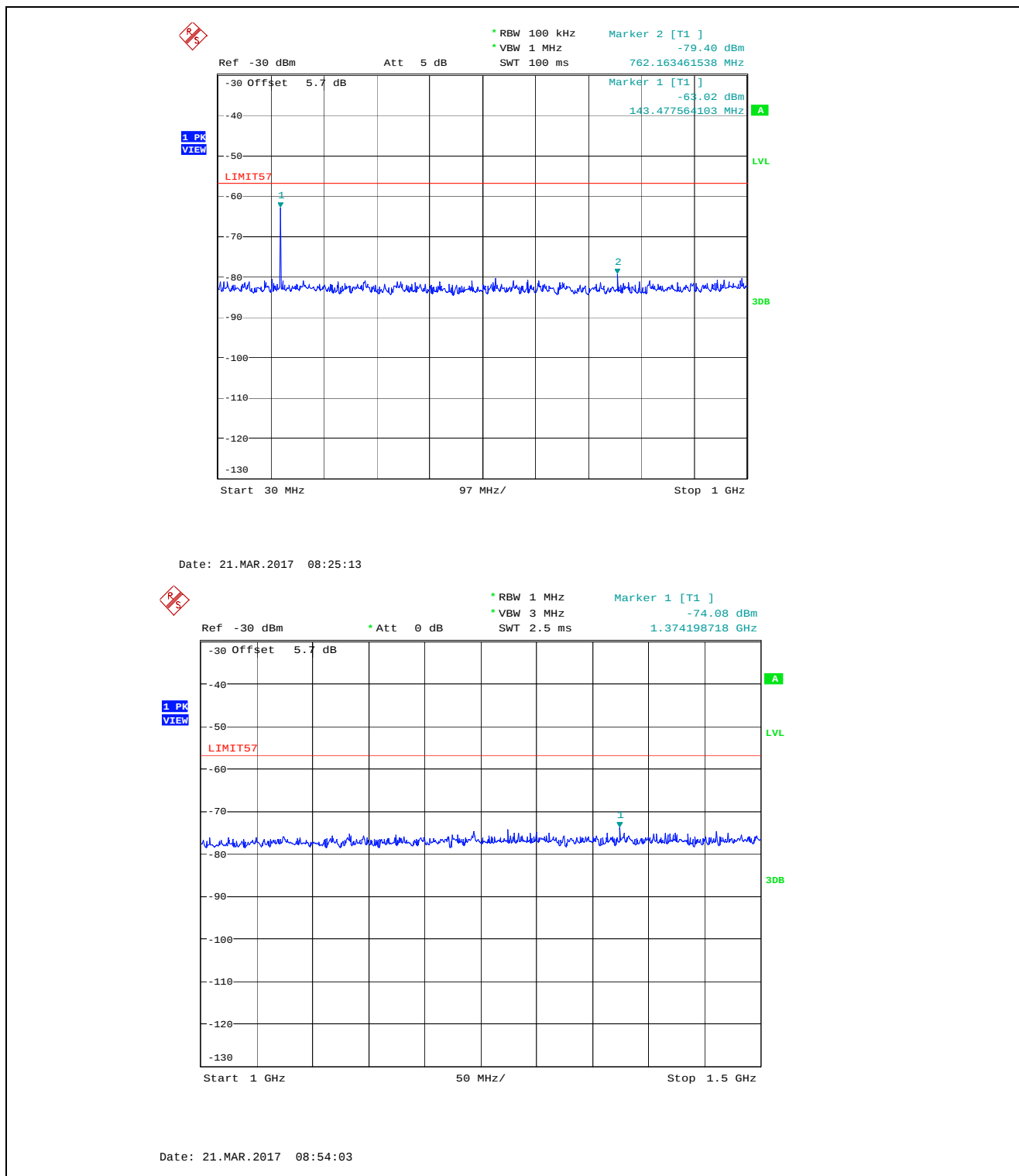
Plot 5.2.4.2. Receiver Antenna Power Conducted Emissions, 144 MHz
