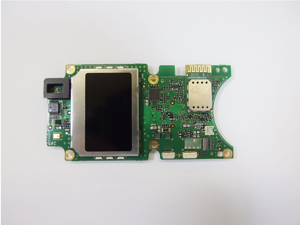
IC-F5330D MIC unit Logic-A board side-A
