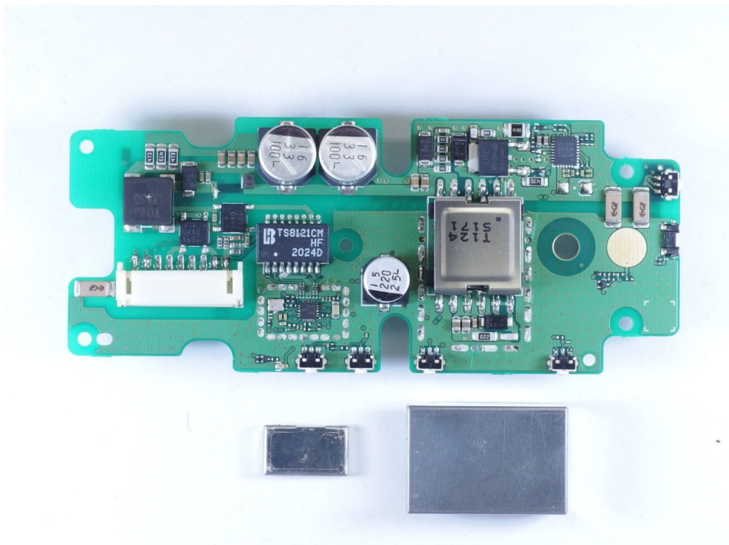
IC-F5330D MIC unit PD board side-B
