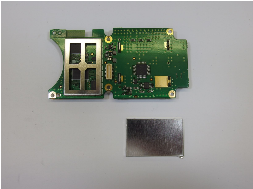
IC-F5330D MIC unit Logic-A board side-B
