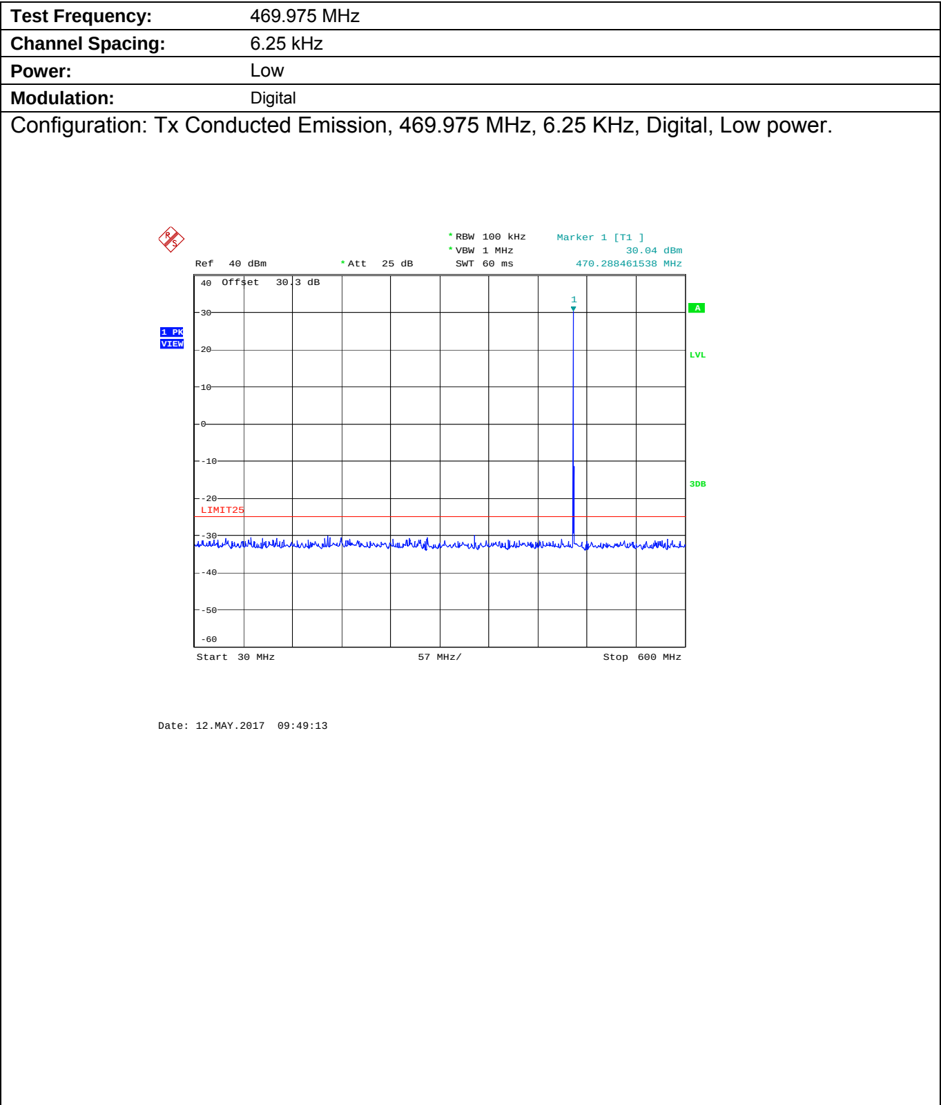
Plot 5.9.4.3.2. Conducted Transmitter Spurious Emissions for 469.975 MHz, Low Power
