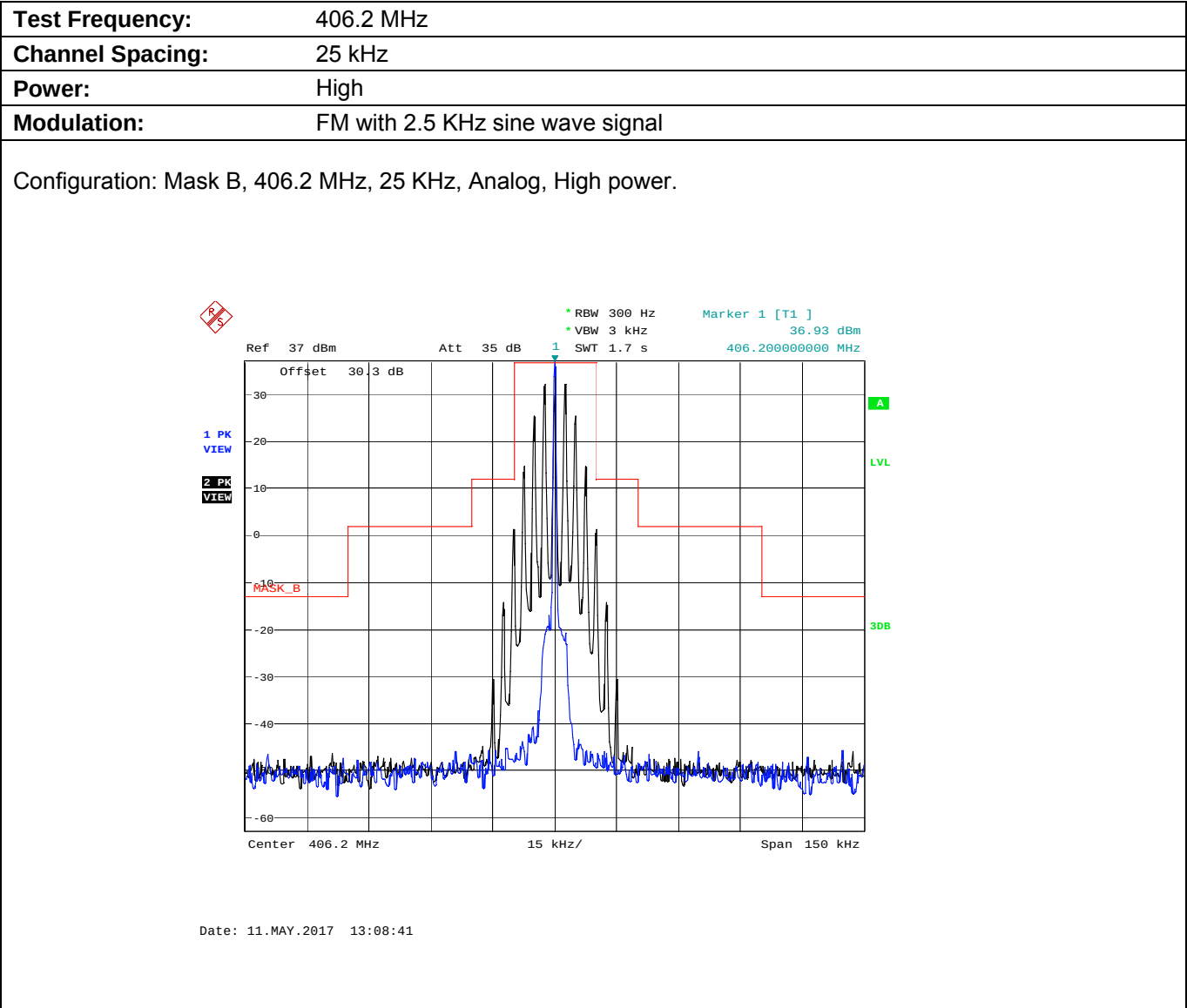
Plot 5.8.4.4.1. Emission Mask B, High Power
