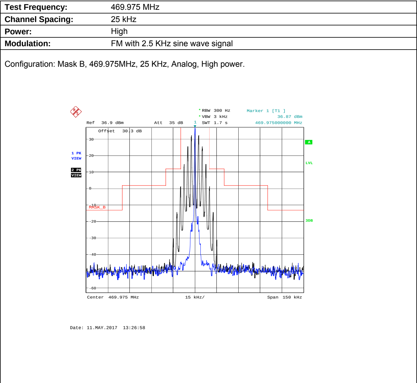
Plot 5.8.4.4.3. Emission Mask B, High Power
