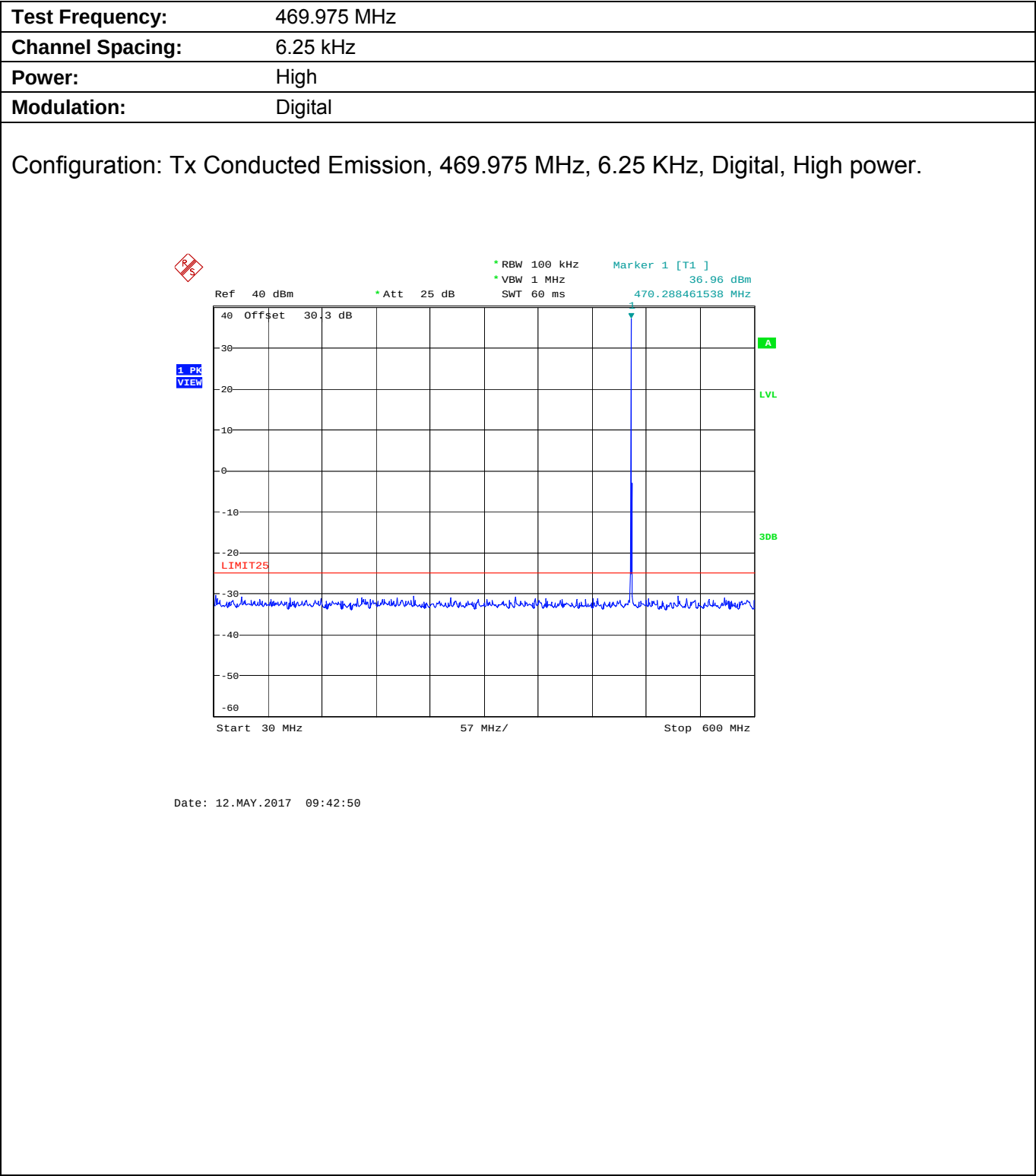
Plot 5.9.4.3.1. Conducted Transmitter Spurious Emissions for 469.975 MHz, High Power
