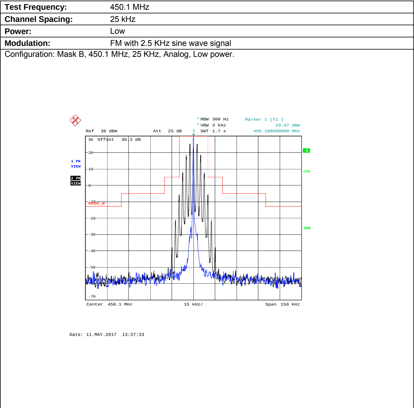
Plot 5.8.4.4.5. Emission Mask B, Low Power
