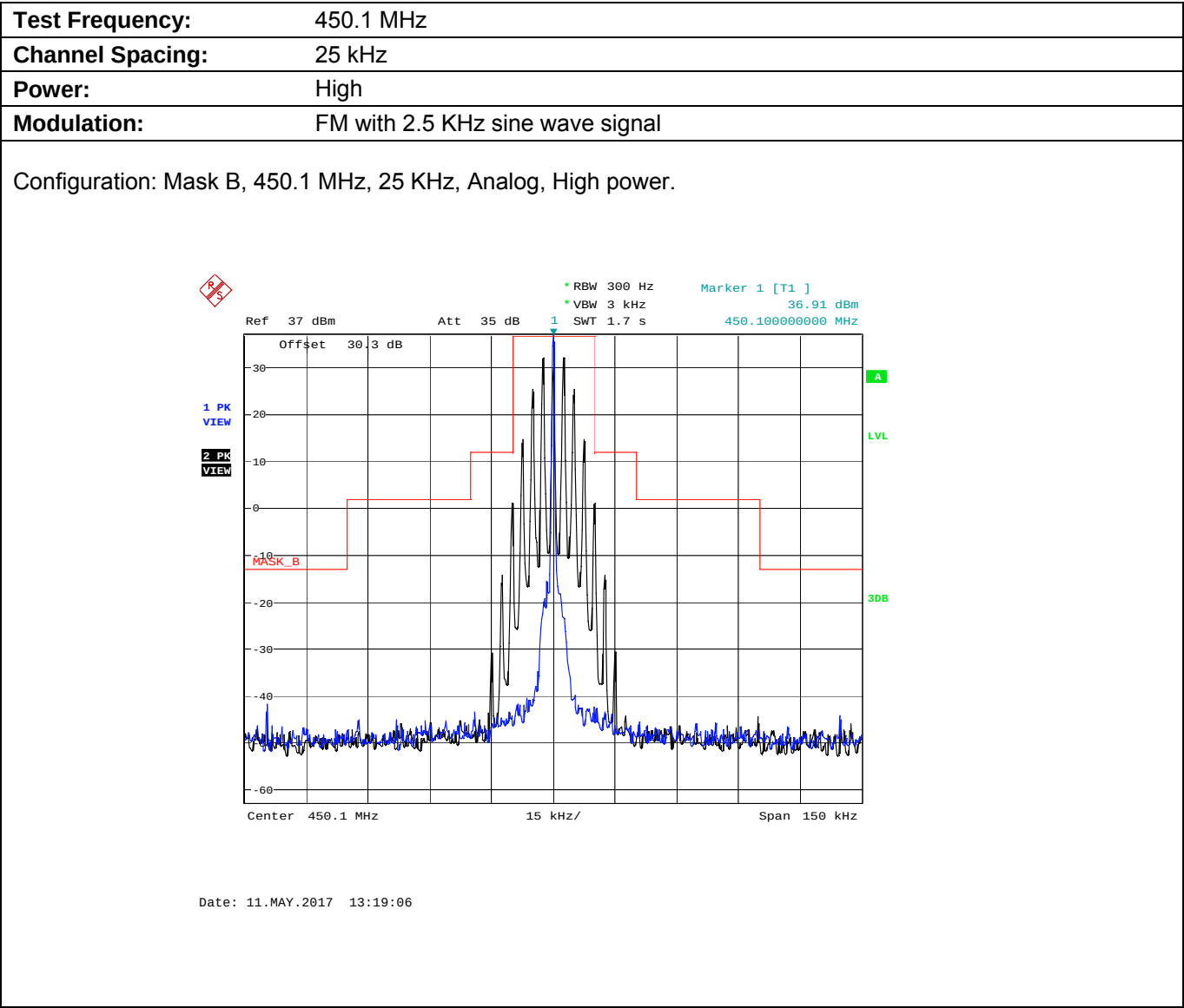
Plot 5.8.4.4.2. Emission Mask B, High Power
