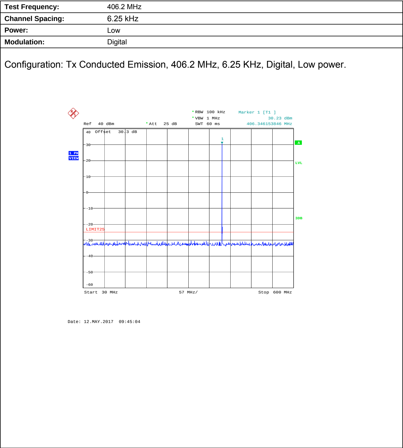
Plot 5.9.4.1.2. Conducted Transmitter Spurious Emissions for 406.2 MHz, Low Power
