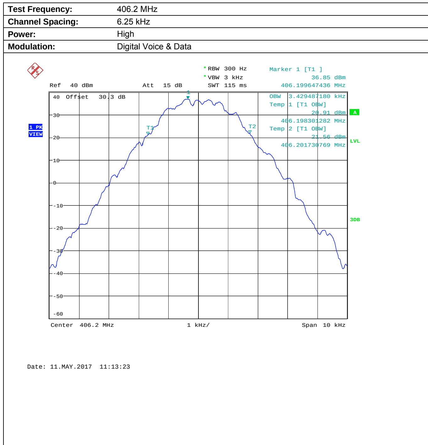
Plot 5.8.4.1.10. Occupied Bandwidth
