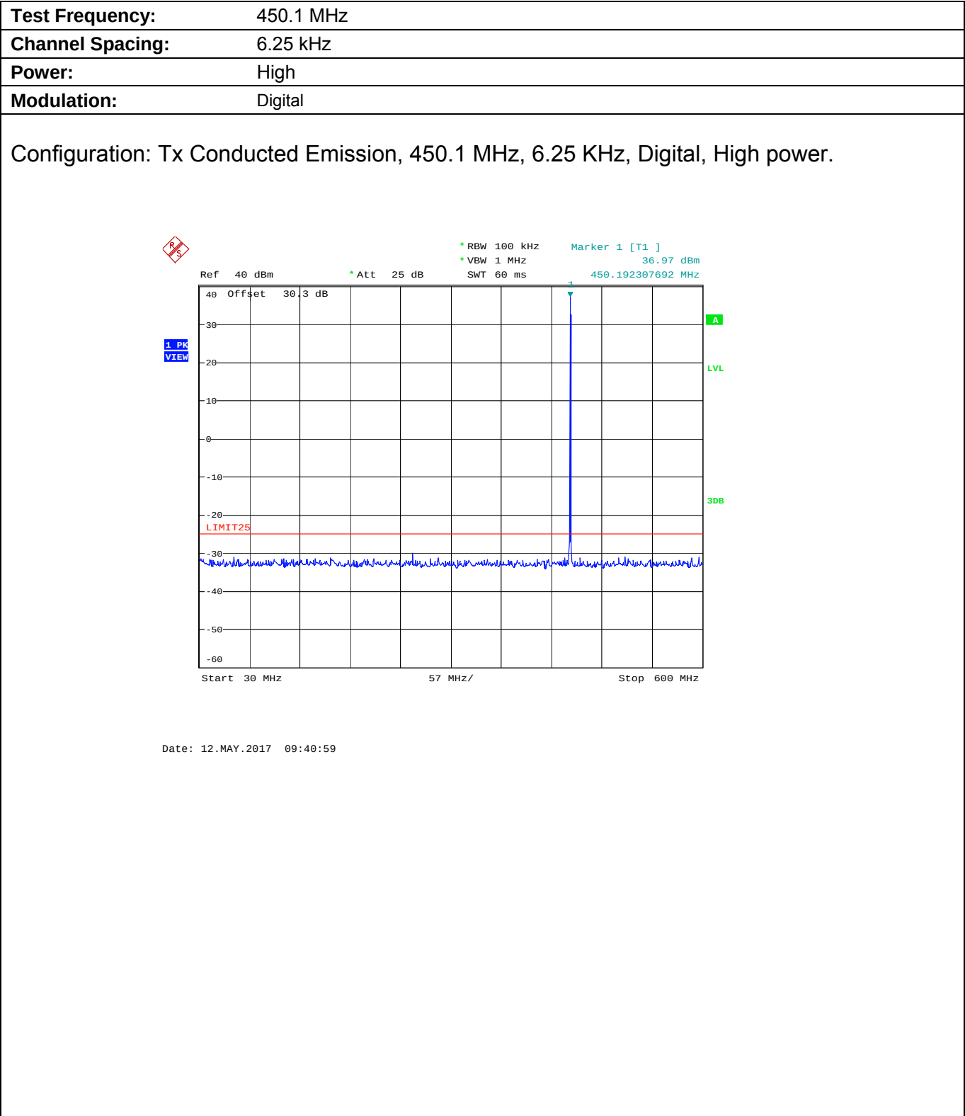
Plot 5.9.4.2.1. Conducted Transmitter Spurious Emissions for 450.1 MHz, High Power
