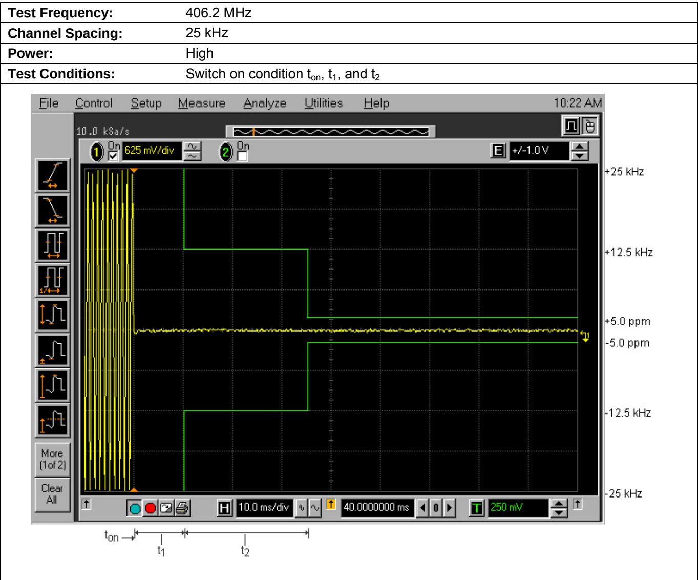
Plot 5.12.4.3. Transient Frequency Behavior for 25 kHz Channel Spacing
