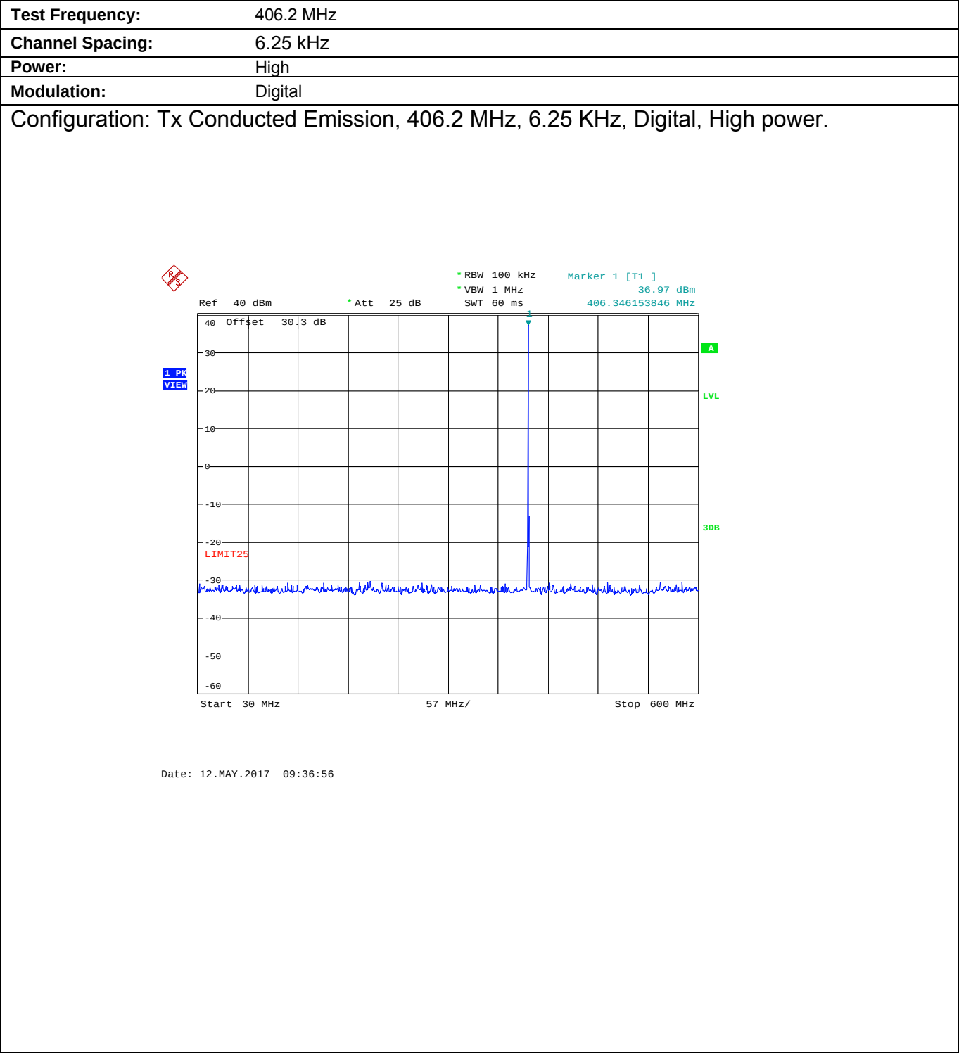
Plot 5.9.4.1.1. Conducted Transmitter Spurious Emissions for 406.2 MHz, High Power,
