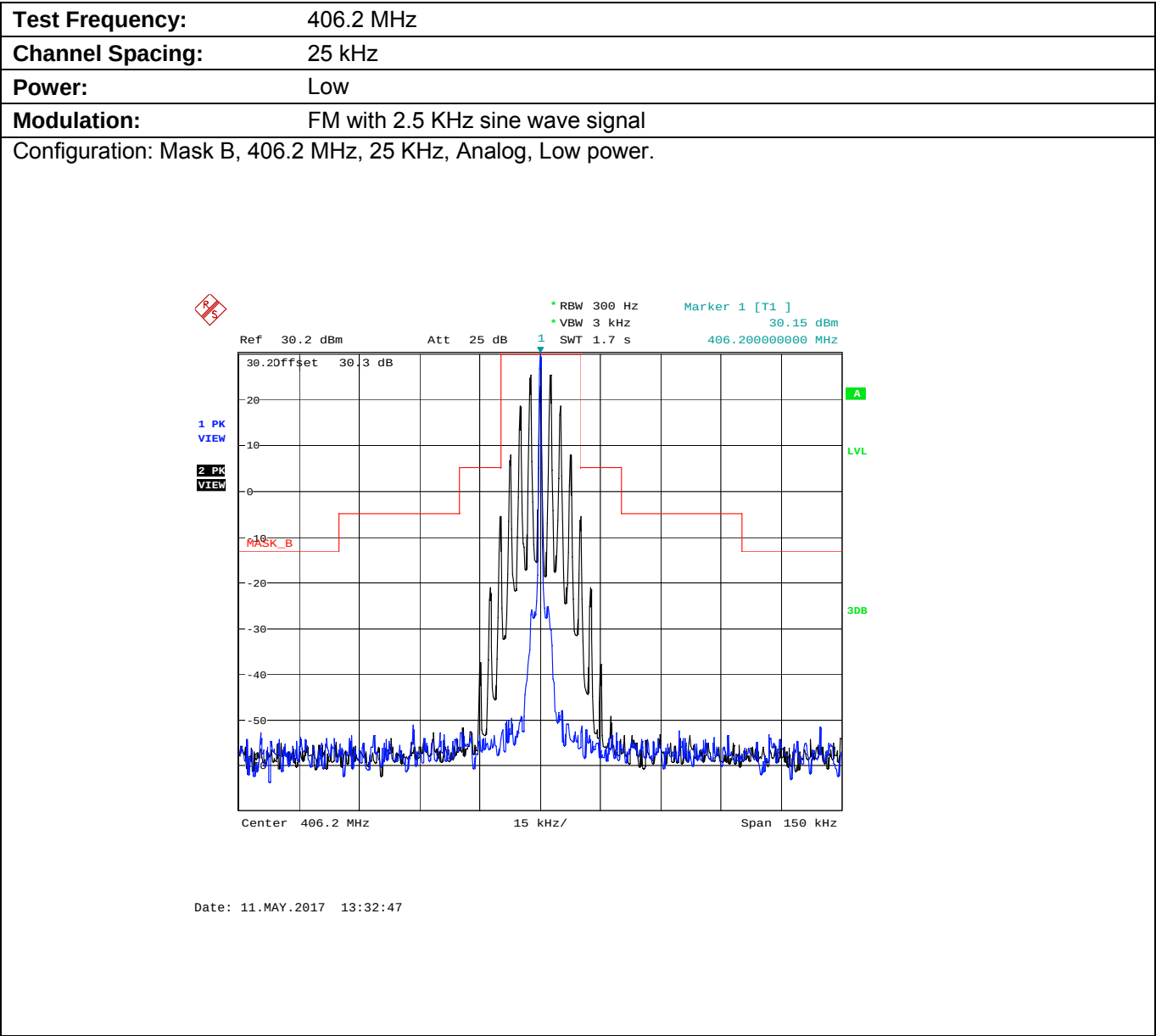
Plot 5.8.4.4.4. Emission Mask B, Low Power
