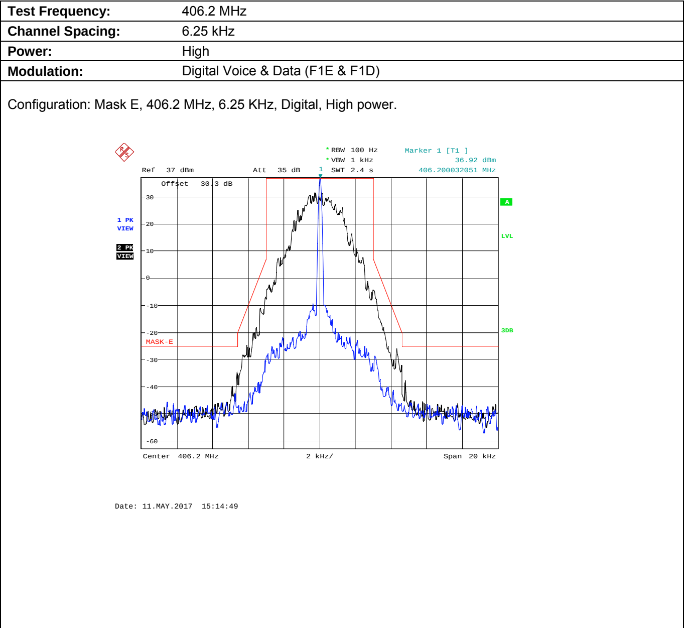
Plot 5.8.4.3.1. Emission Mask E, High Power
