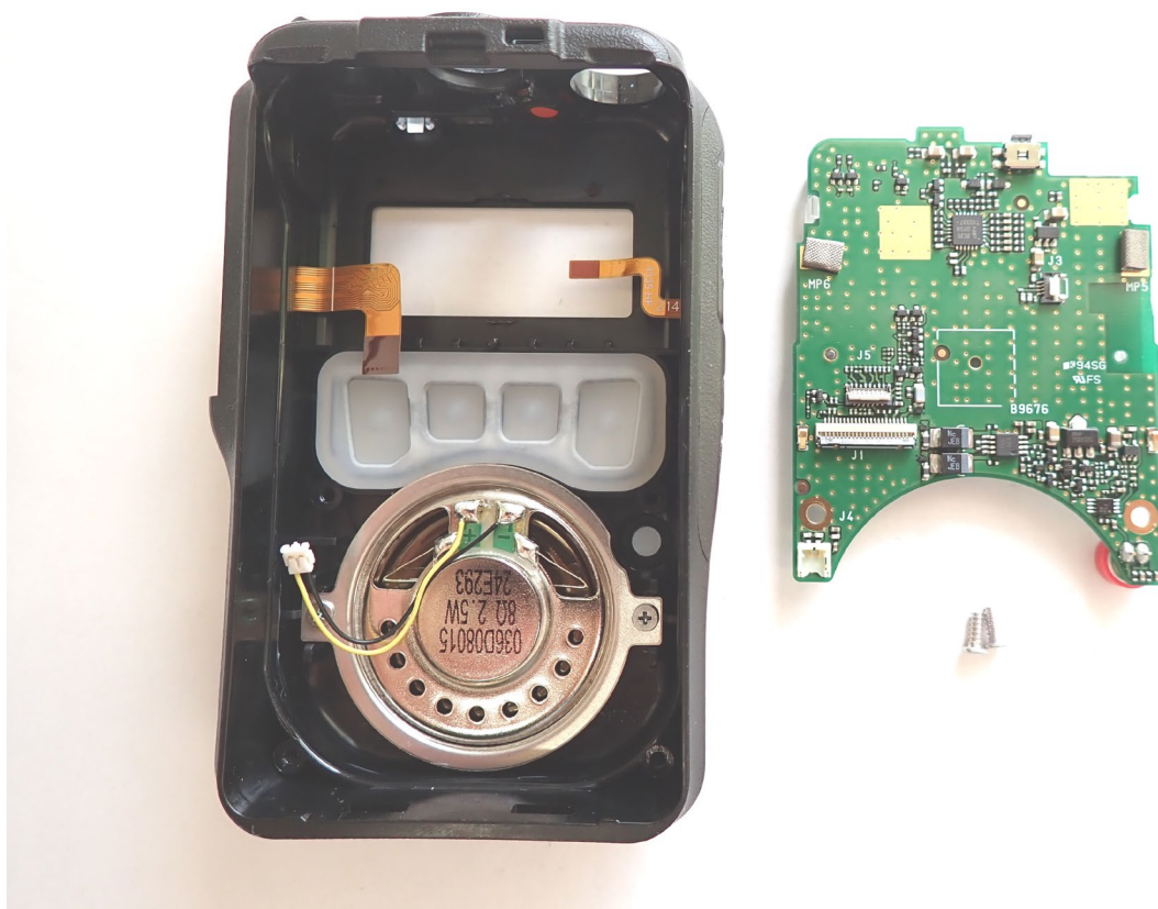
IC-F62D FRONT PANEL OPEN
