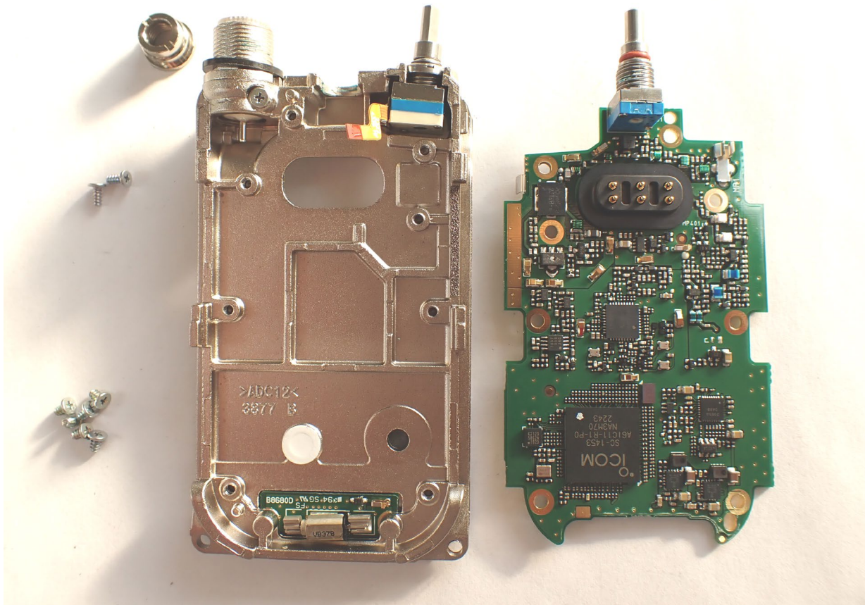
IC-F62D CHASSIS OPEN
