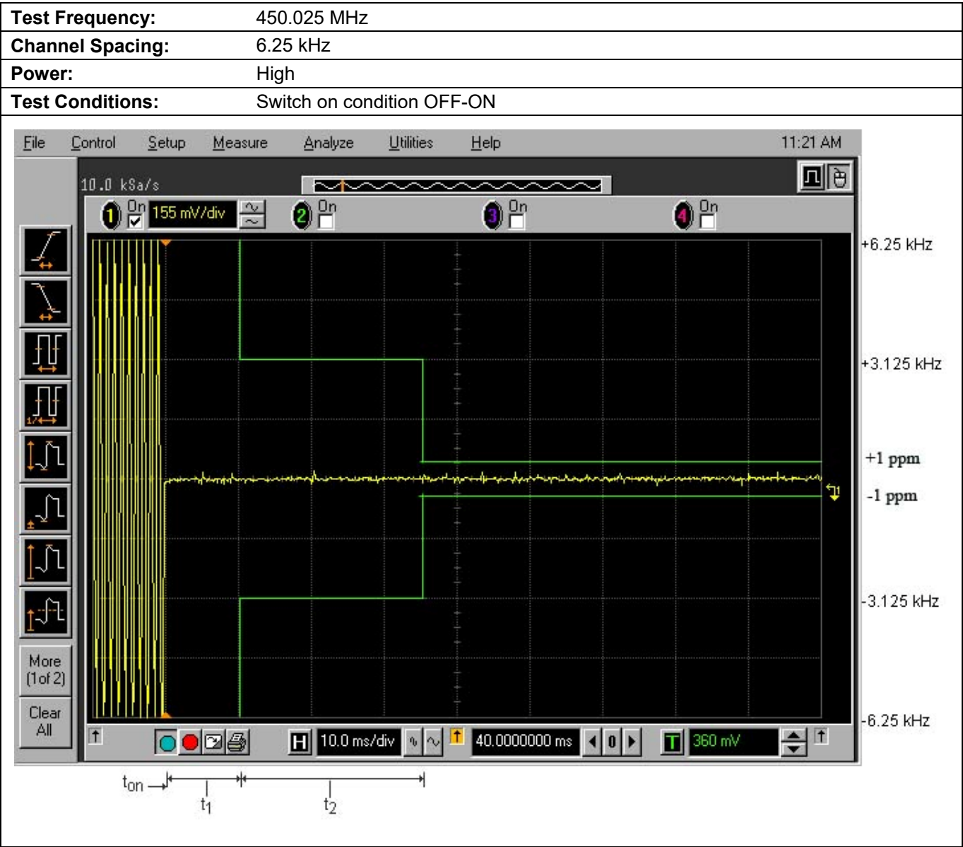
Plot 5.12.4.1. Transient Frequency Behavior for 6.25 kHz Channel Spacing
