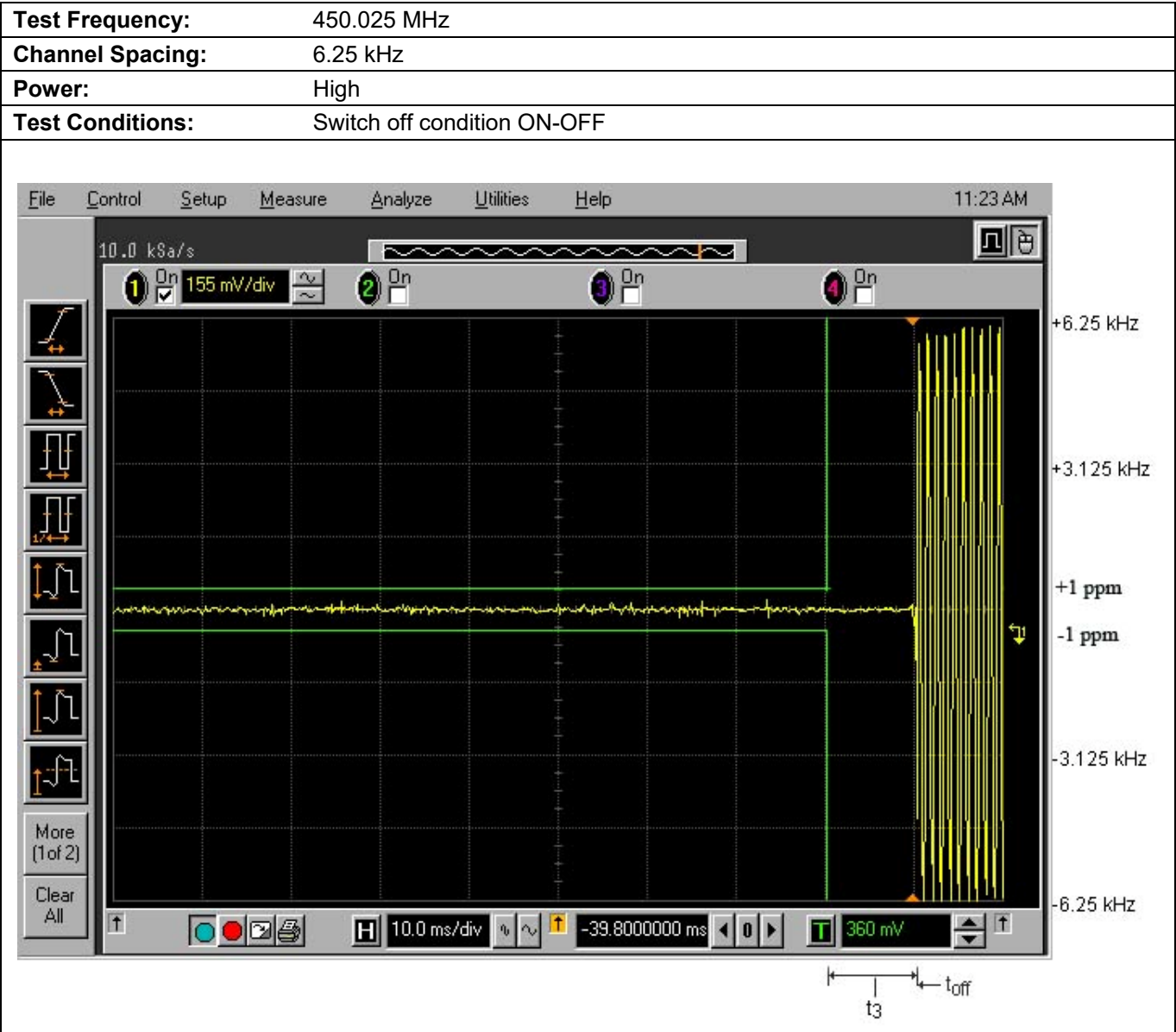
Plot 5.12.4.2. Transient Frequency Behavior for 6.25 kHz Channel Spacing
