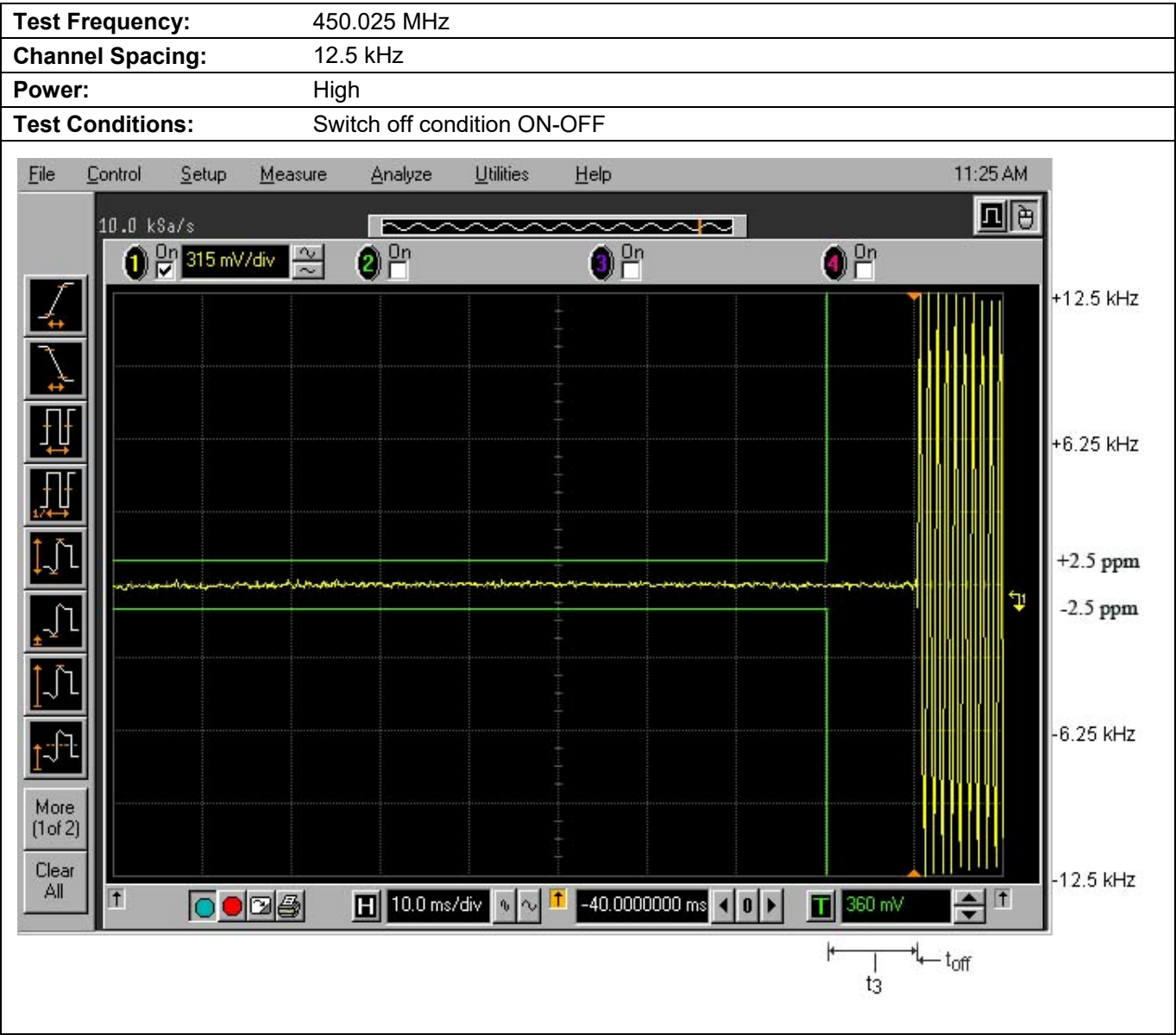
Plot 5.12.4.4. Transient Frequency Behavior for 12.5 kHz Channel Spacing
