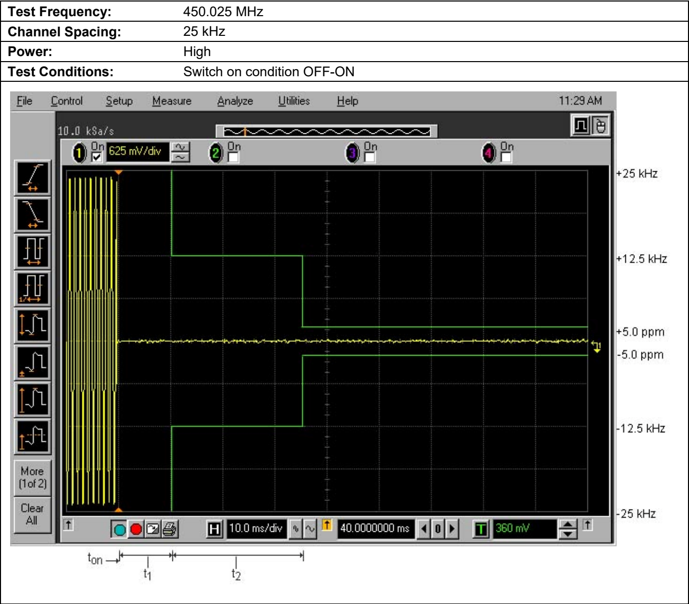
Plot 5.12.4.5. Transient Frequency Behavior for 25 kHz Channel Spacing
