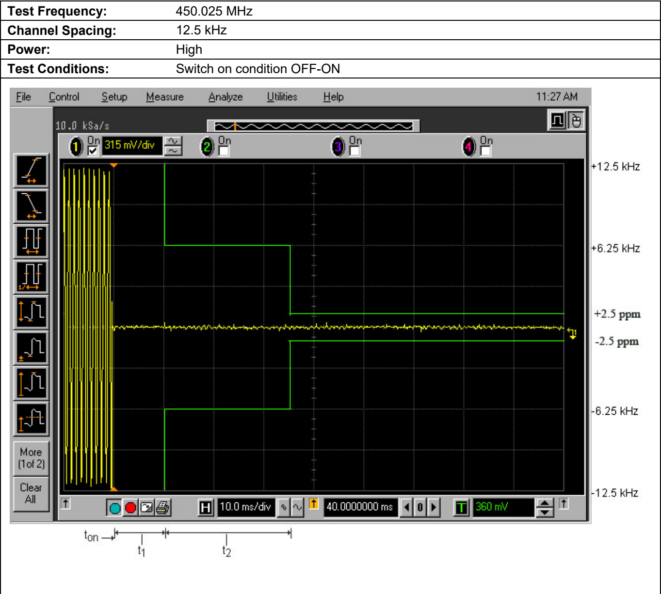
Plot 5.12.4.3. Transient Frequency Behavior for 12.5 kHz Channel Spacing
