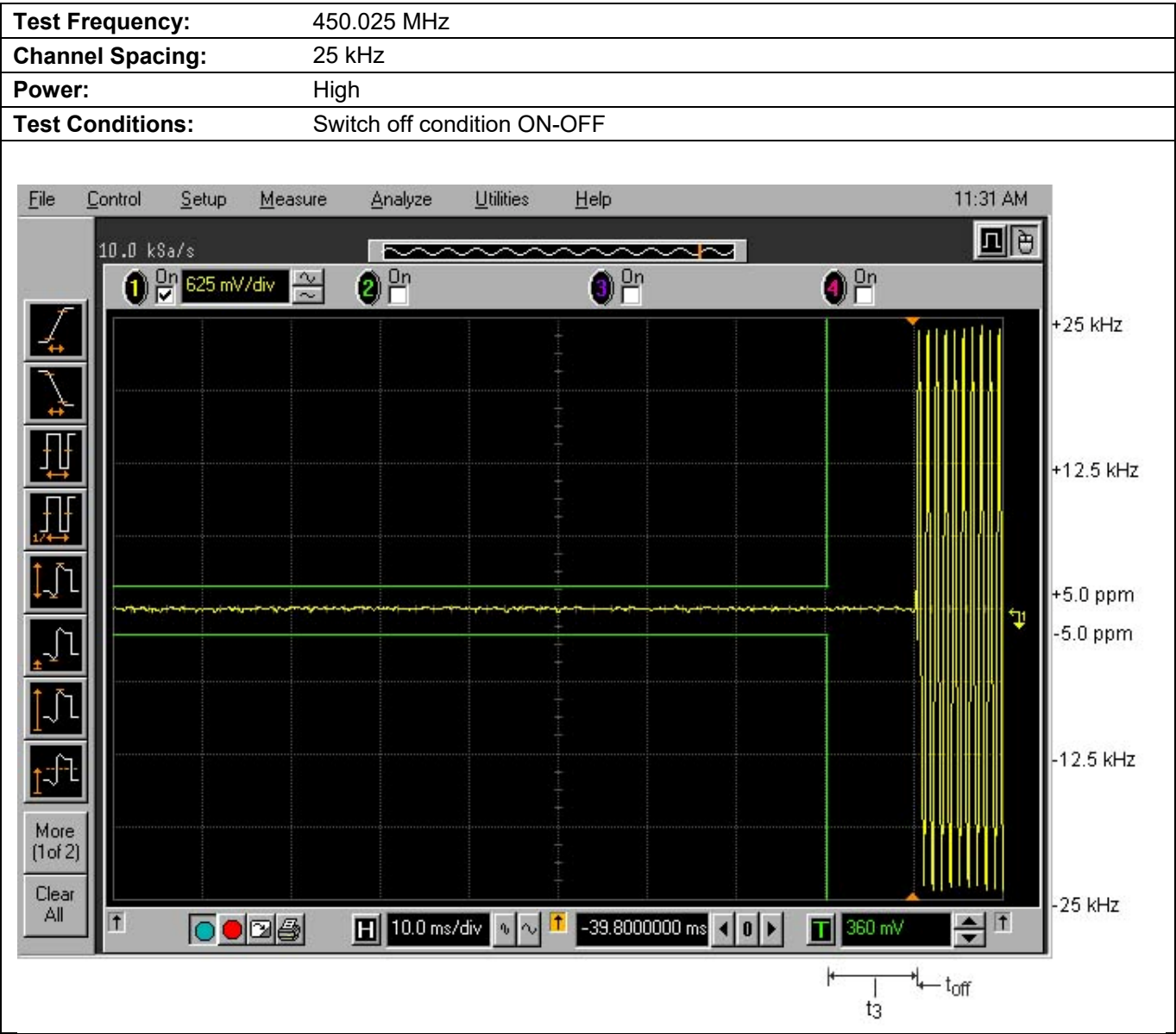
Plot 5.12.4.6. Transient Frequency Behavior for 25 kHz Channel Spacing
