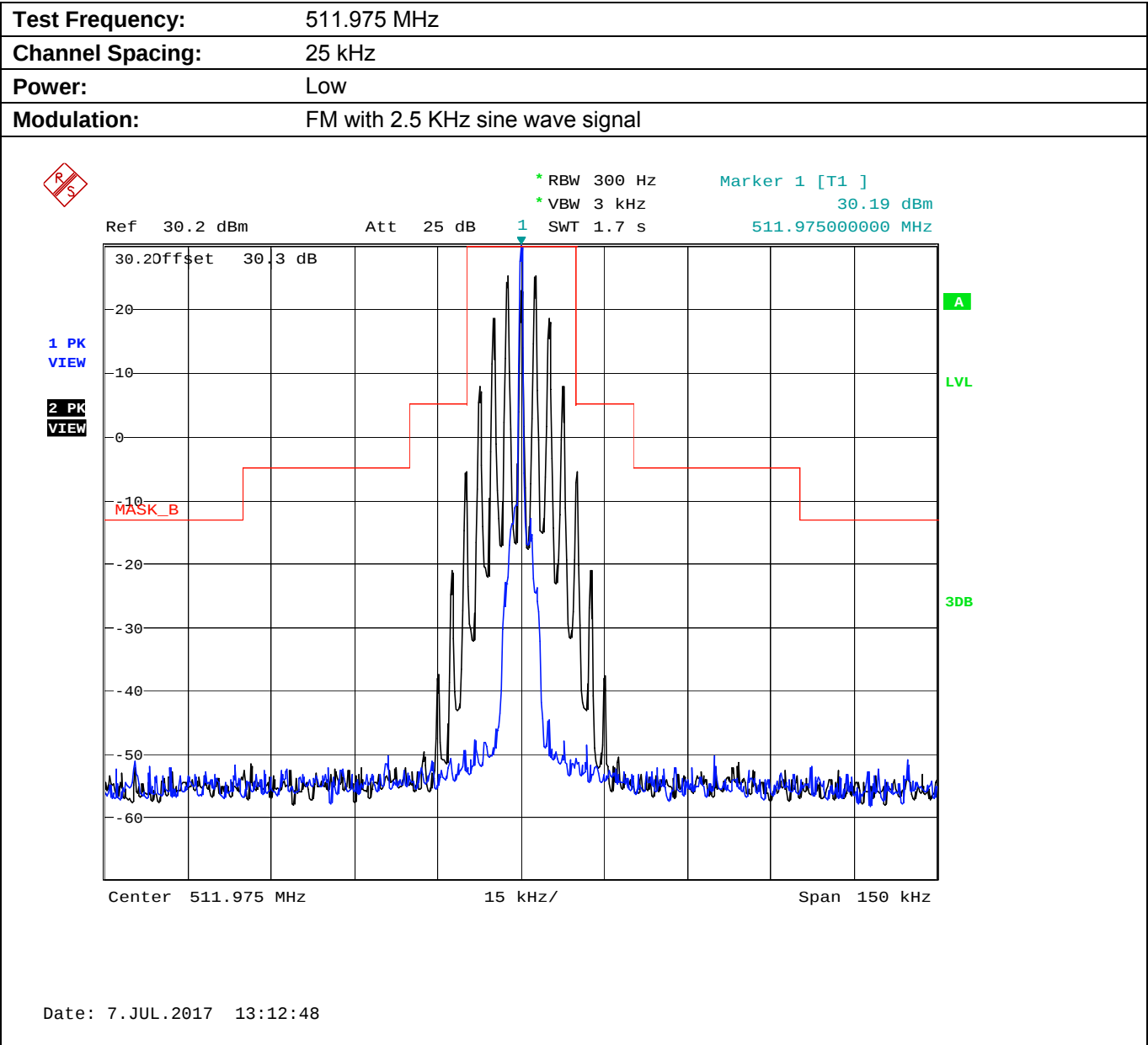
Plot 5.8.4.4.6. Emission Mask B, Low Power
