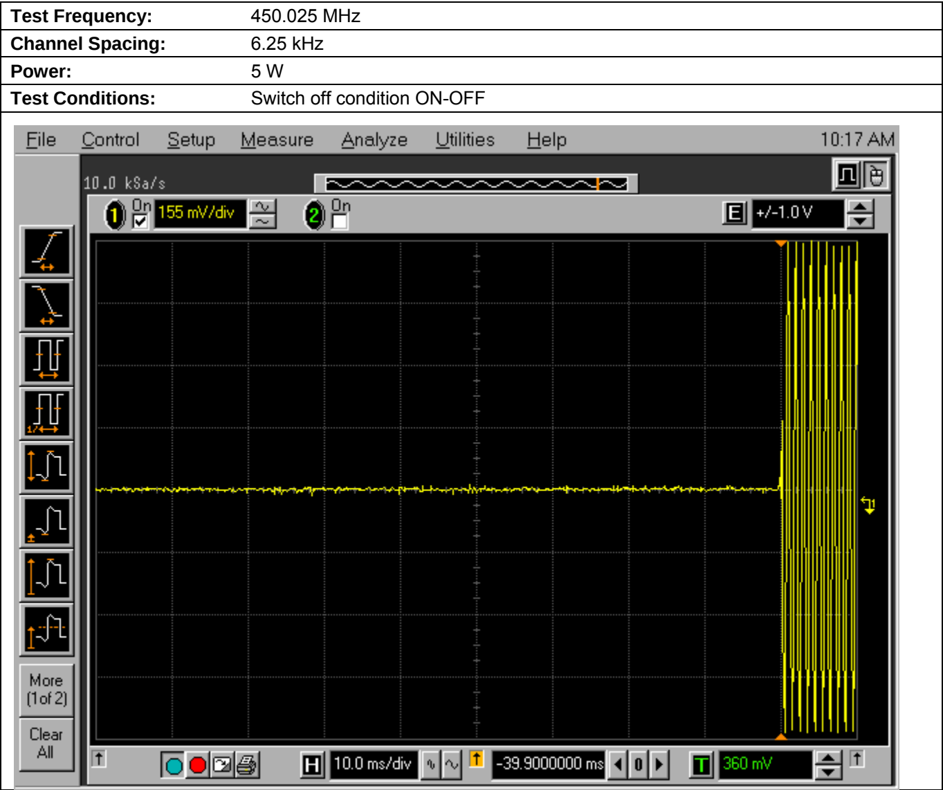
Plot 5.12.4.6. Transient Frequency Behavior for 6.25 kHz Channel Spacing
