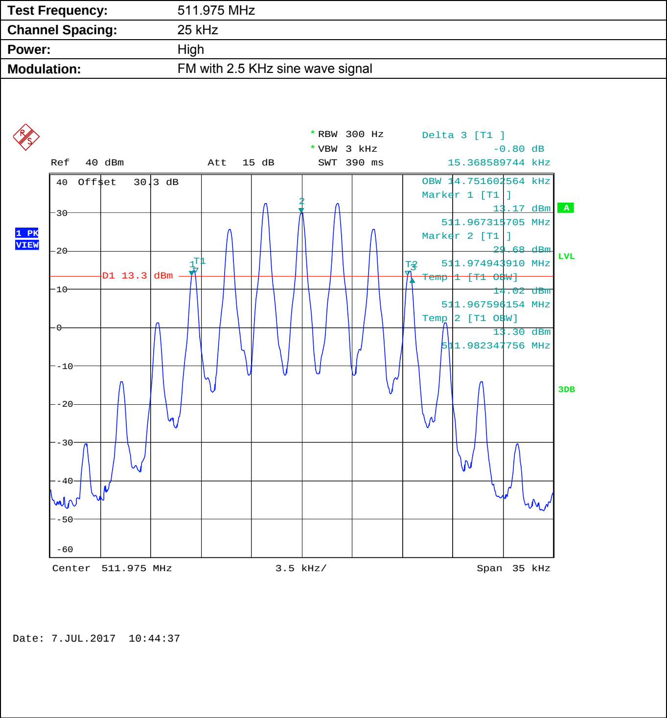
Plot 5.8.4.1.3. Occupied Bandwidth
