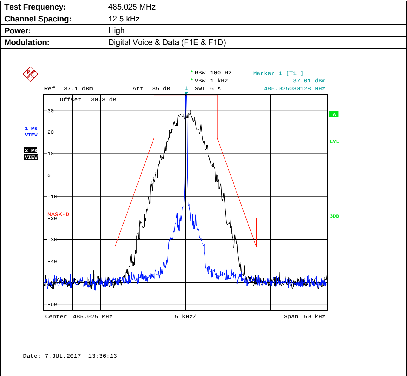
Plot 5.8.4.2.8. Emission Mask D, High Power
