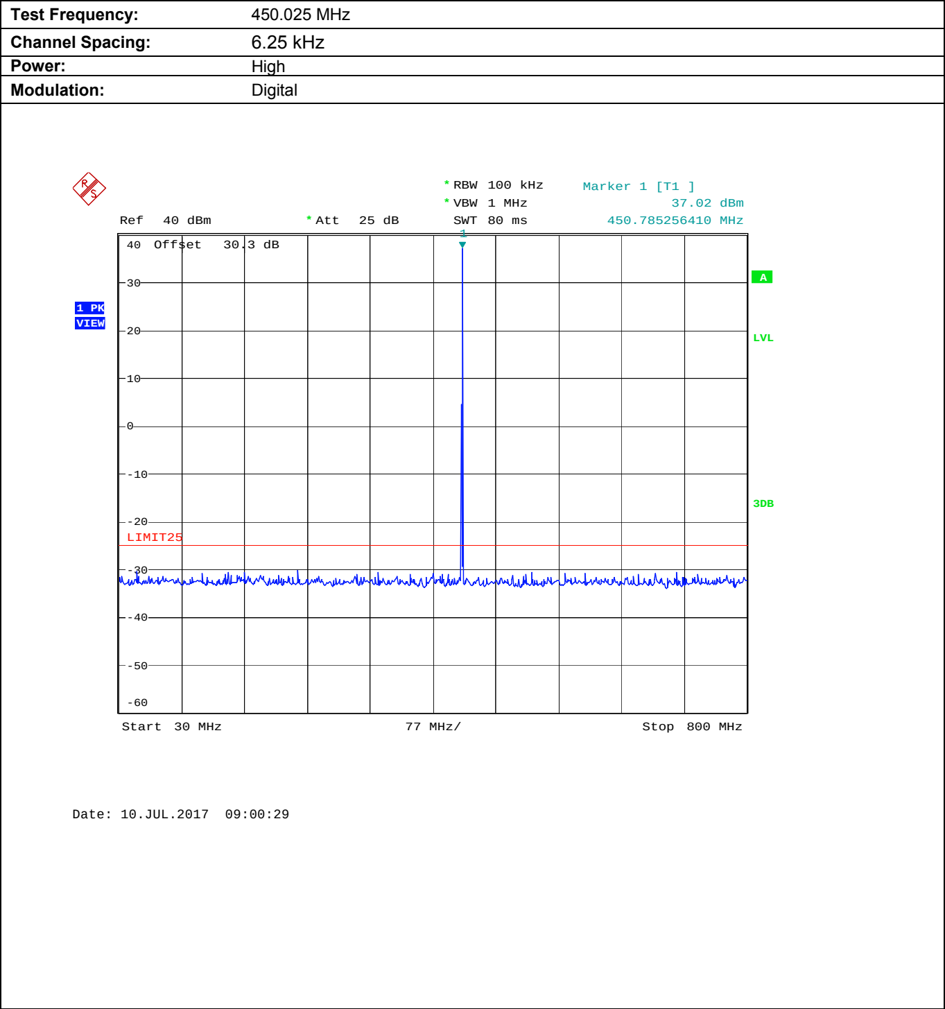
Plot 5.9.4.1.1. Conducted Transmitter Spurious Emissions for 450.025 MHz, High Power,
