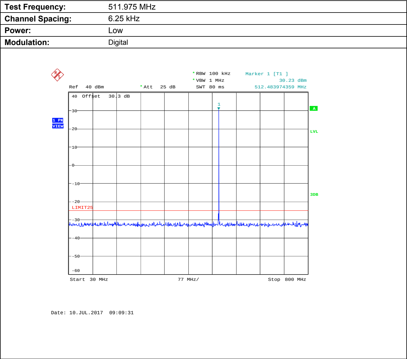
Plot 5.9.4.3.2. Conducted Transmitter Spurious Emissions for 511.975 MHz, Low Power
