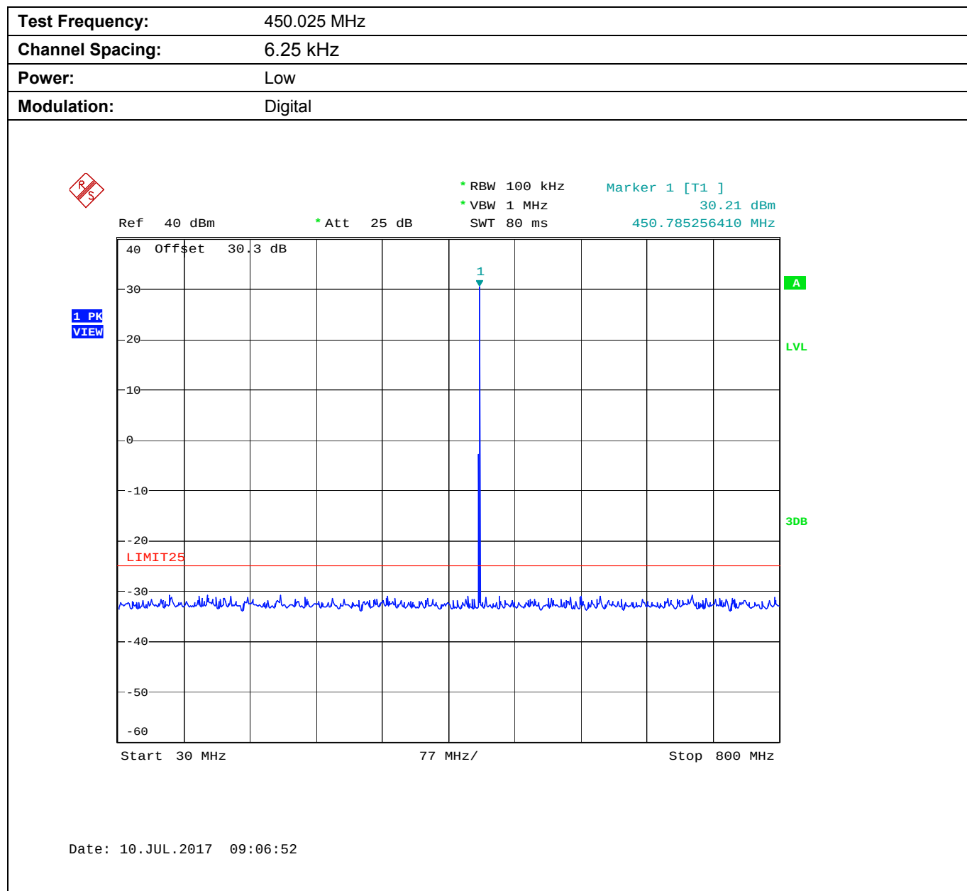
Plot 5.9.4.1.2. Conducted Transmitter Spurious Emissions for 450.025 MHz, Low Power
