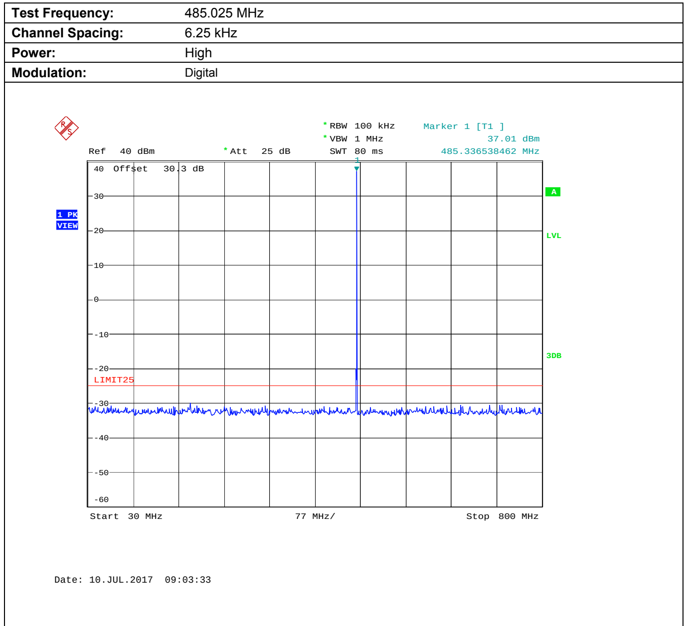
Plot 5.9.4.2.1. Conducted Transmitter Spurious Emissions for 485.025 MHz, High Power
