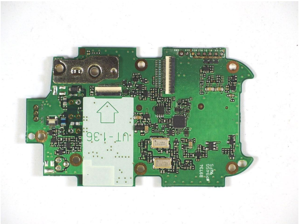
MAIN SIDE A (WITHOUT UT-136)
