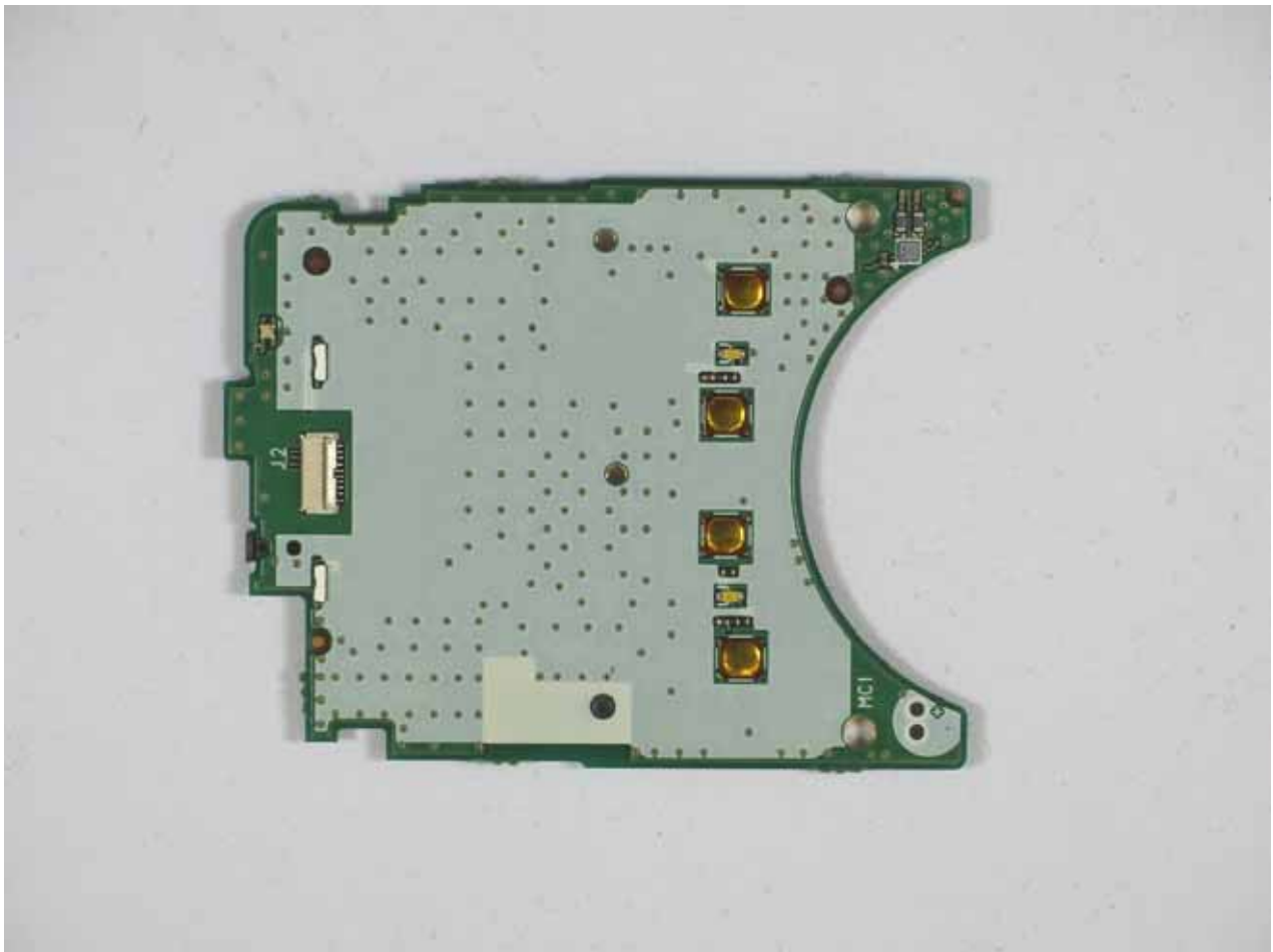
FRONT SIDE A WITHOUT LCD
