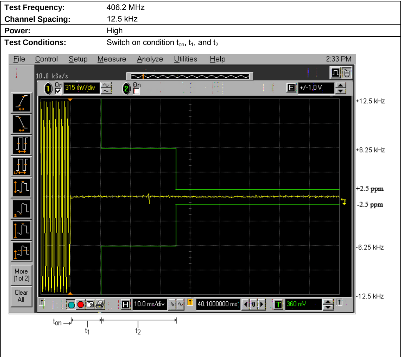
Plot 5.12.4.1. Transient Frequency Behavior for 12.5 kHz Channel Spacing
