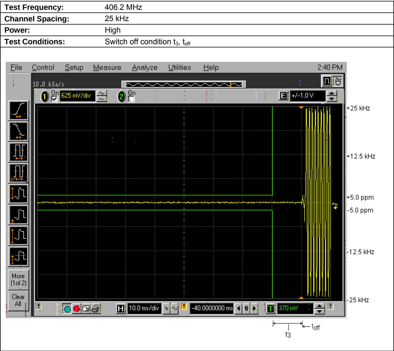
Plot 5.12.4.4. Transient Frequency Behavior for 25 kHz Channel Spacing
