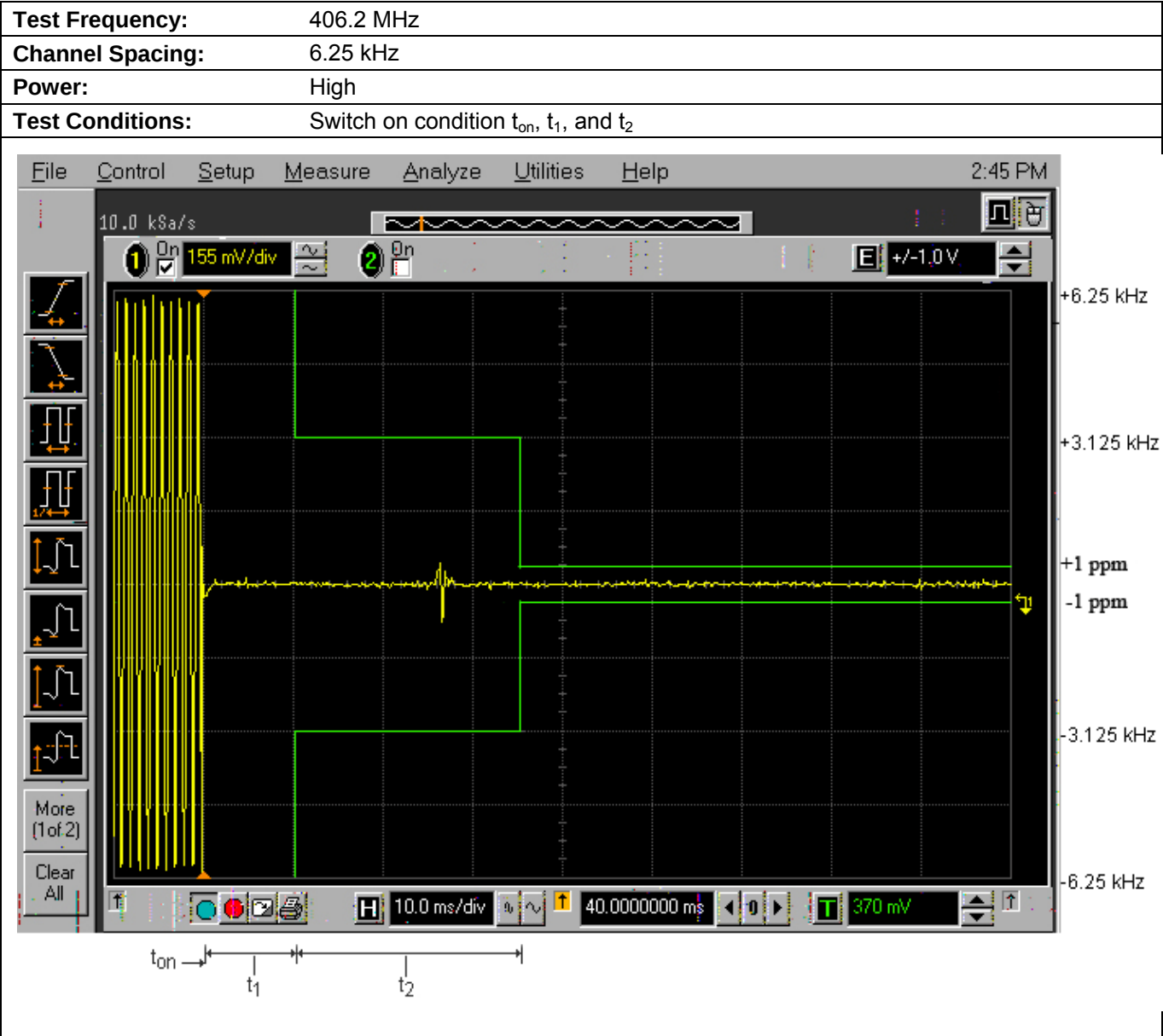
Plot 5.12.4.5. Transient Frequency Behavior for 6.25 kHz Channel Spacing
