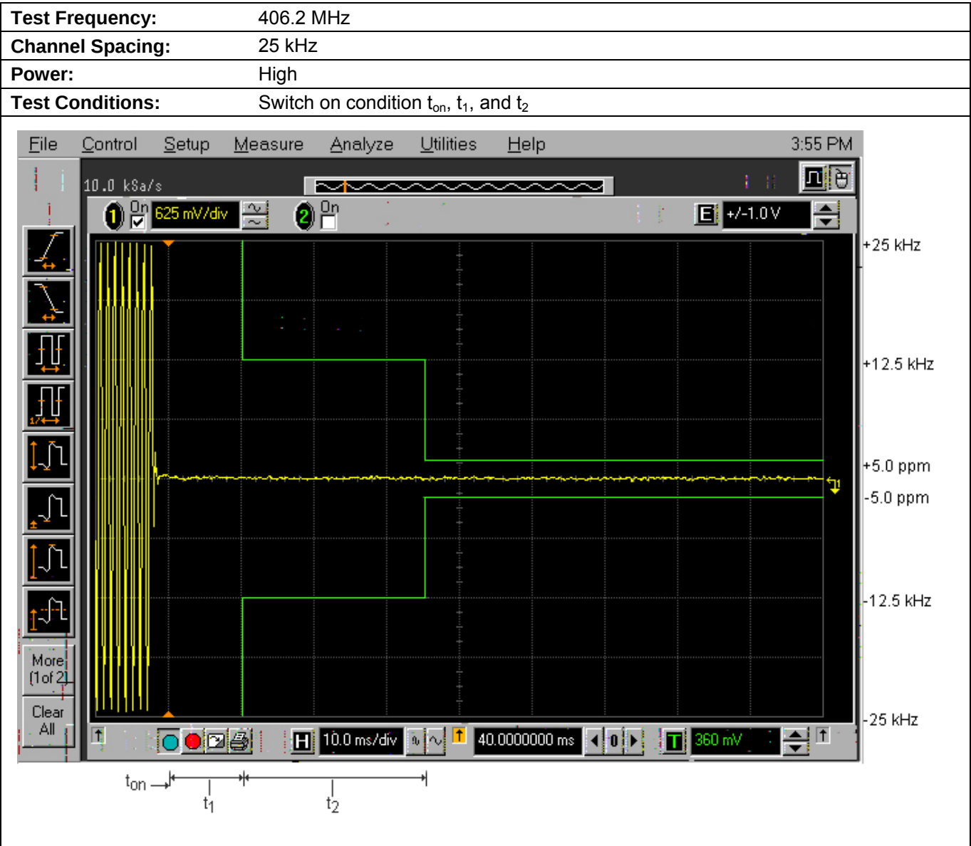
Plot 5.12.3.3. Transient Frequency Behavior for 25 kHz Channel Spacing
