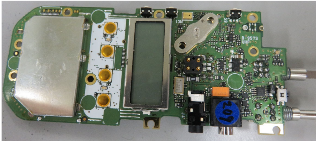
MAIN Board side-A view(IC-F2100DS)
