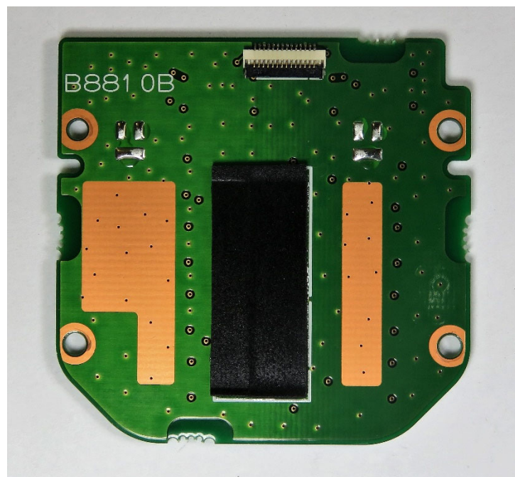
Front Board side-B view(IC-F2100DT)
