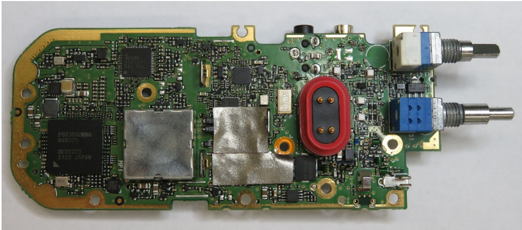
MAIN Board side-B view(IC-F2100DS)
