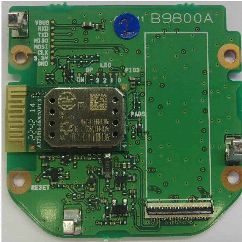
FRONT-1_B_built-in Bluetooth Ver.
