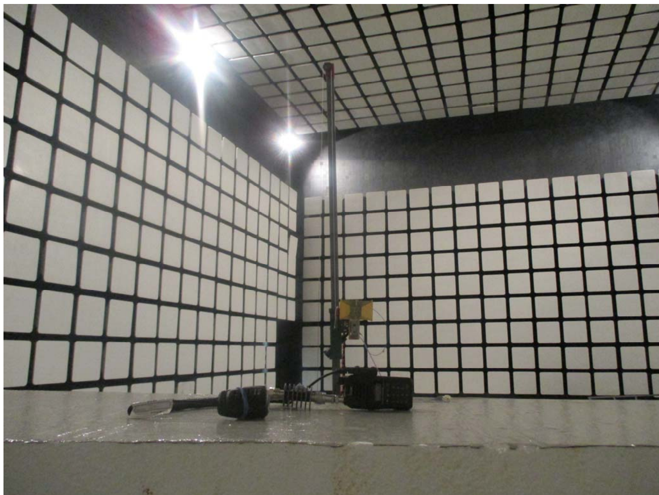
Radiated Emissions at 3 m, Above 1 GHz Orthogonal Position 3
