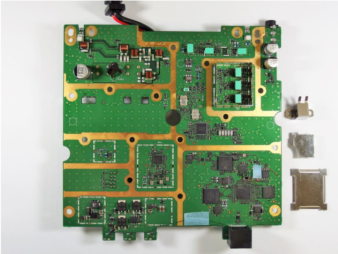
UR-FR5300 MAIN BOARD SIDE-B
