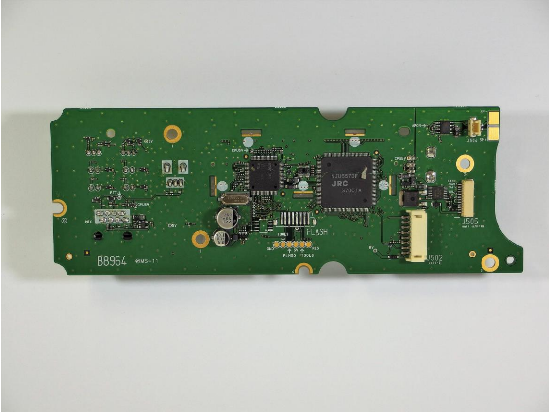
IC-FR5300 FRONT BOARD SIDE-B
