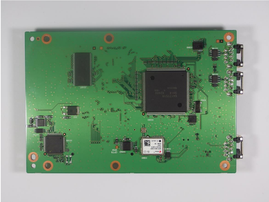
UC-FR5300 MAIN BOARD SIDE-B
