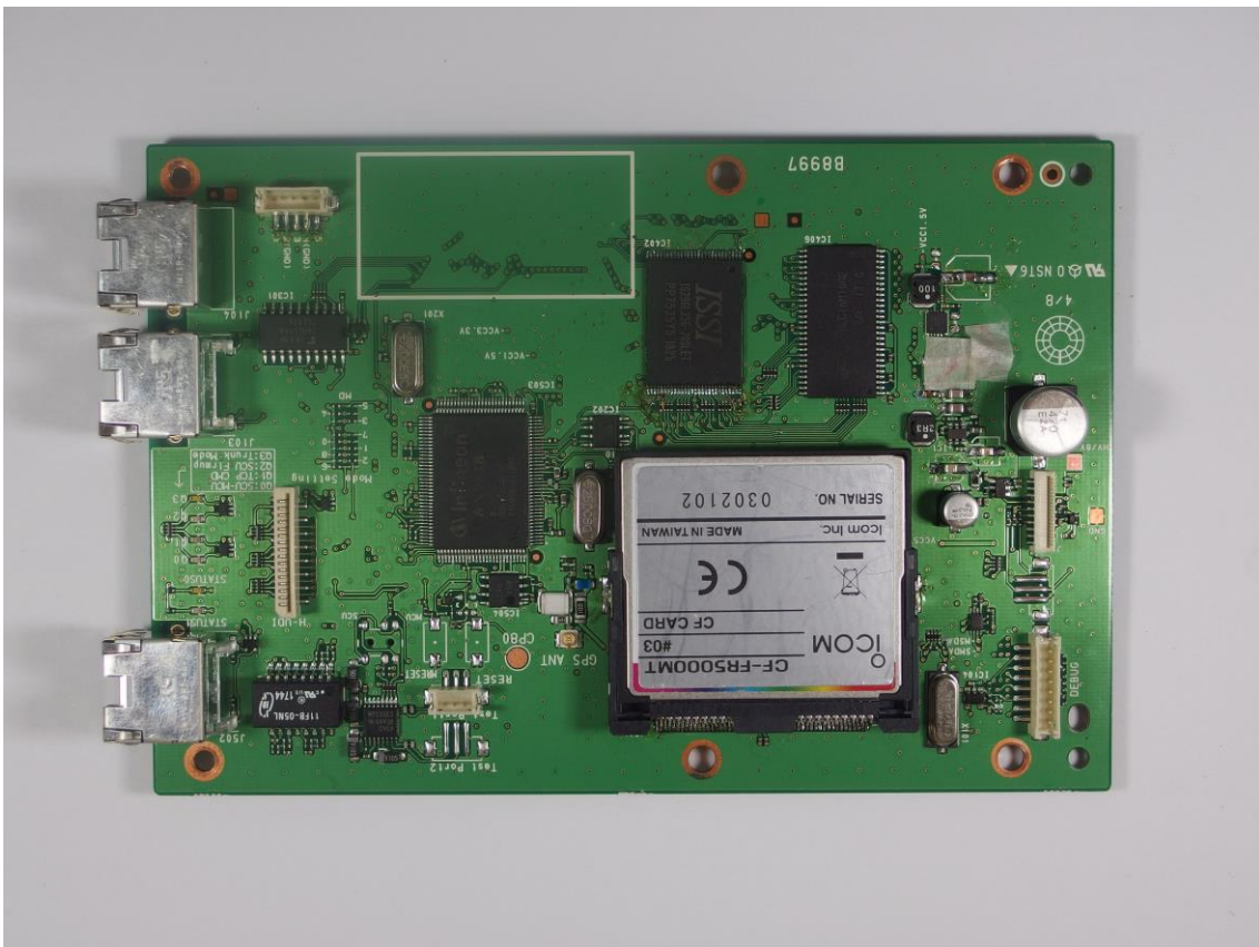
UC-FR5300 MAIN BOARD SIDE-A
