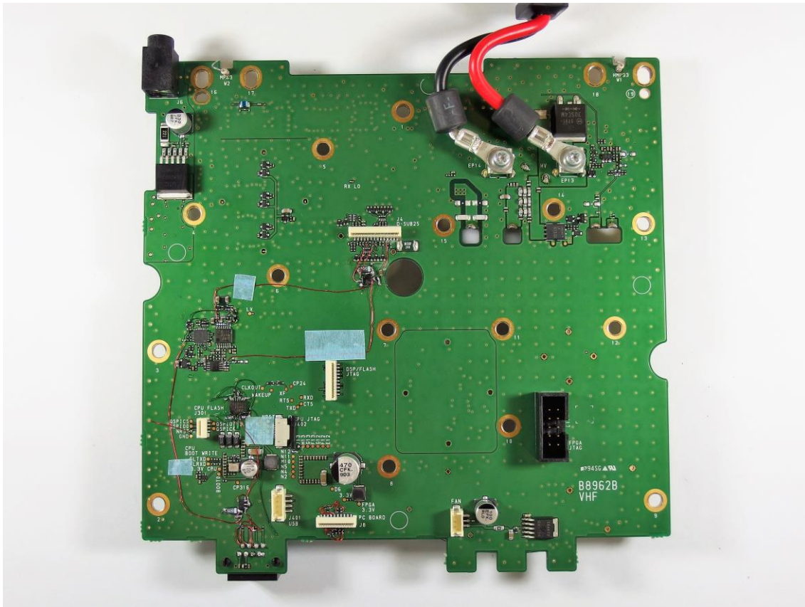
UR-FR5300 MAIN BOARD SIDE-A
