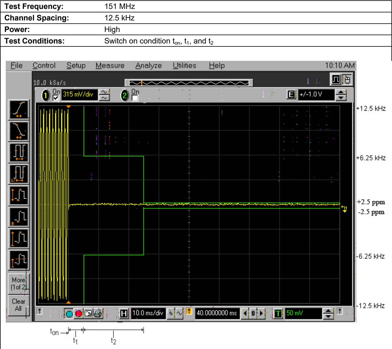
Plot 5.12.3.1. Transient Frequency Behavior for 12.5 kHz Channel Spacing
