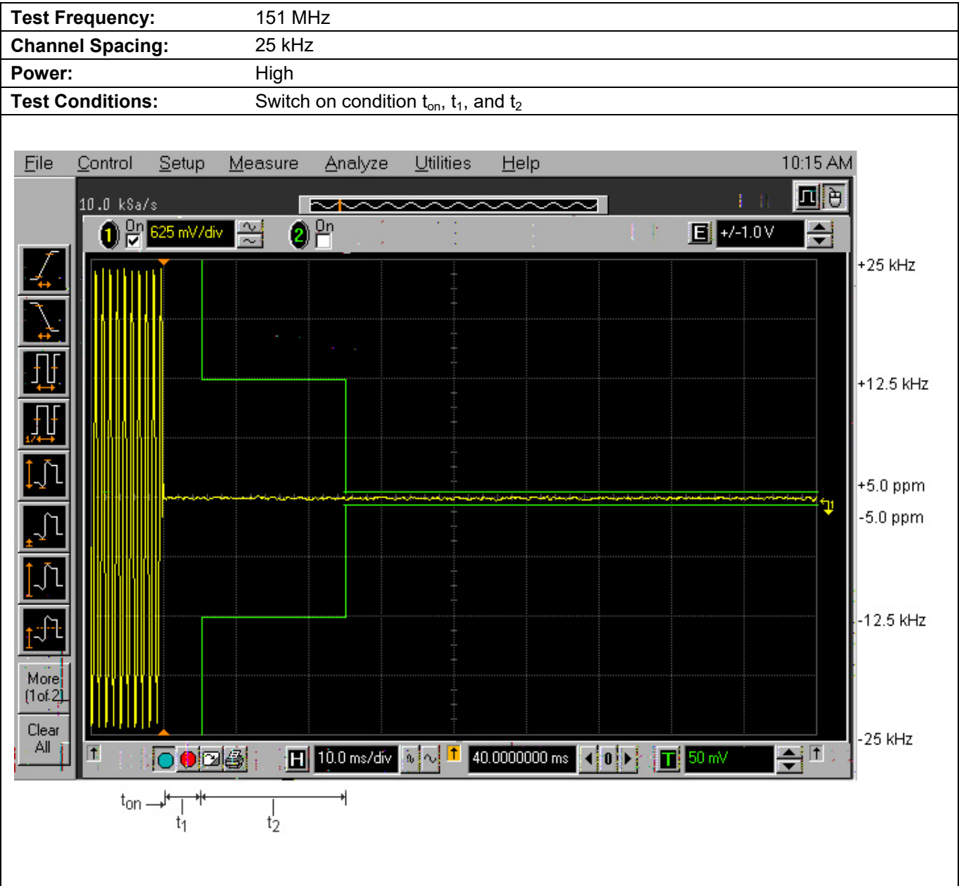
Plot 5.12.3.3. Transient Frequency Behavior for 25 kHz Channel Spacing
