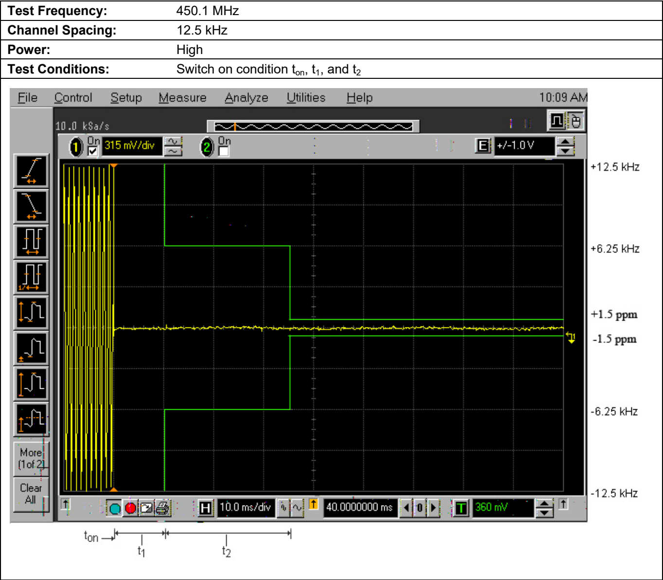
Plot 5.12.3.1. Transient Frequency Behavior for 12.5 kHz Channel Spacing
