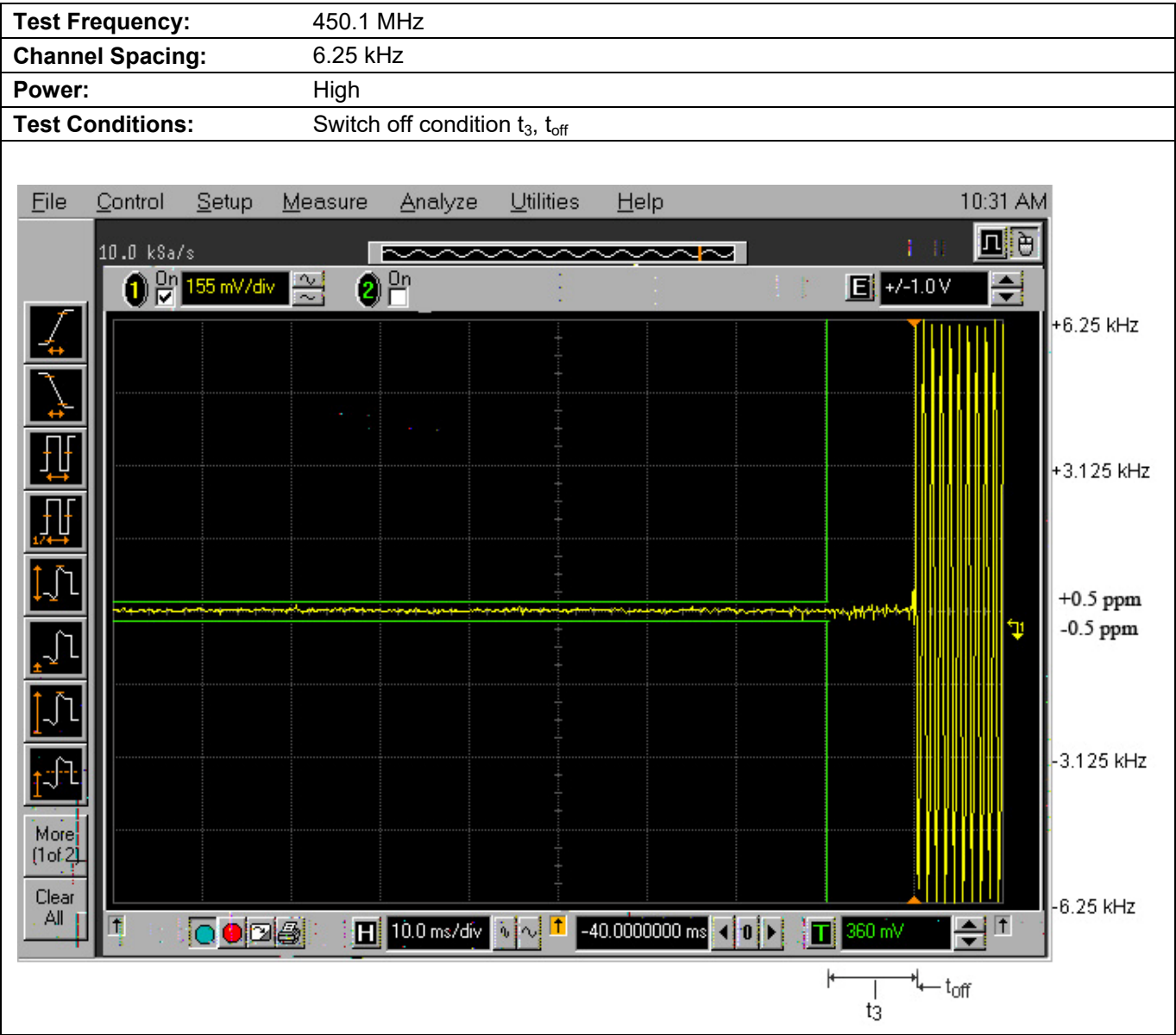
Plot 5.12.3.6. Transient Frequency Behavior for 6.25 kHz Channel Spacing
