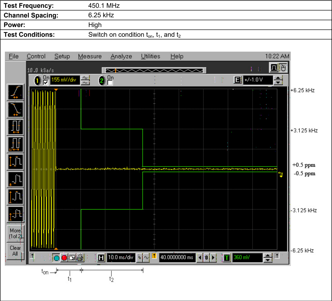
Plot 5.12.3.5. Transient Frequency Behavior for 6.25 kHz Channel Spacing
