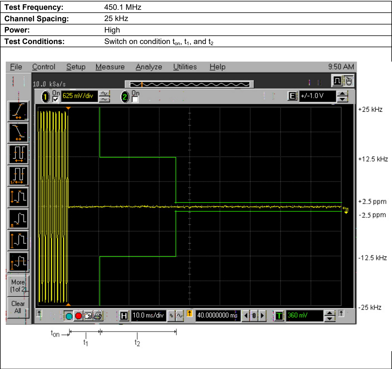
Plot 5.12.3.3. Transient Frequency Behavior for 25 kHz Channel Spacing
