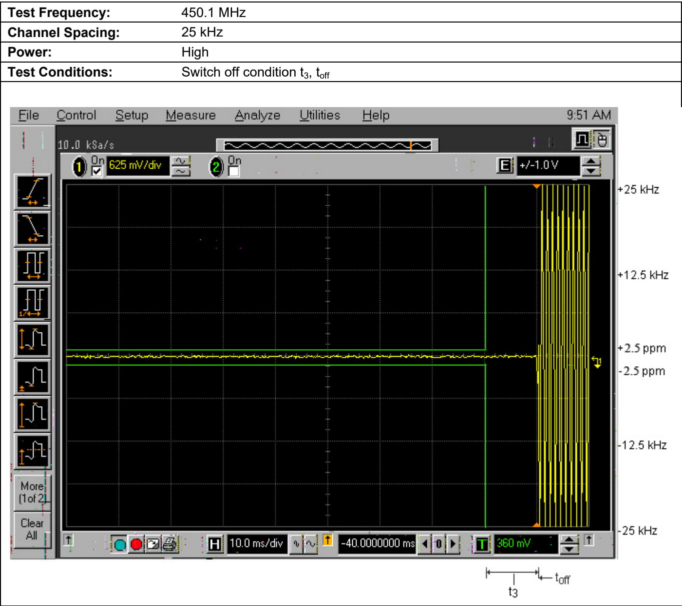
Plot 5.12.3.4. Transient Frequency Behavior for 25 kHz Channel Spacing
