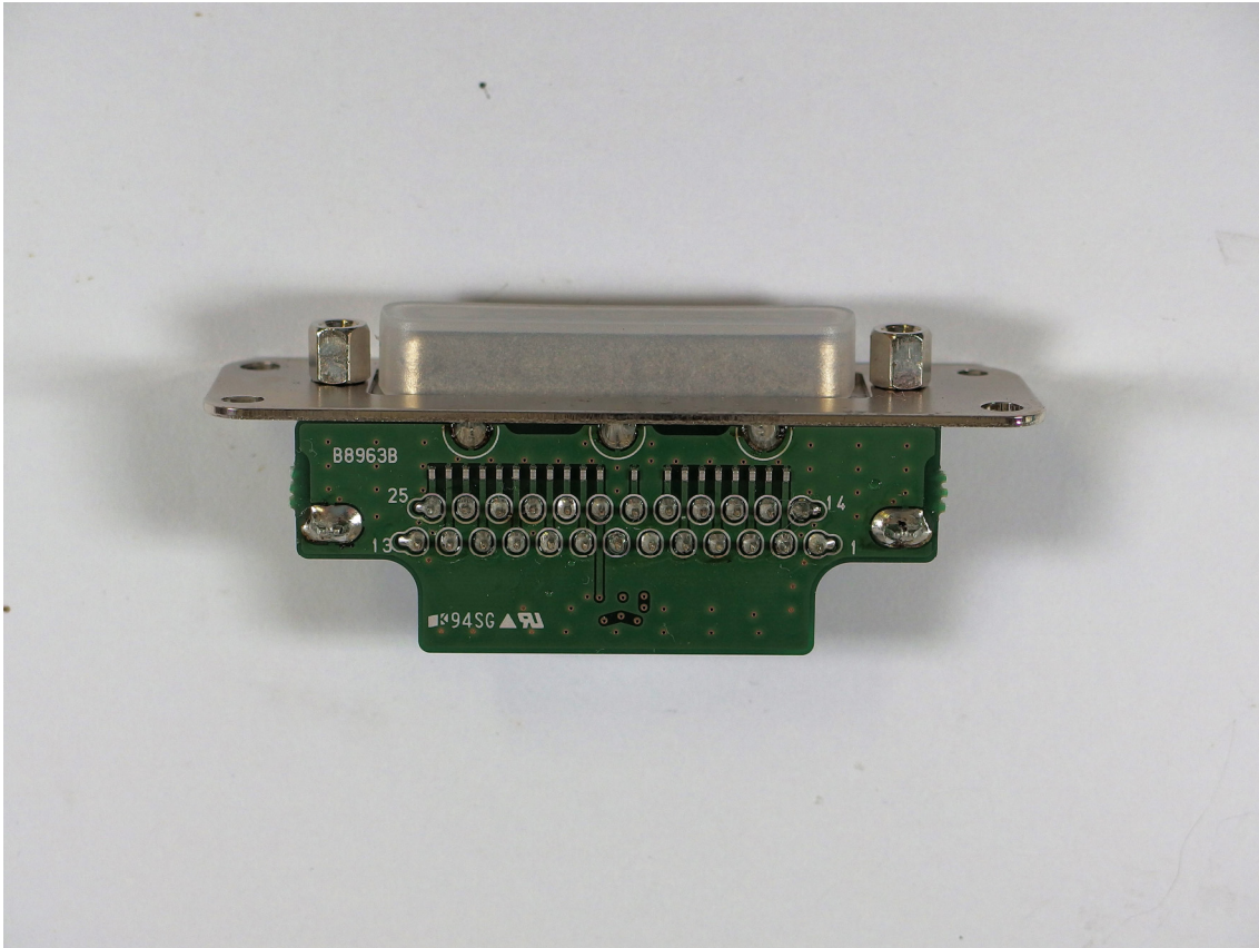
MAIN UNIT CONNECT BOARD SIDE-B
