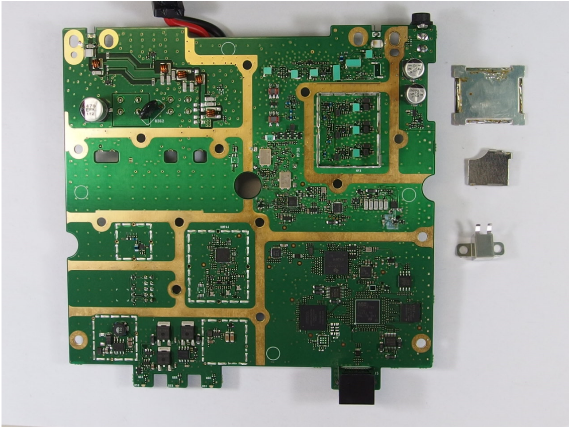
MAIN UNIT MAIN BOARD SIDE-B
