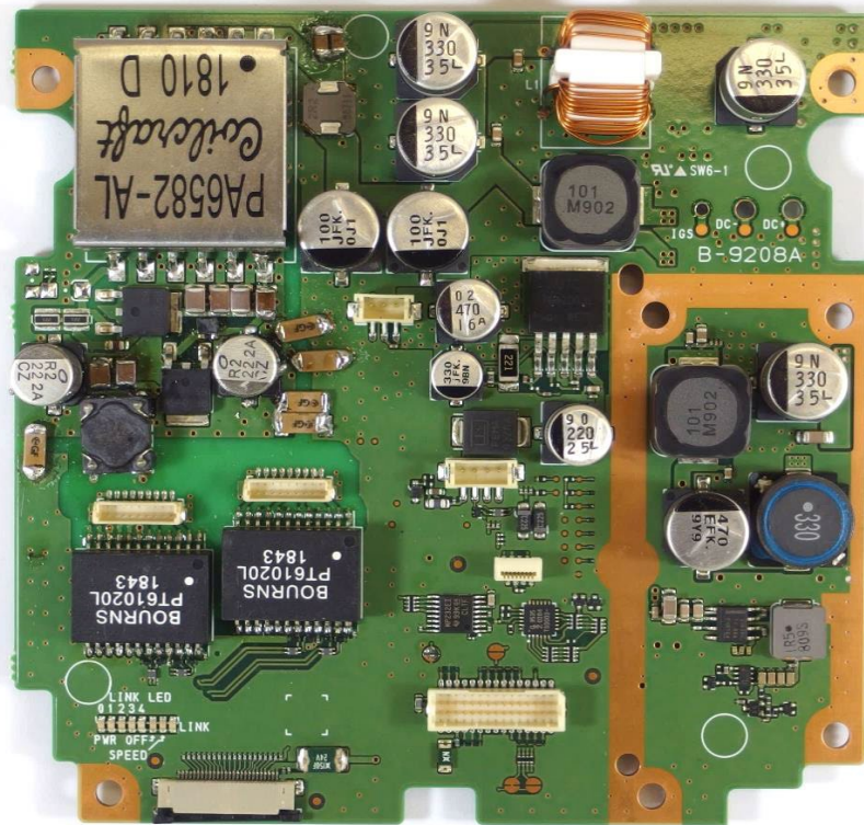
MAIN UNIT BOARD (SIDE A)
