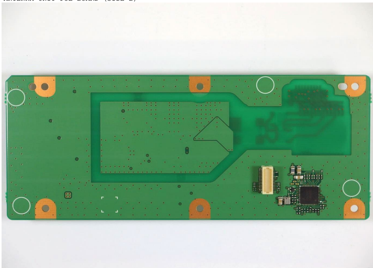
ANTENNA UNIT PoE BOARD (SIDE B)
