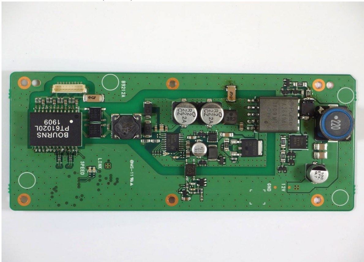
ANTENNA UNIT PoE BOARD (SIDE A)
