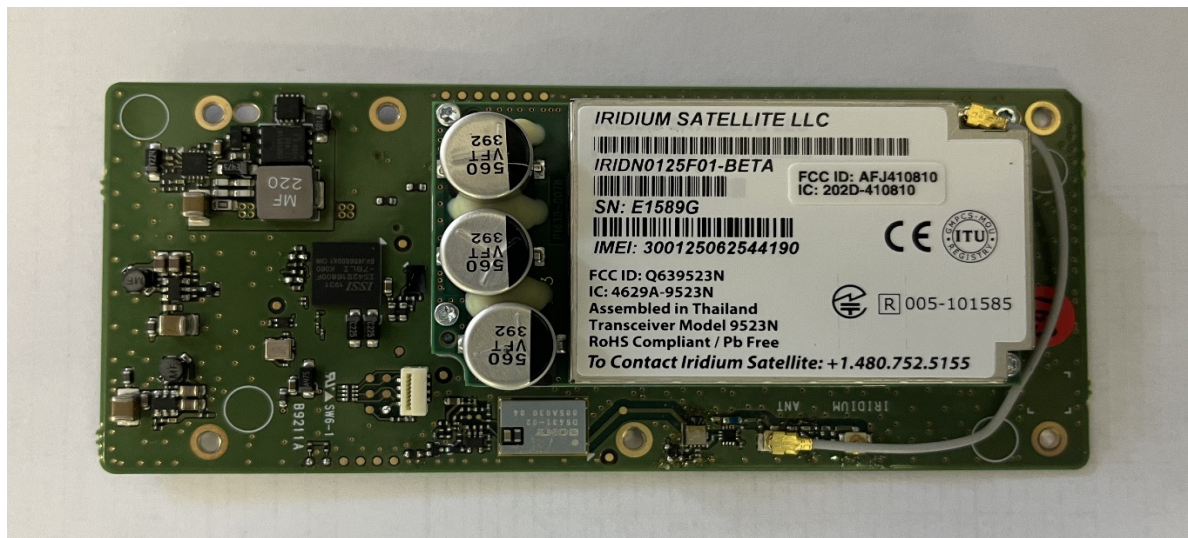
ANTENNA UNIT RF BOARD (SIDE A)
