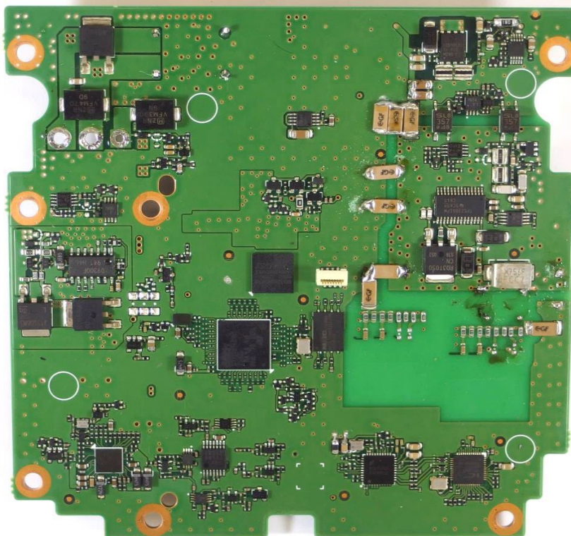
MAIN UNIT BOARD (SIDE B)
