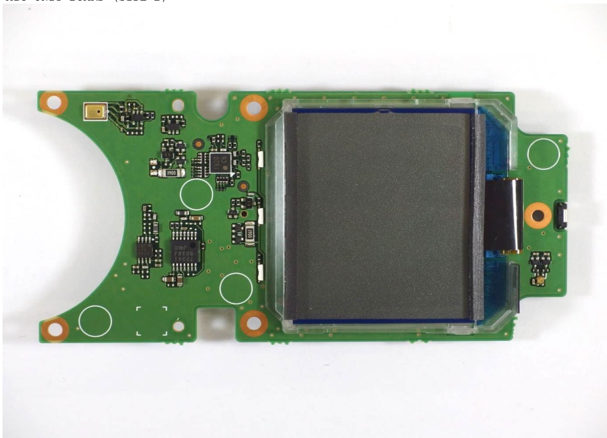
MIC UNIT BOARD (SIDE B)
