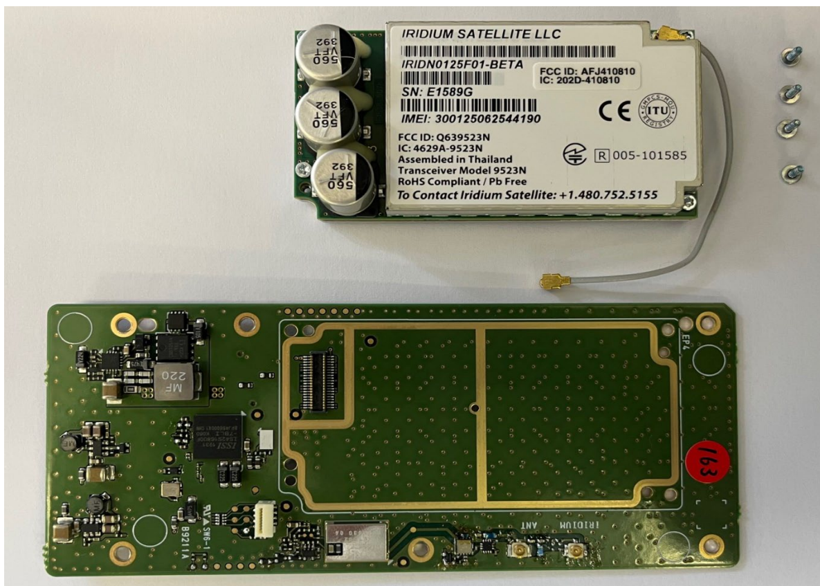
ANTENNA UNIT RF BOARD (SIDE A)
