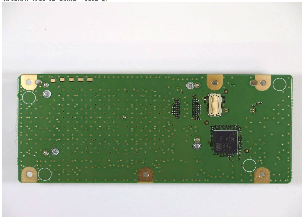
ANTENNA UNIT RF BOARD (SIDE B)
