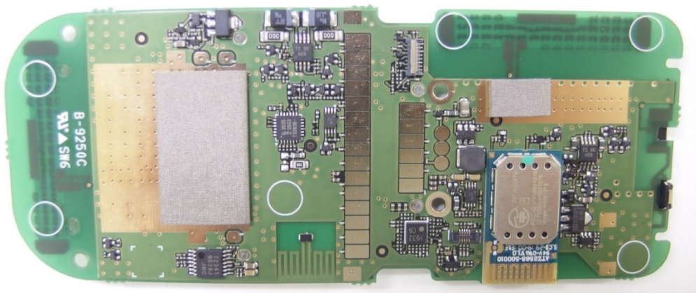
Front Board side-B view
