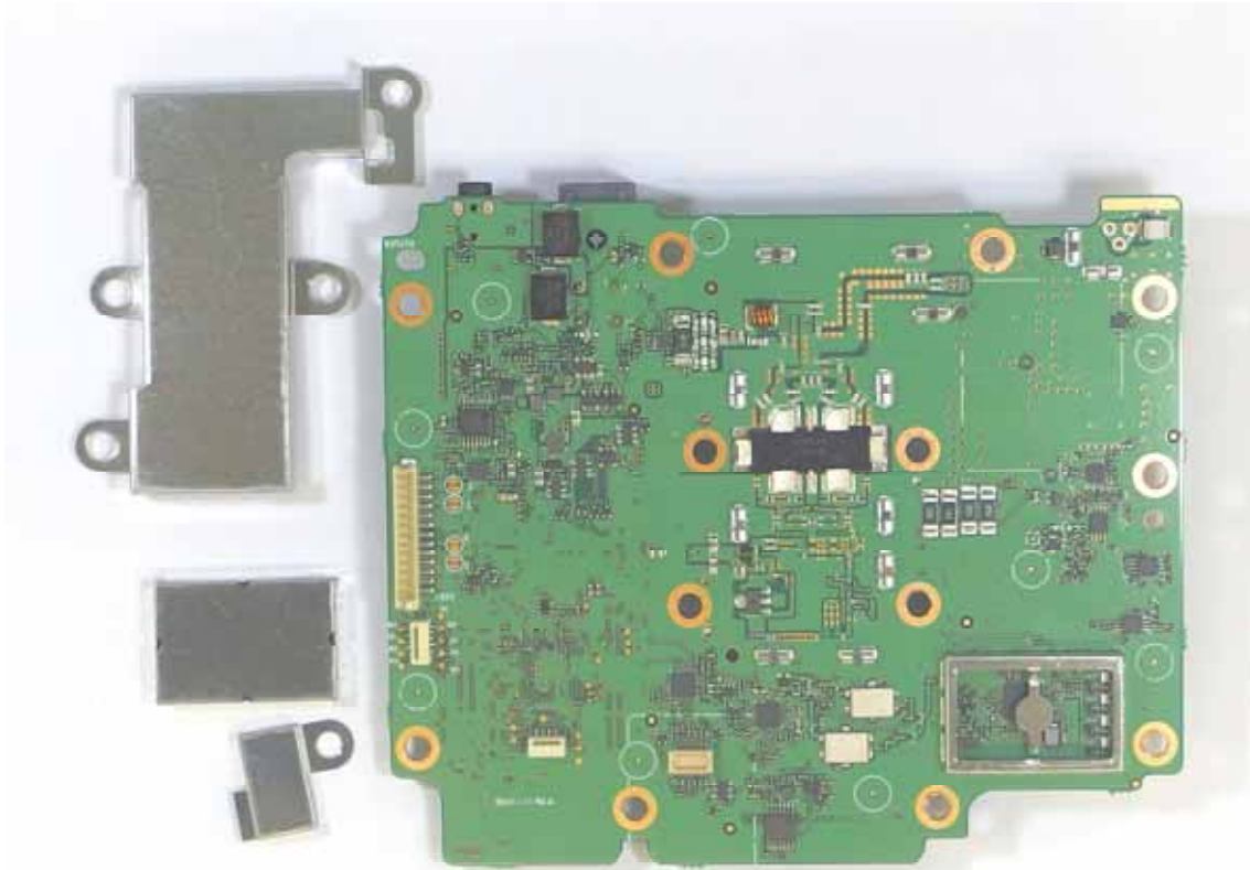
IC-F6130D MAIN unit Main board side-A
