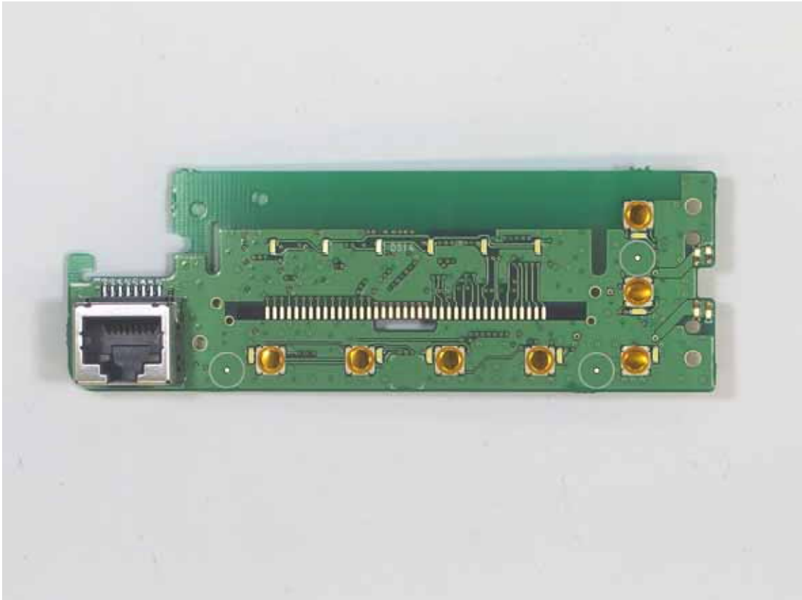
IC-F6130D MAIN unit Front board side-A
