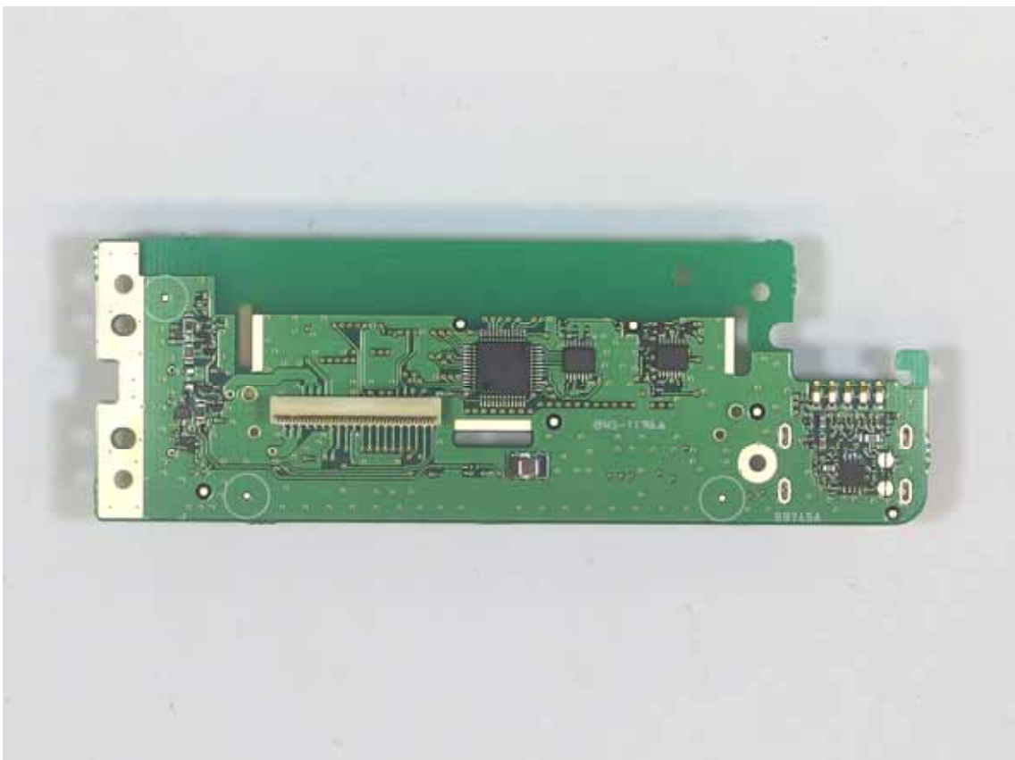
IC-F6130D MAIN unit Front board side-B
