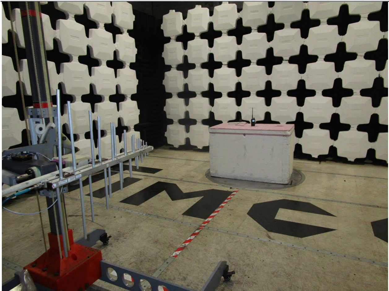
Radiated Testing, Below 1 GHz #2
