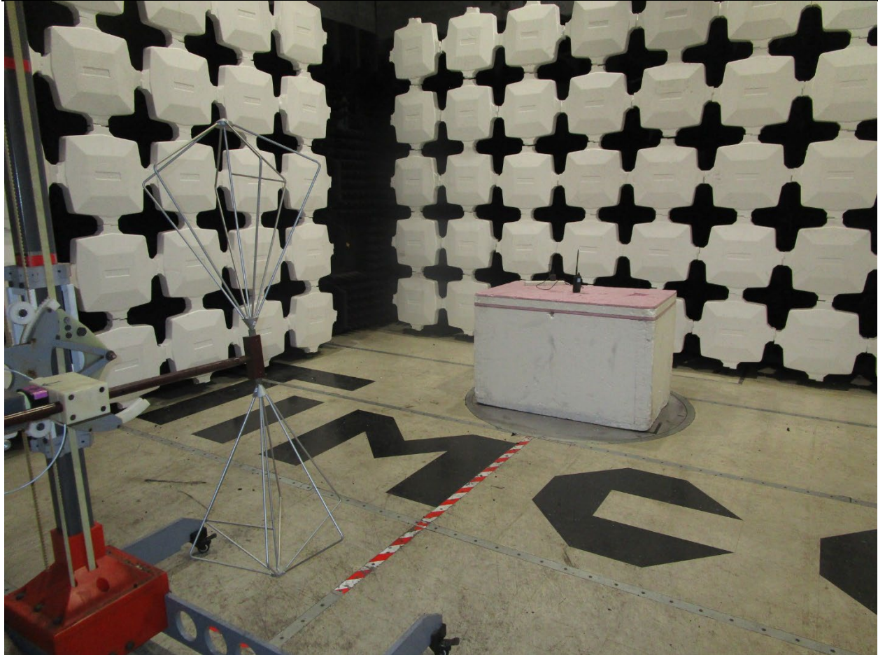
Radiated Testing, Below 1 GHz #1
