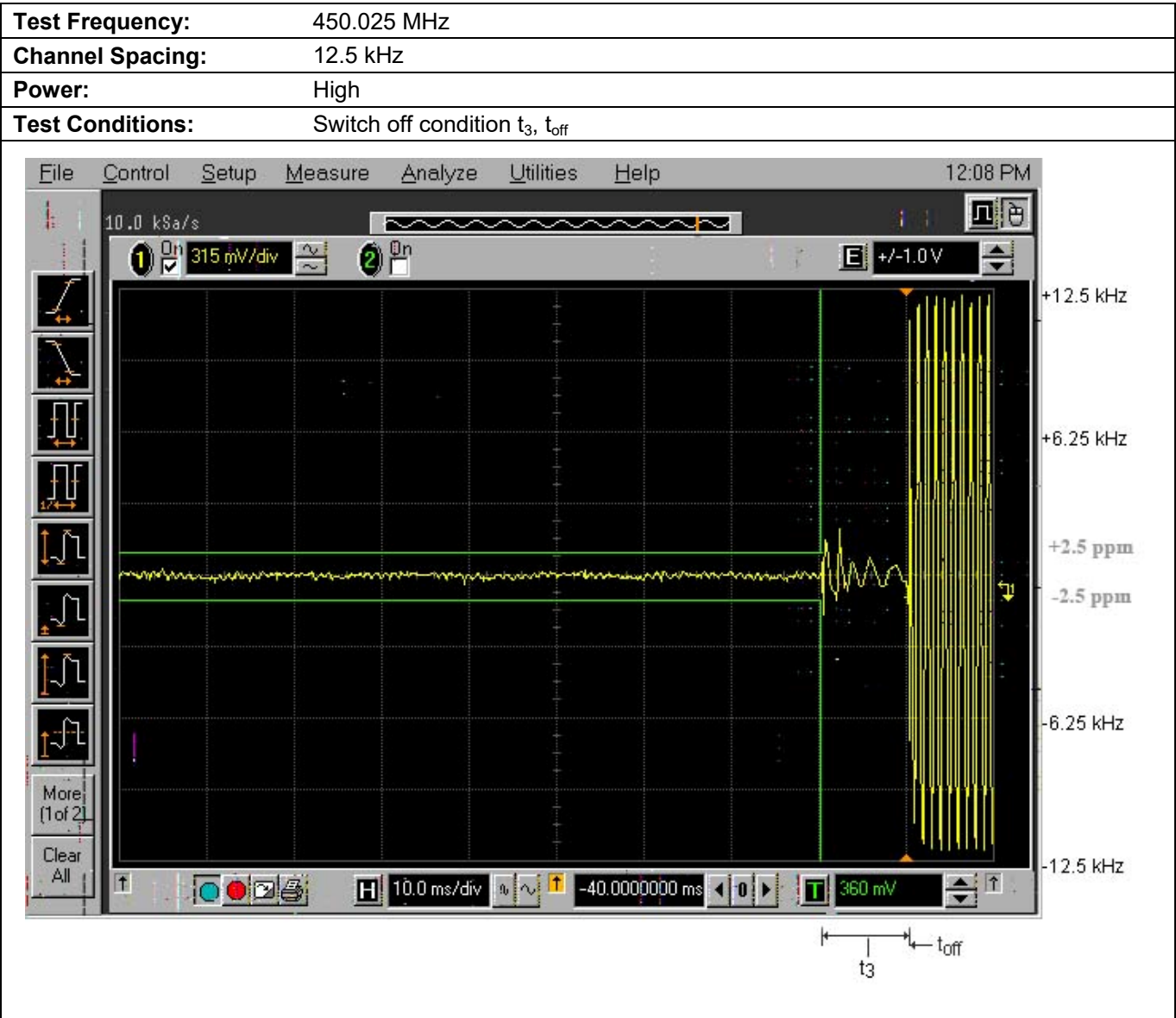
Plot 5.12.3.2. Transient Frequency Behavior for 12.5 kHz Channel Spacing
