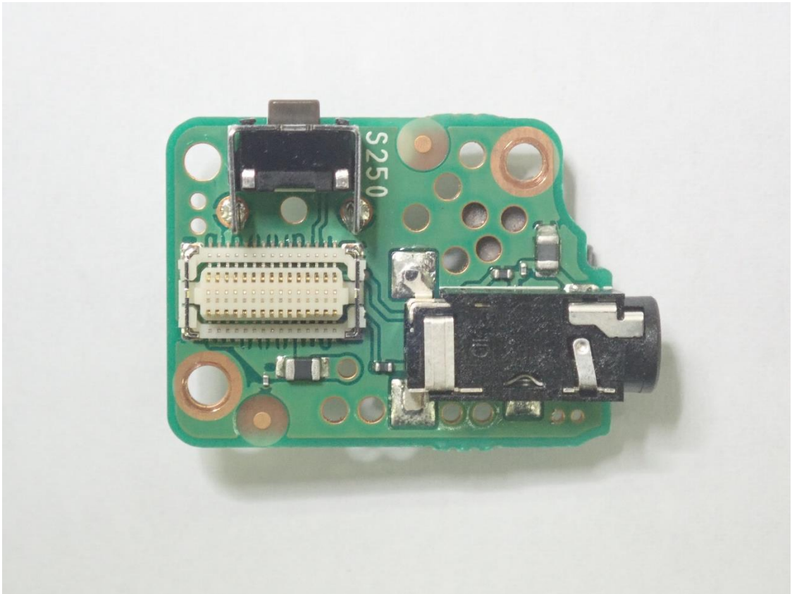
PCB_MIC-A
