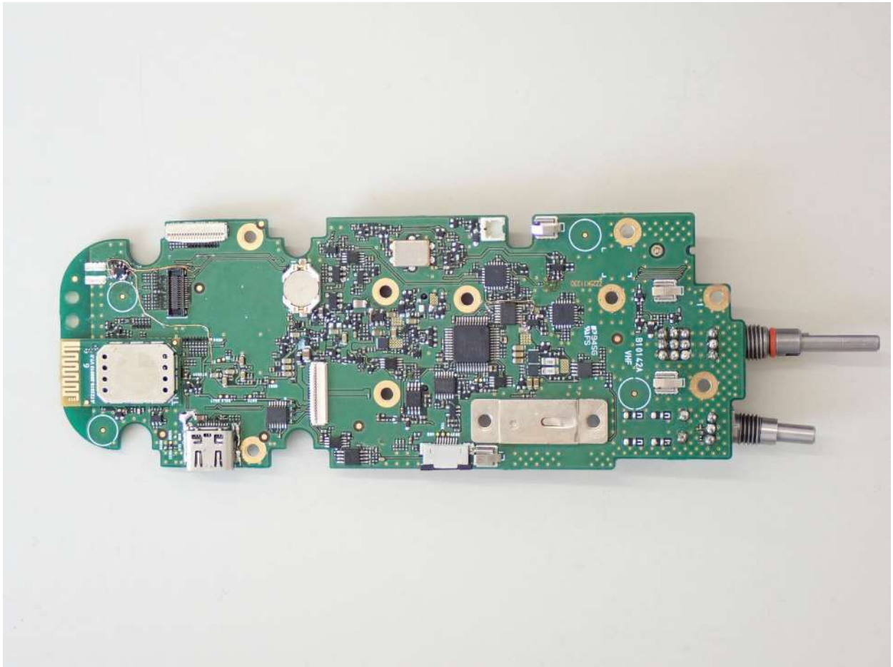
IC-F3600DT MAIN SIDE A
