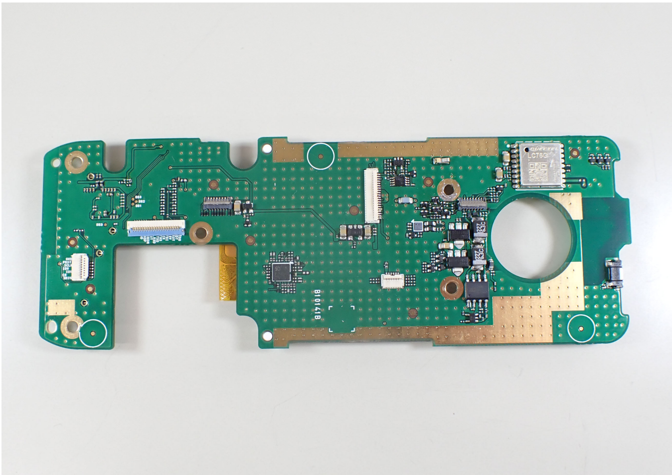
IC-F4600DT FRONT SIDE A
