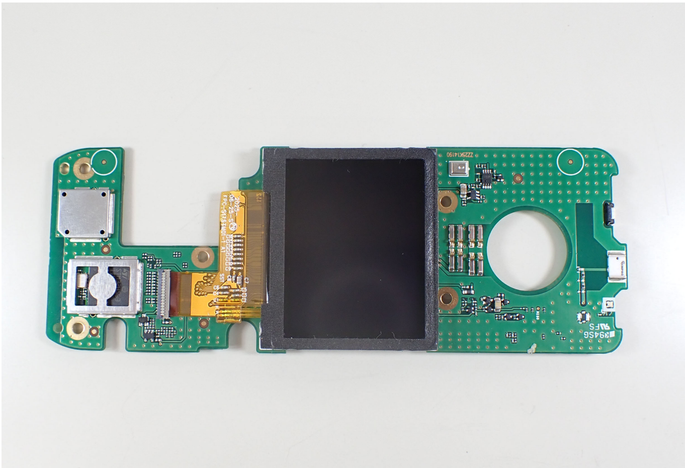
IC-F4600DT FRONT SIDE B
