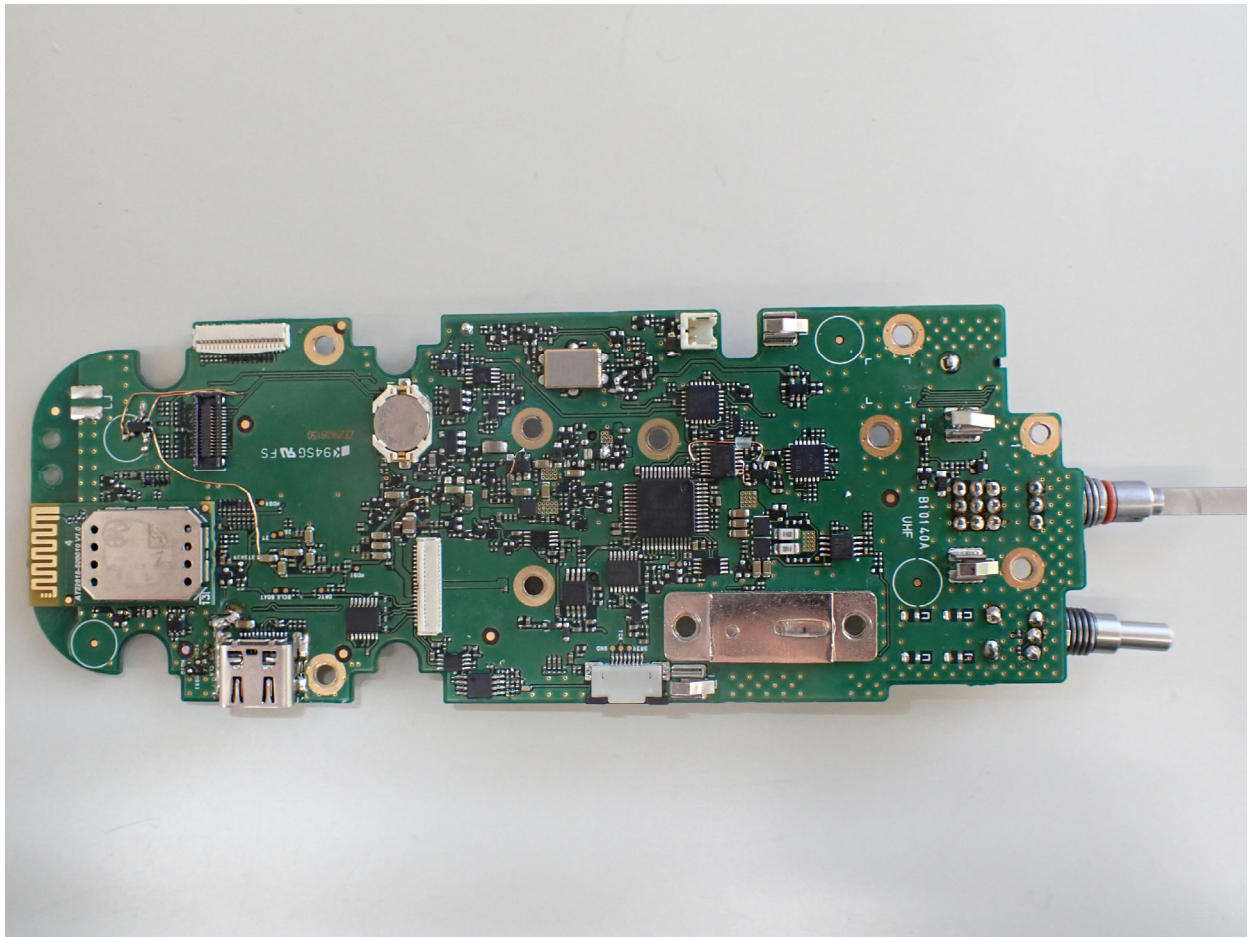
IC-F4600DT MAIN SIDE A
