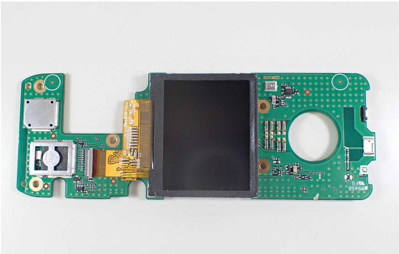
IC-F4600DS FRONT SIDE B
