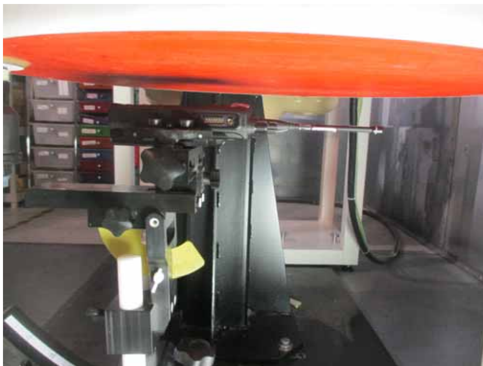
<Face Frontal Position, FA-S76UC 480MHz Antenna, BP-316 battery pack>
