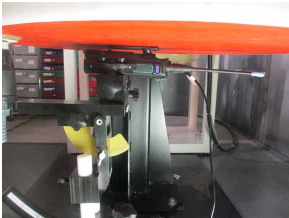
< Belt Clip MB133 Touch Position FA-S76UC 400MHz Antenna, BP-303N battery pack >
