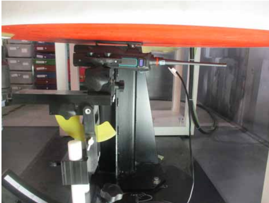
< Belt Clip MB133 Touch Position FA-S83U Antenna, BP-303N battery pack >
