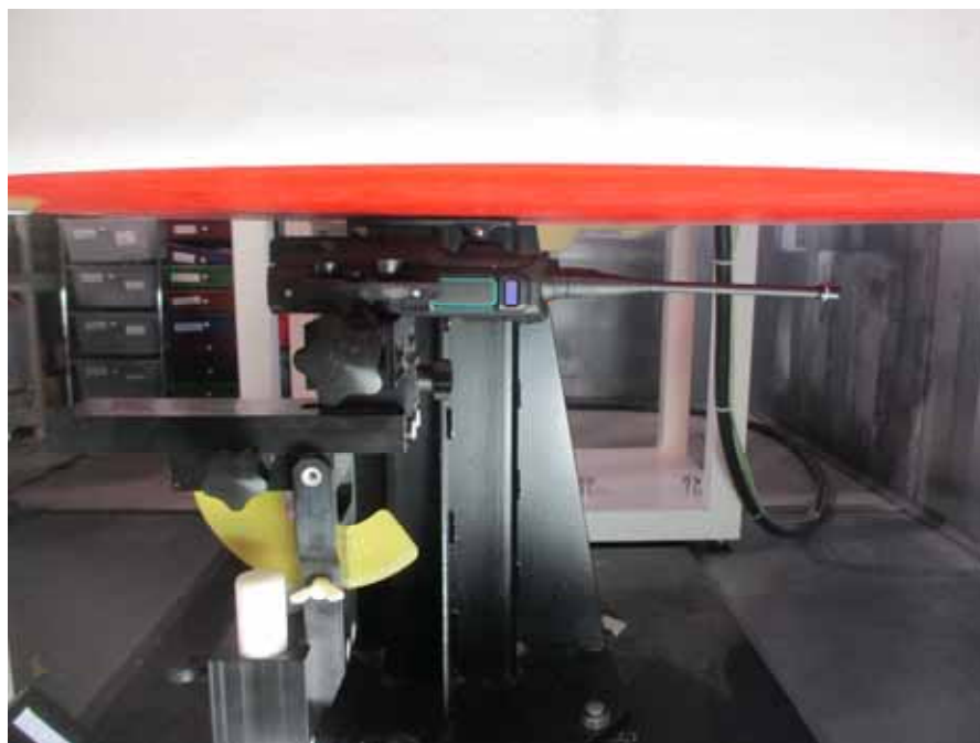
< Belt Clip MB133 Touch Position FA-S76UC 520MHz Antenna, BP-303N battery pack >
