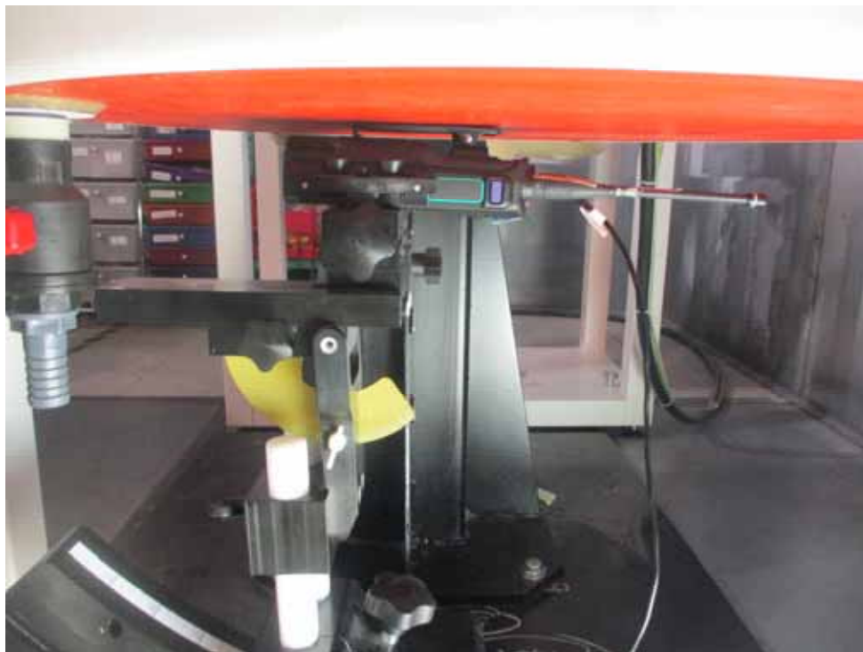
< Belt Clip MB133 Touch Position FA-S76UC 480MHz Antenna, BP-303N battery pack >
