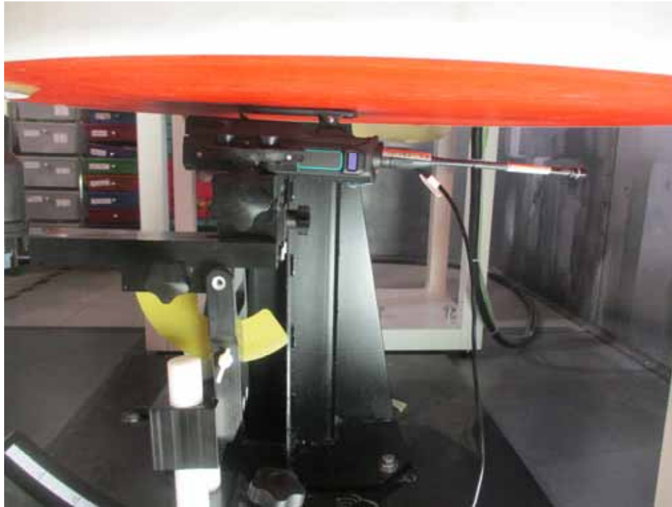
< Belt Clip MB133 Touch Position FA-S76UC 420MHz Antenna, BP-303N battery pack >
