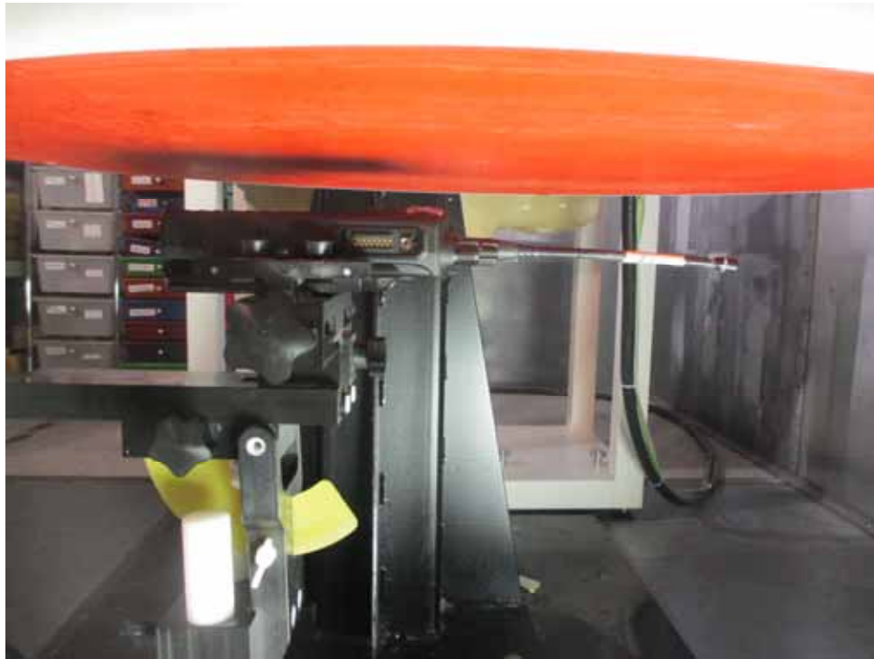
<Face Frontal Position, FA-S76UC 420MHz Antenna, BP-316 battery pack>
