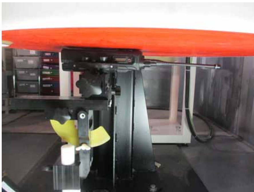
<Face Frontal Position, FA-S76UC 520MHz Antenna, BP-316 battery pack>
