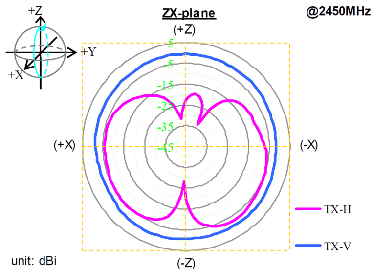
Fig.3: Radiation pattern ZX-plane
