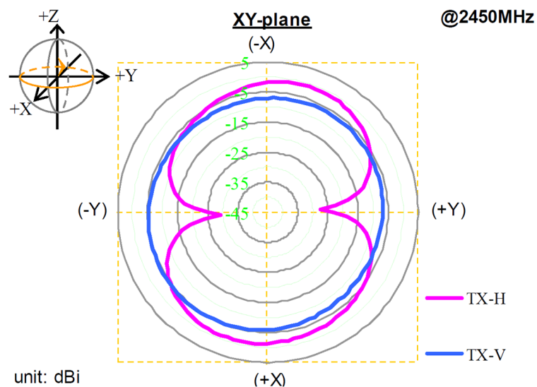
Fig.1: Radiation pattern XY-plane
