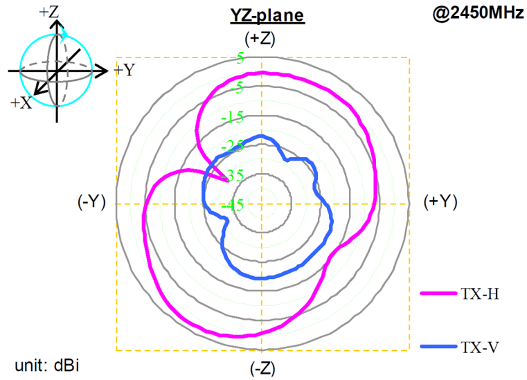
Fig.2: Radiation pattern YZ-plane
