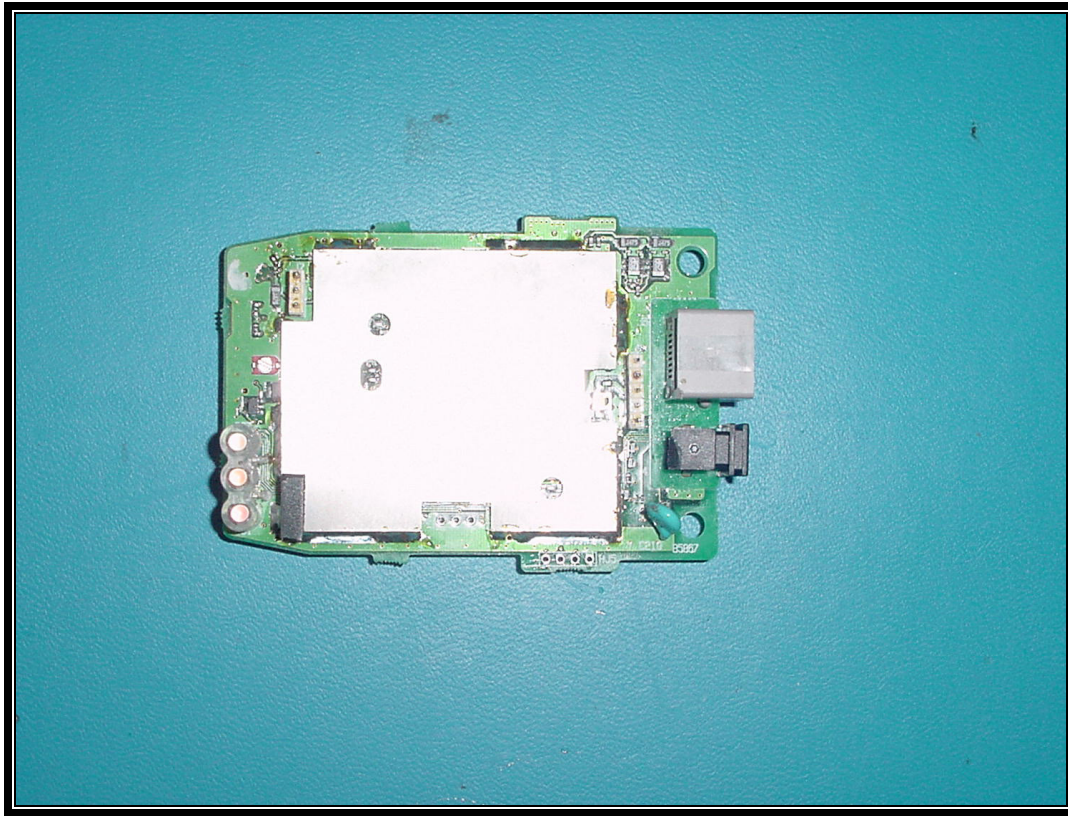
PHOTOGRAPH 11: TOP VIEW MAIN PCB WITH SHIELD
