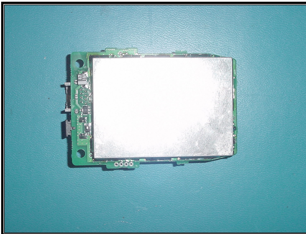
PHOTOGRAPH 12: BOTTOM VIEW MAIN PCB WITH SHIELD
