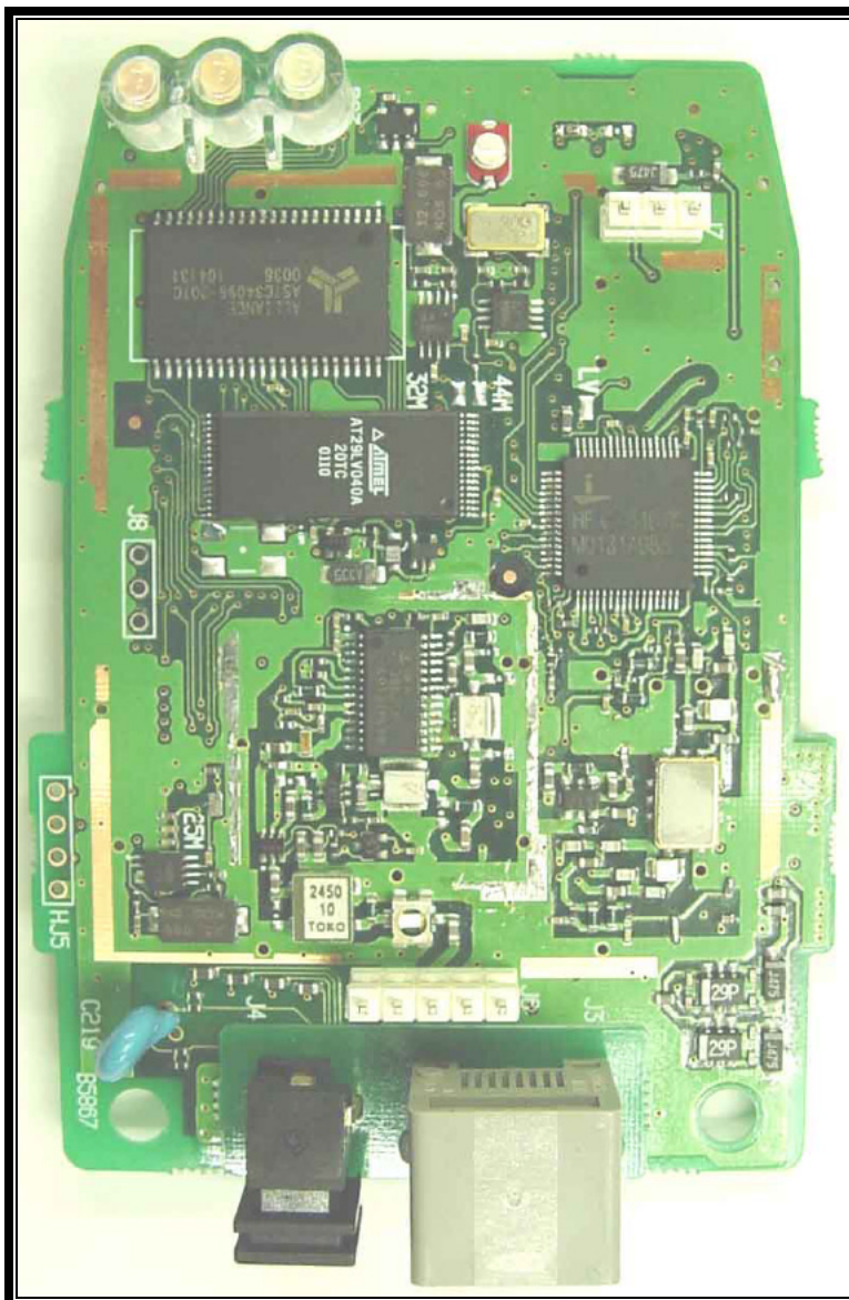
PHOTOGRAPH 13: TOP VIEW MAIN PCB WITHOUT SHIELD
