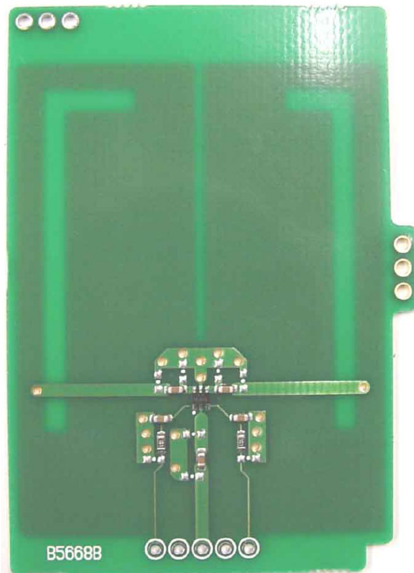
PHOTOGRAPH 10: BOTTOM VIEW OF ANTENNA
