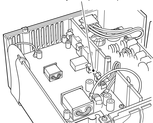
Circuitry fuse (FGB 5 A)
