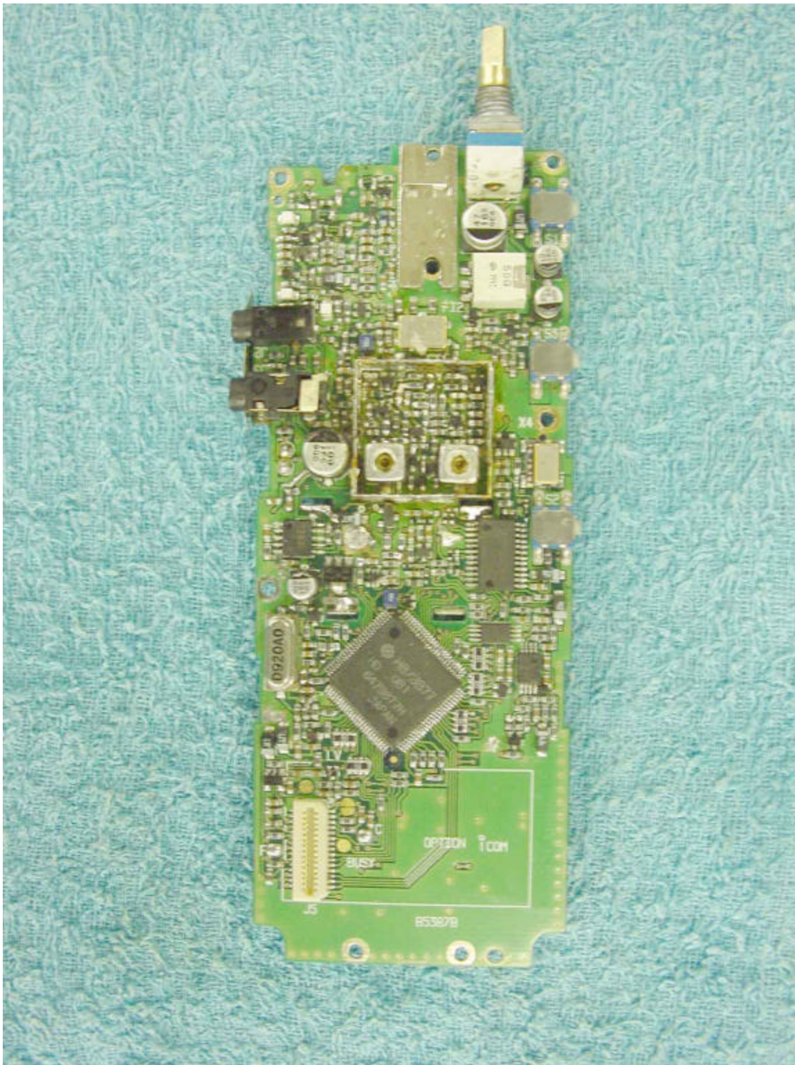
Icom Incorporated UHF Transceiver, Model IC-F4GT-4 / IC-F4GS-4 FCC ID: AFJIC-F4G-4
