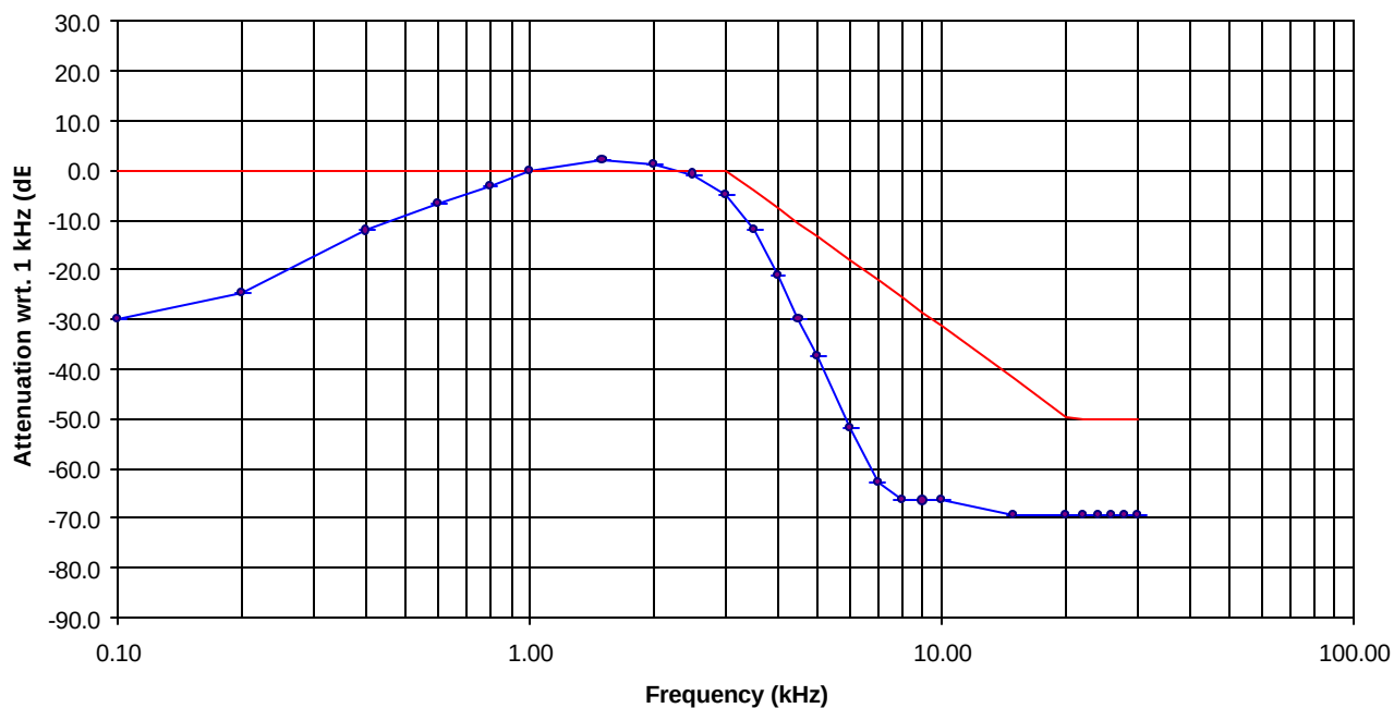
AUDIO FREQUENCY REPSONSE @ FCC 2.987(a) UHF Transceiver, Model IC-F4GT-4 / IC-F4GS-4, FCC ID: AFJIC-F4G-4
