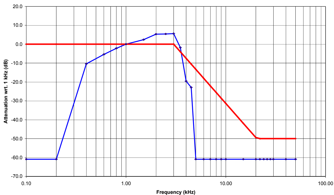
AUDIO FREQUENCY RESPONSE @ FCC 2.1047(a) & 90.242b(8) VHF FM Transceiver, Model IC-F521 (25 kHz Channel Spacing)
