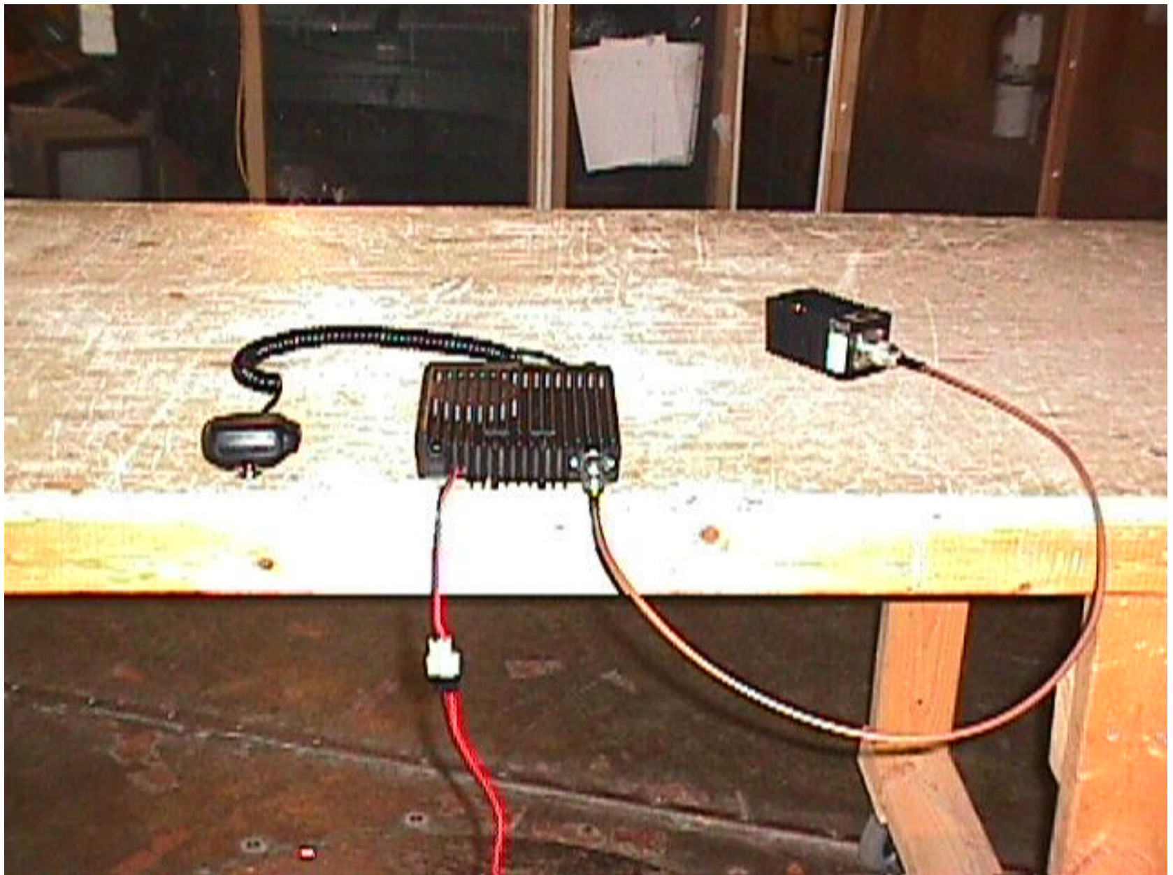
ANNEX 2 - PHOTO OF TEST SETUP Mobile UHF FM Transceiver, Model IC-F620-1
