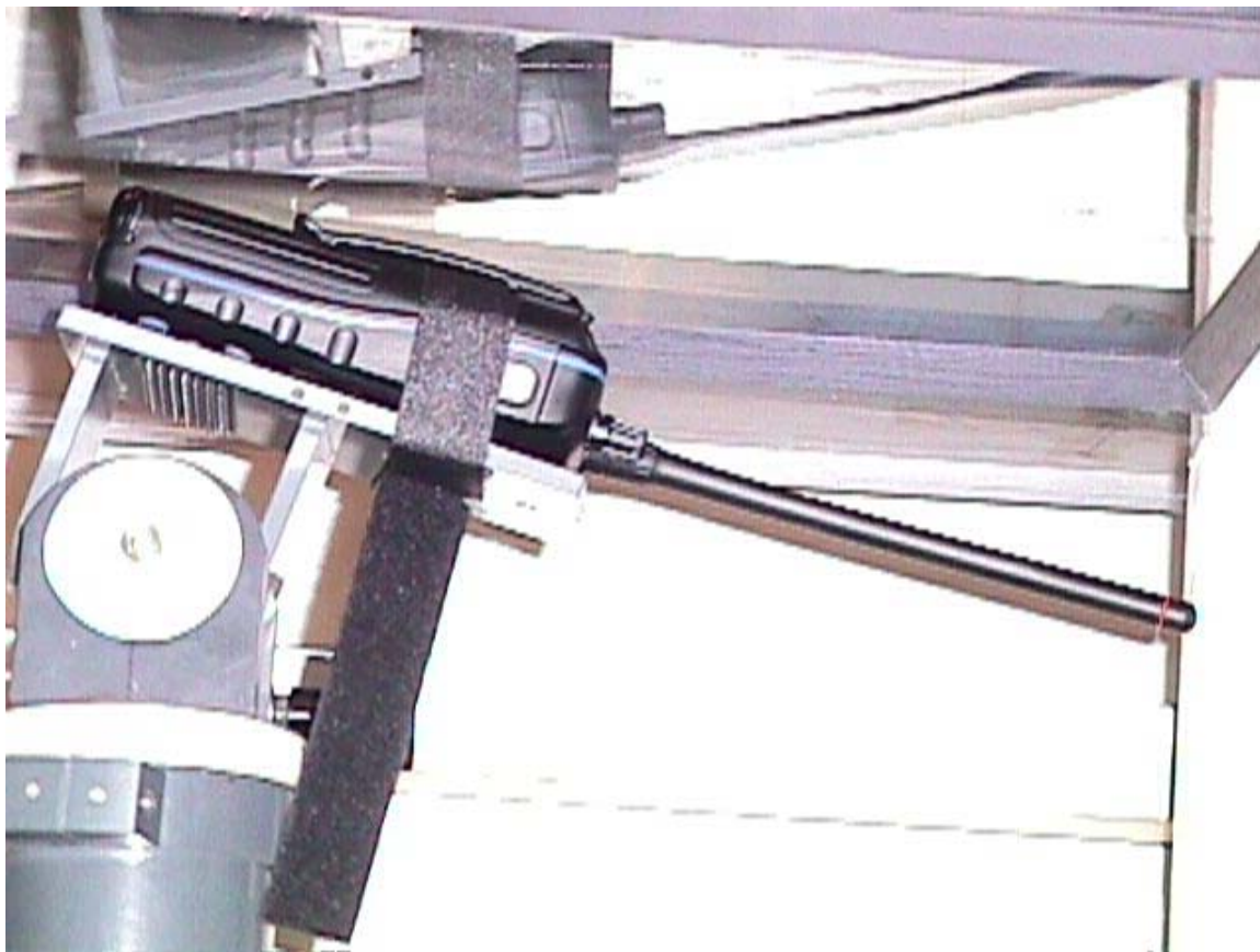
< The bottom of the EUT in contact with the phantom with the belt clip(M/N: MB-68) – Closeup-View >
