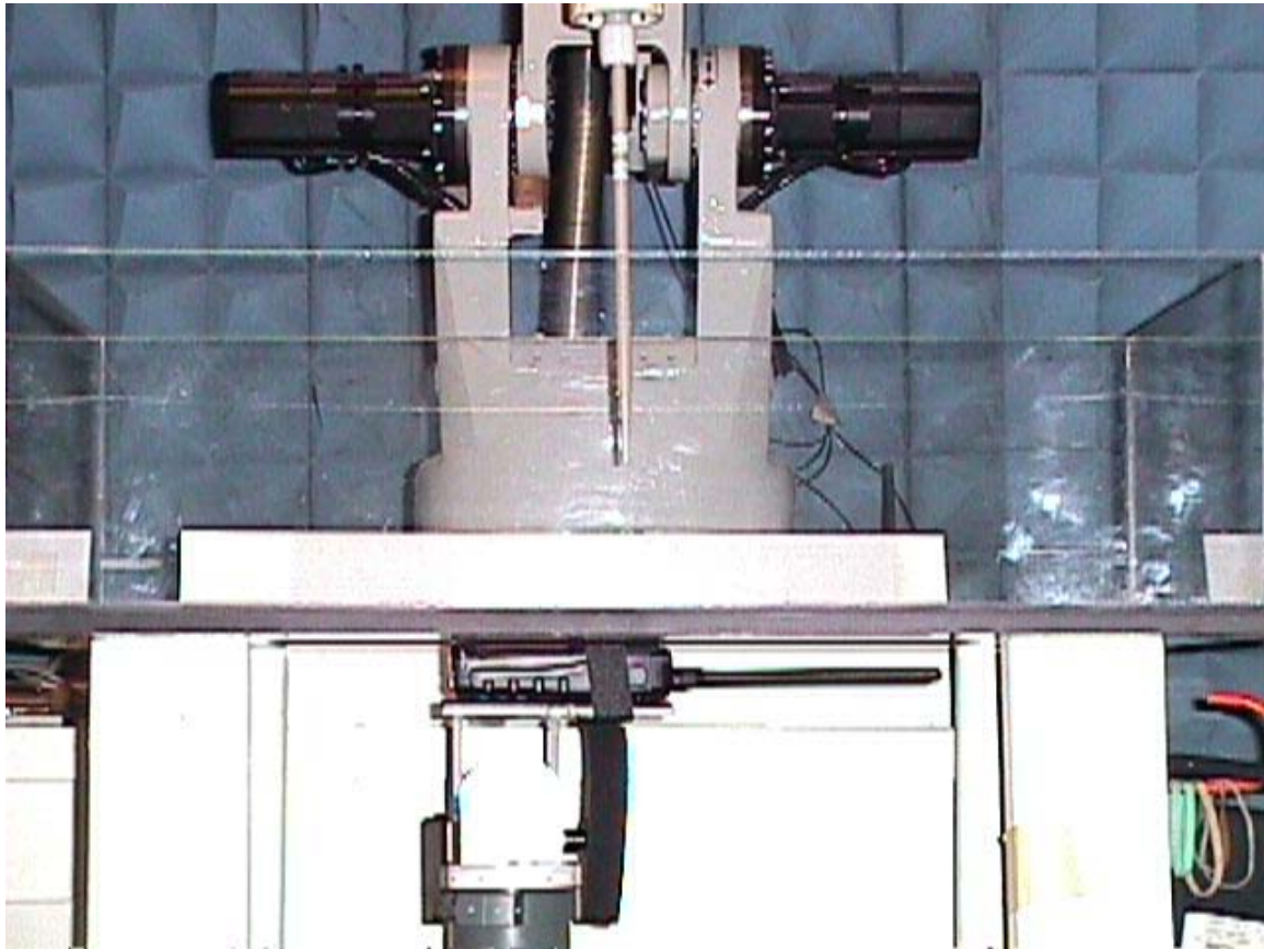
< The EUT parallel to the phantom with the belt clip(M/N: MB-68) – Overview >
