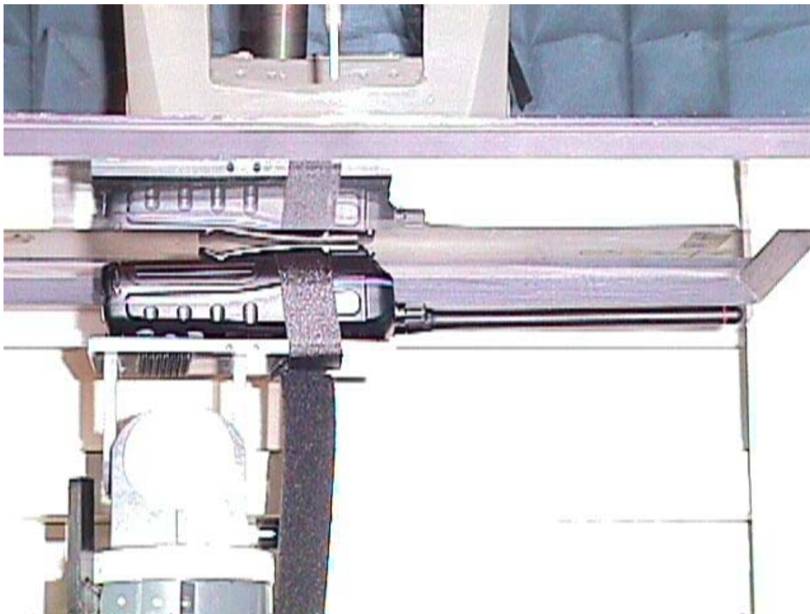
< The EUT parallel to the phantom with the belt clip(M/N: MB-68) – Closeup-View >
