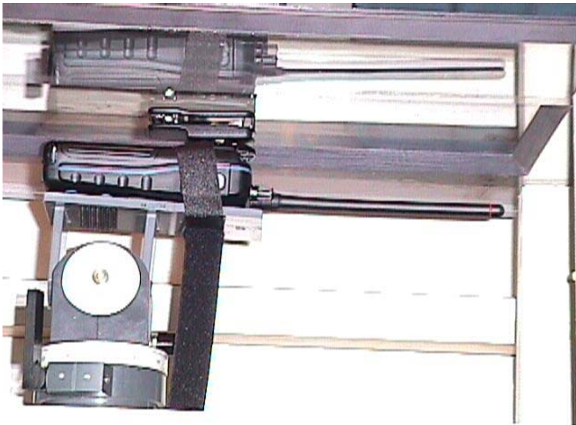
< The EUT parallel to the phantom with the rotary belt clip(M/N: MB-87) – Closeup -iew >
