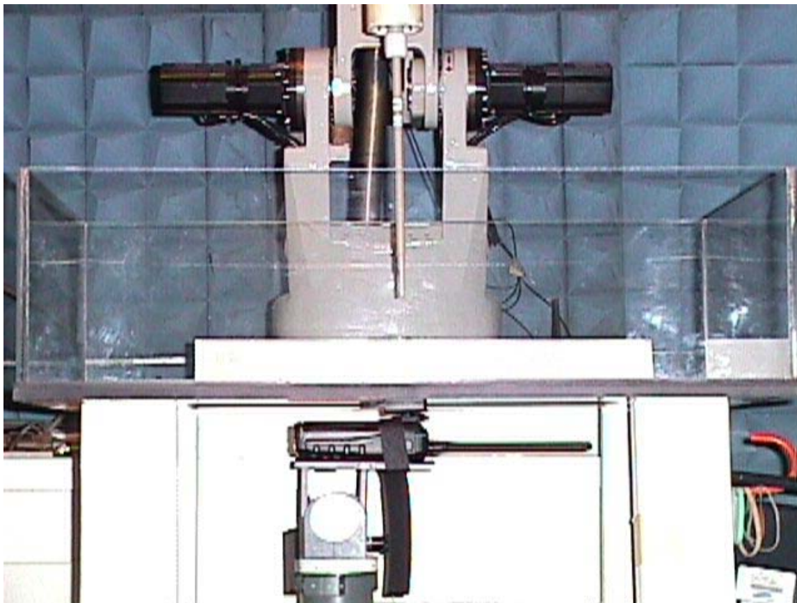
< The EUT parallel to the phantom with the rotary belt clip(M/N: MB-87) – Overview >
