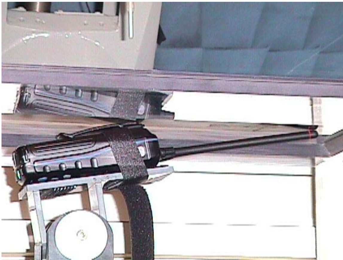
< The tip of the antenna in contact with the phantom with the belt clip(M/N: MB-68) – Closeup-View >
