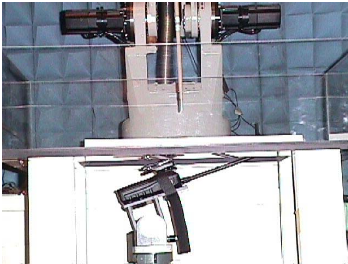
< The tip of the antenna in contact with the phantom with the rotary belt clip(M/N: MB-87) – Overview >
