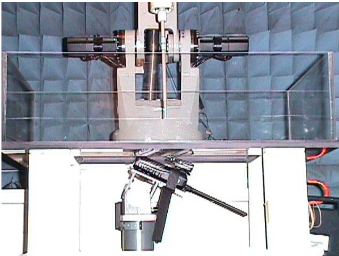
< The bottom of the EUT in contact with the phantom with the rotary belt clip(M/N: MB-87) – Overview >
