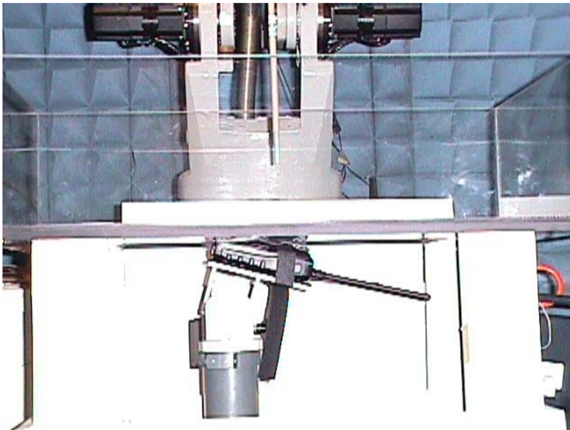
< The bottom of the EUT in contact with the phantom with the belt clip(M/N: MB-68) – Overview >
