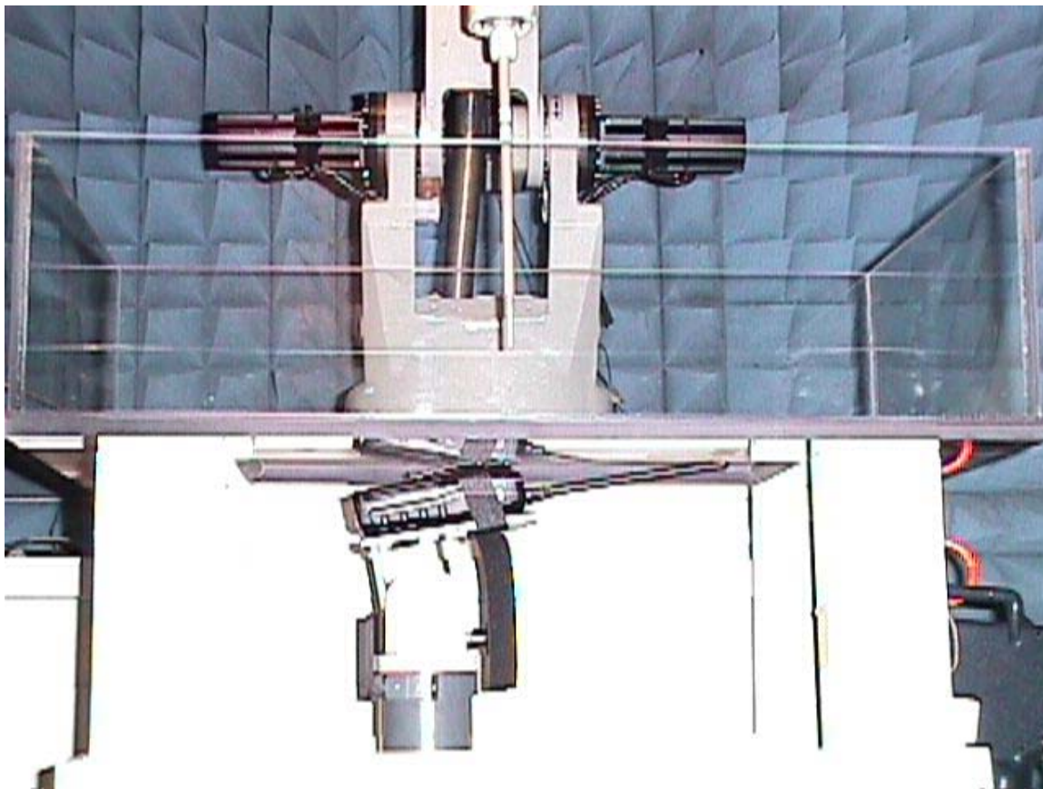
< The tip of the antenna in contact with the phantom with the belt clip(M/N: MB-68) – Overview >
