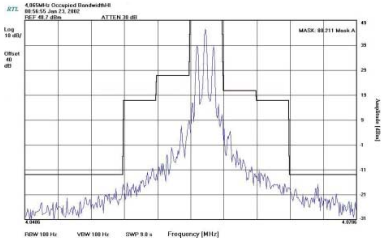
PLOT 5-14: OCCUPIED BANDWIDTH (3KHZ): CHANNEL FREQUENCY 4.065MHZ H3E
