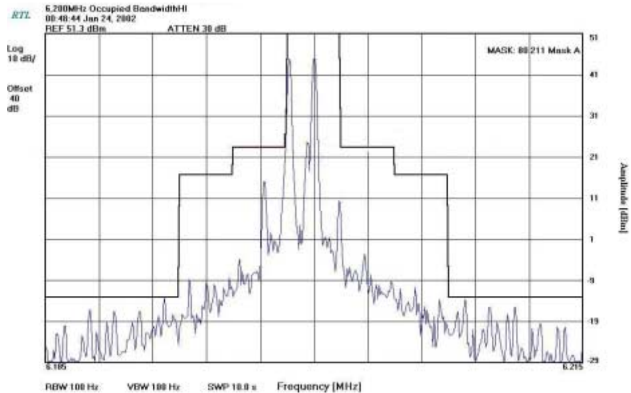
PLOT 5-26: OCCUPIED BANDWIDTH (3KHZ): CHANNEL FREQUENCY 6.200MHZ J2B
