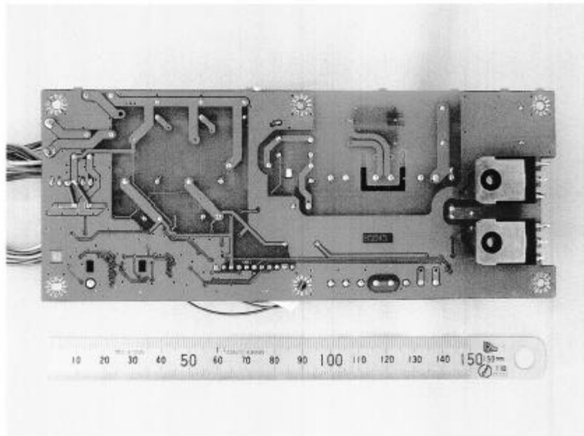
PA Board B side view
