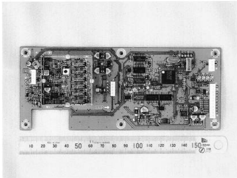
IF Board B side view
