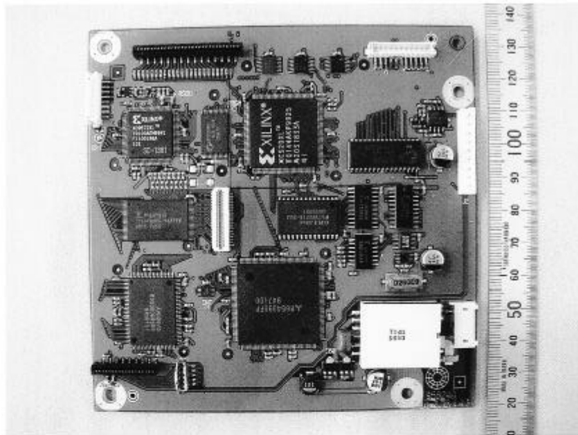
LOGIC Board B side view
