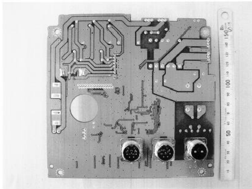
MAIN Board B side view
