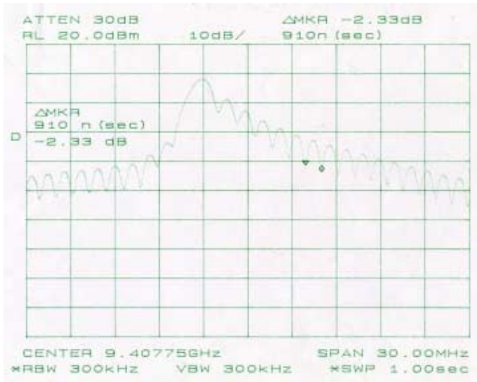
PLOT 4: PULSE LENGTH (0.91 MICROSECONDS)
