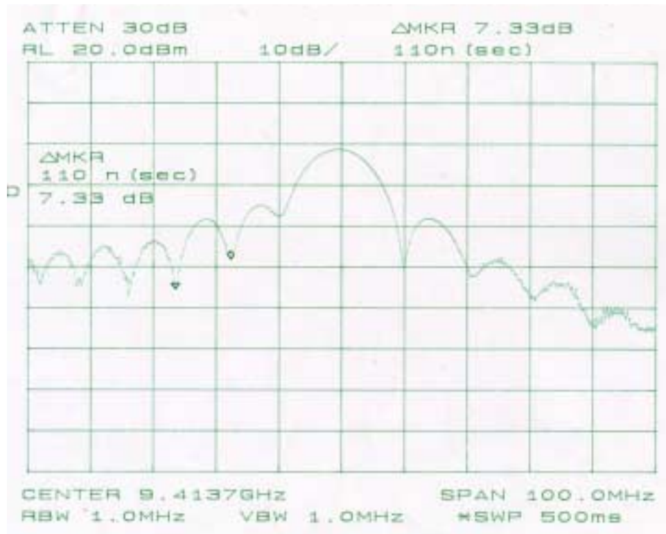
PLOT 1: PULSE LENGTH (0.11 MICROSECONDS)
