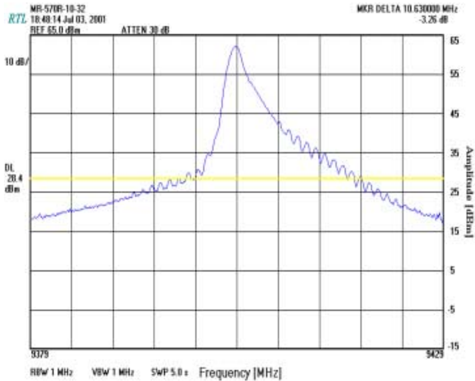
PLOT 8: BANDWIDTH 10.63 MHZ (0.36 MICROSECONDS PULSE LENGTH)
