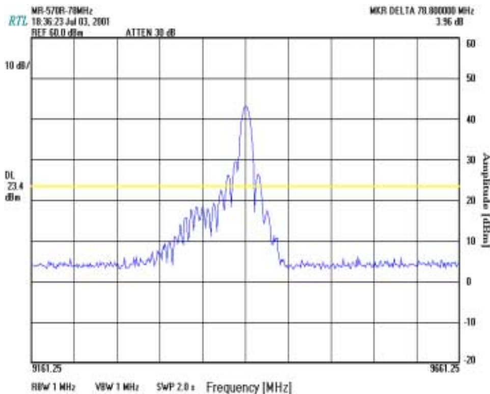
PLOT 5: BANDWIDTH 78.8 MHZ (0.11 MICROSECONDS PULSE LENGTH)
