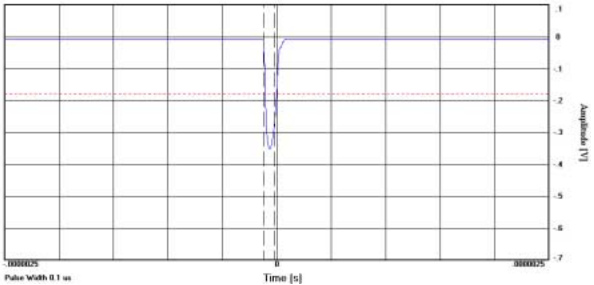
PLOT 9: MAGNETRON CONTROL PULSE 0.1 \mu S
