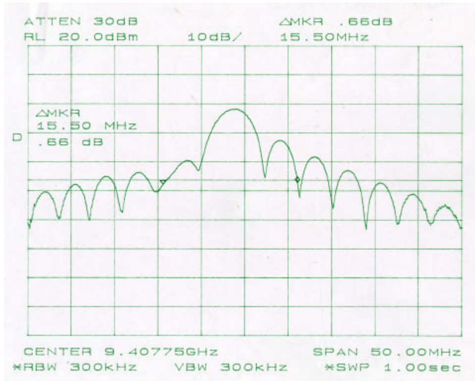
PLOT 6: BANDWIDTH (0.29 MICROSECONDS PULSE LENGTH)
