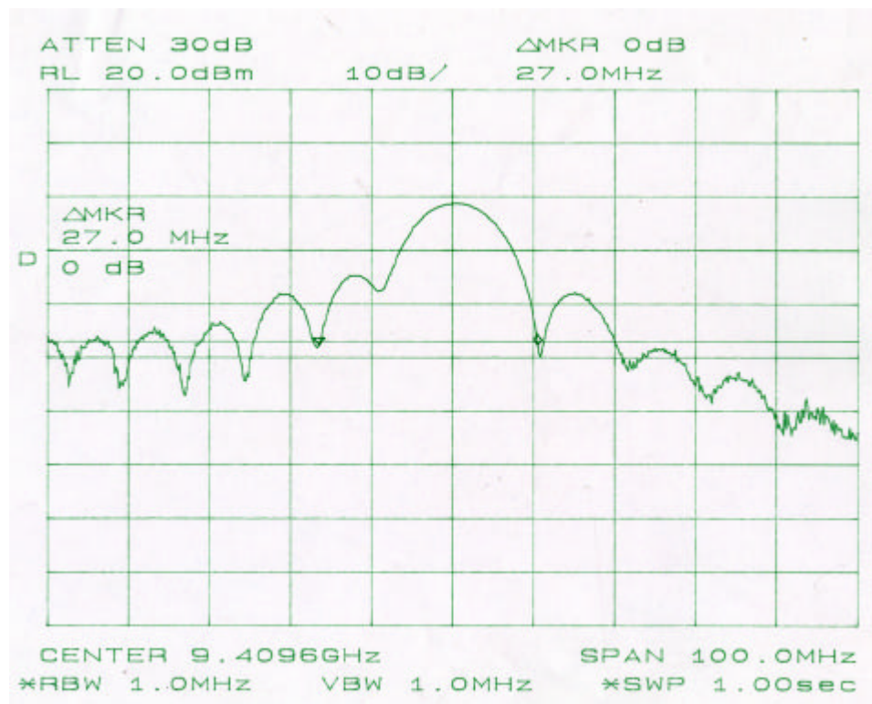
PLOT 5: BANDWIDTH (0.11 MICROSECONDS PULSE LENGTH)
