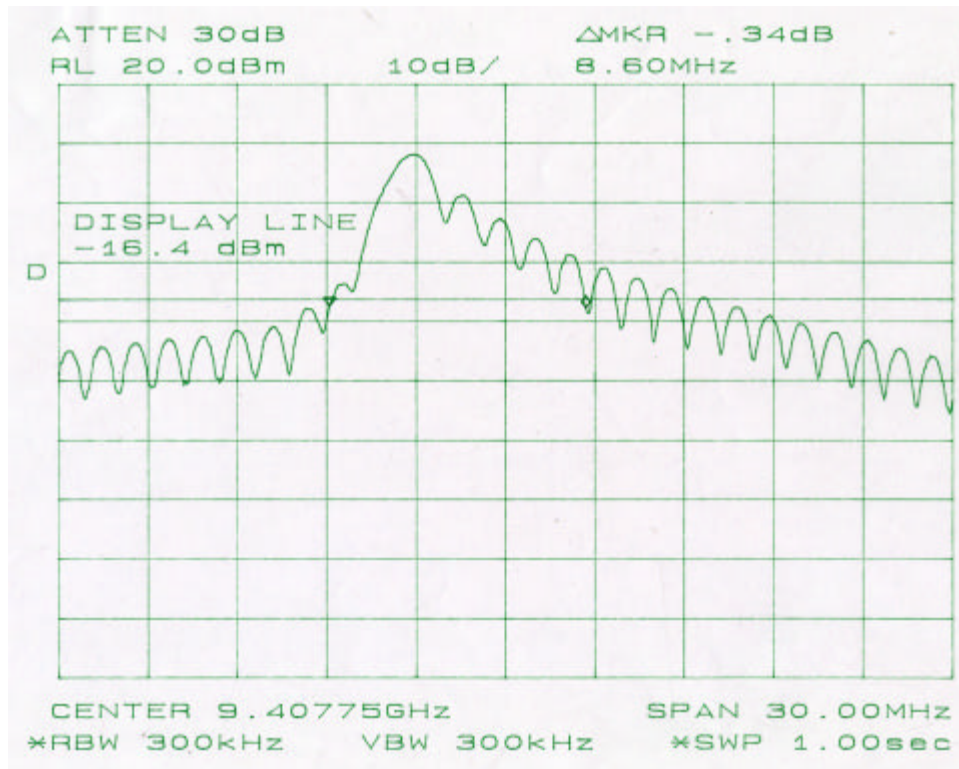
PLOT 8: BANDWIDTH (0.36 MICROSECONDS PULSE LENGTH)
