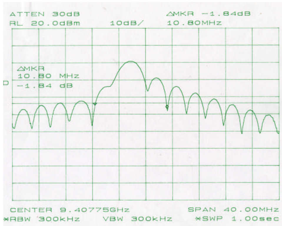
PLOT 7: BANDWIDTH (0.36 MICROSECONDS PULSE LENGTH)
