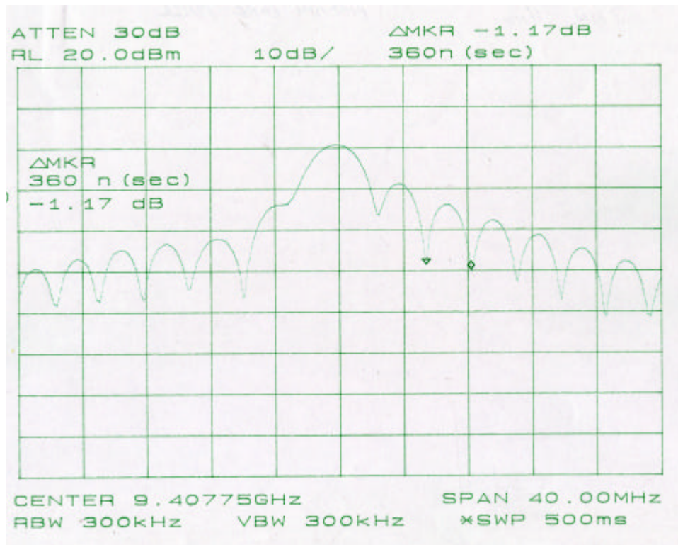
PLOT 3 PULSE LENGTH (0.36 MICROSECONDS)
