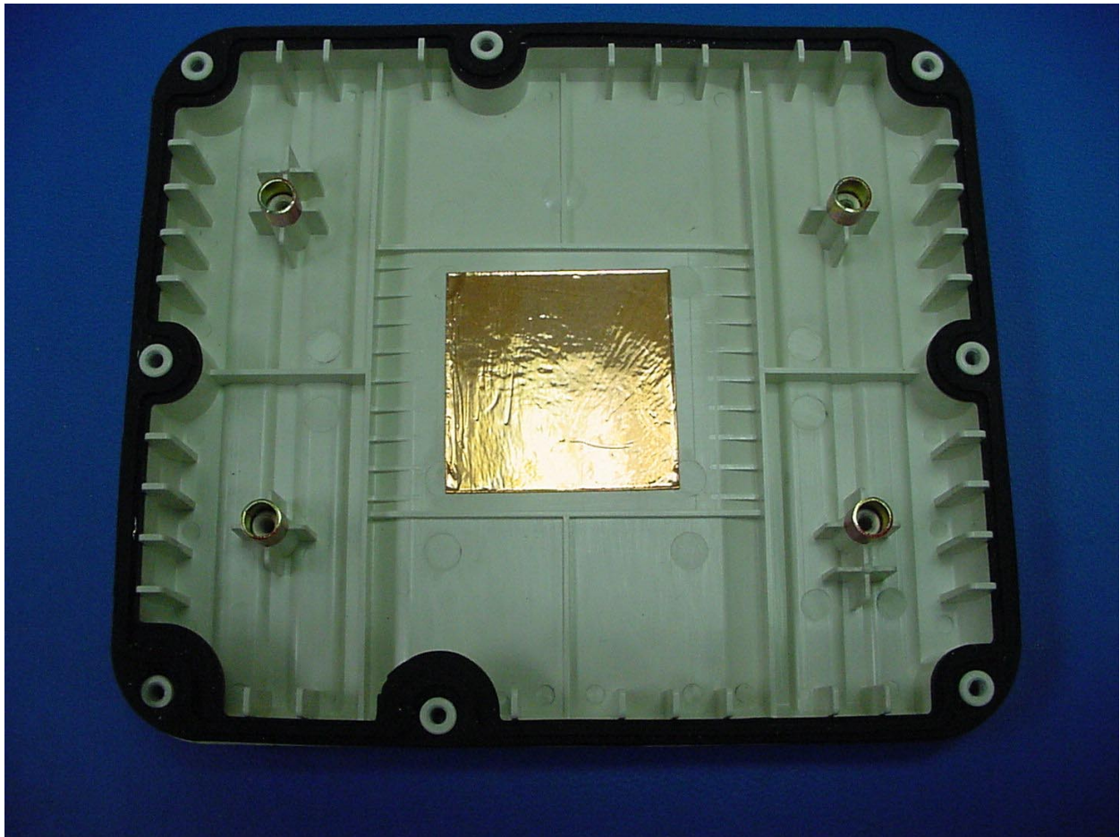
PHOTOGRAPH 14: INSIDE VIEW OF REMOVABLE COVE WITHOUT ANTENNA
