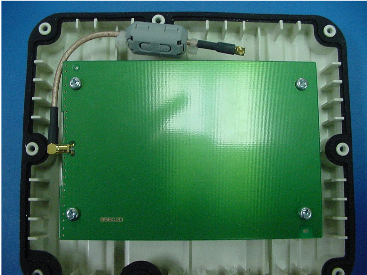
PHOTOGRAPH 13: BOTTOM VIEW OF ANTENNA IN THE REMOVABLE COVER
