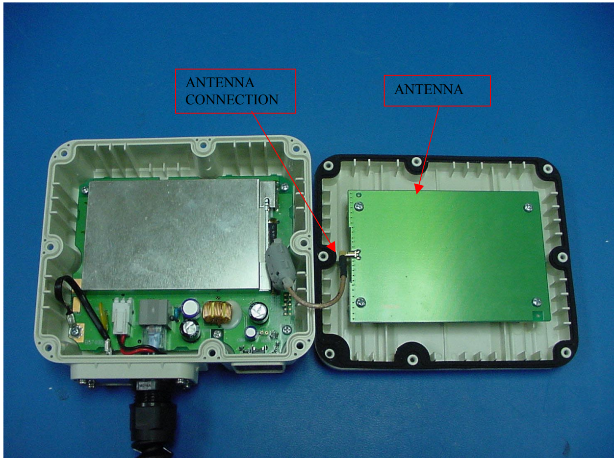
PHOTOGRAPH 12: TOP VIEW WITH COVER REMOVED
