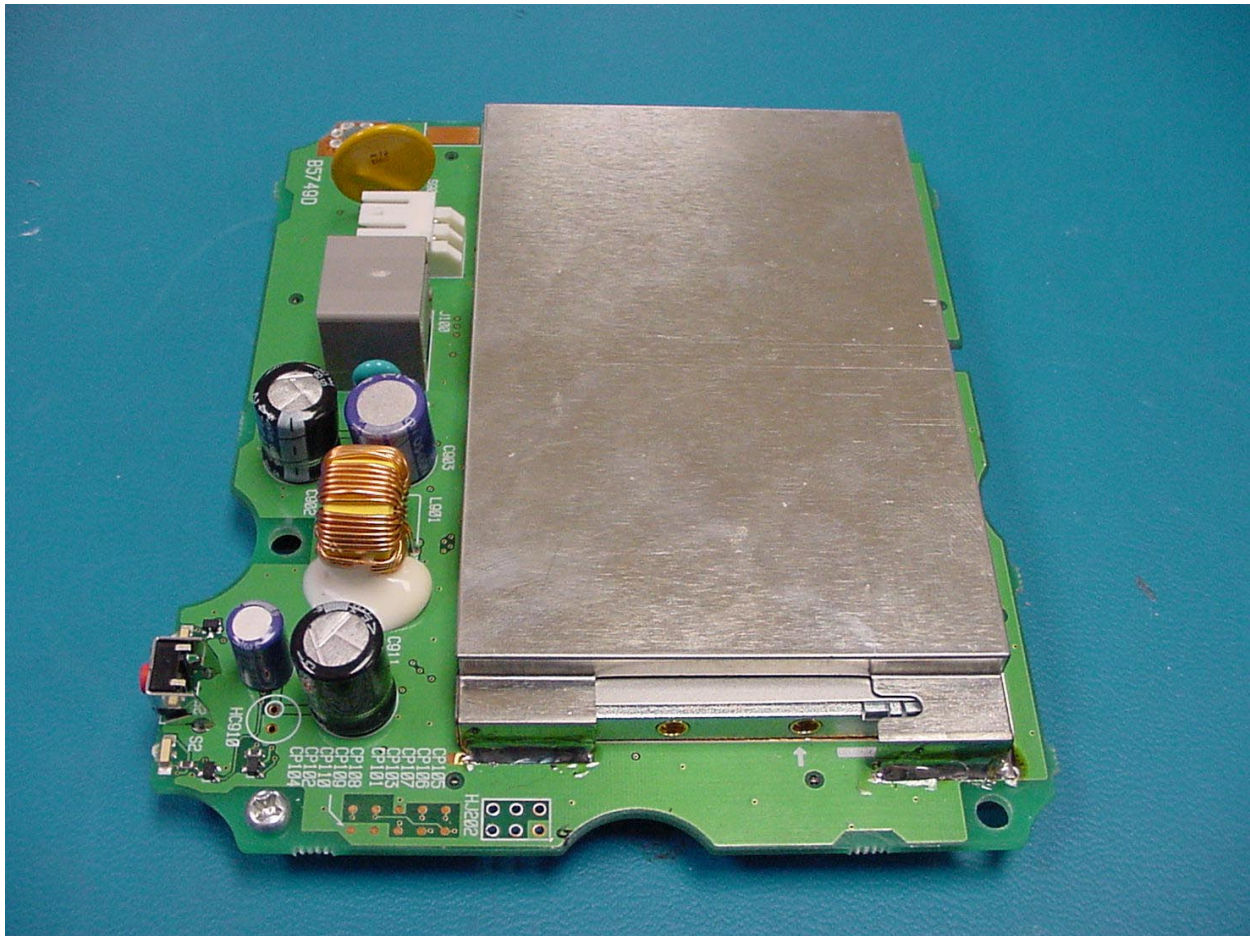
PHOTOGRAPH 17: TOP VIEW OF MAIN PCB BOARD REMOVED FROM CHASSIS
