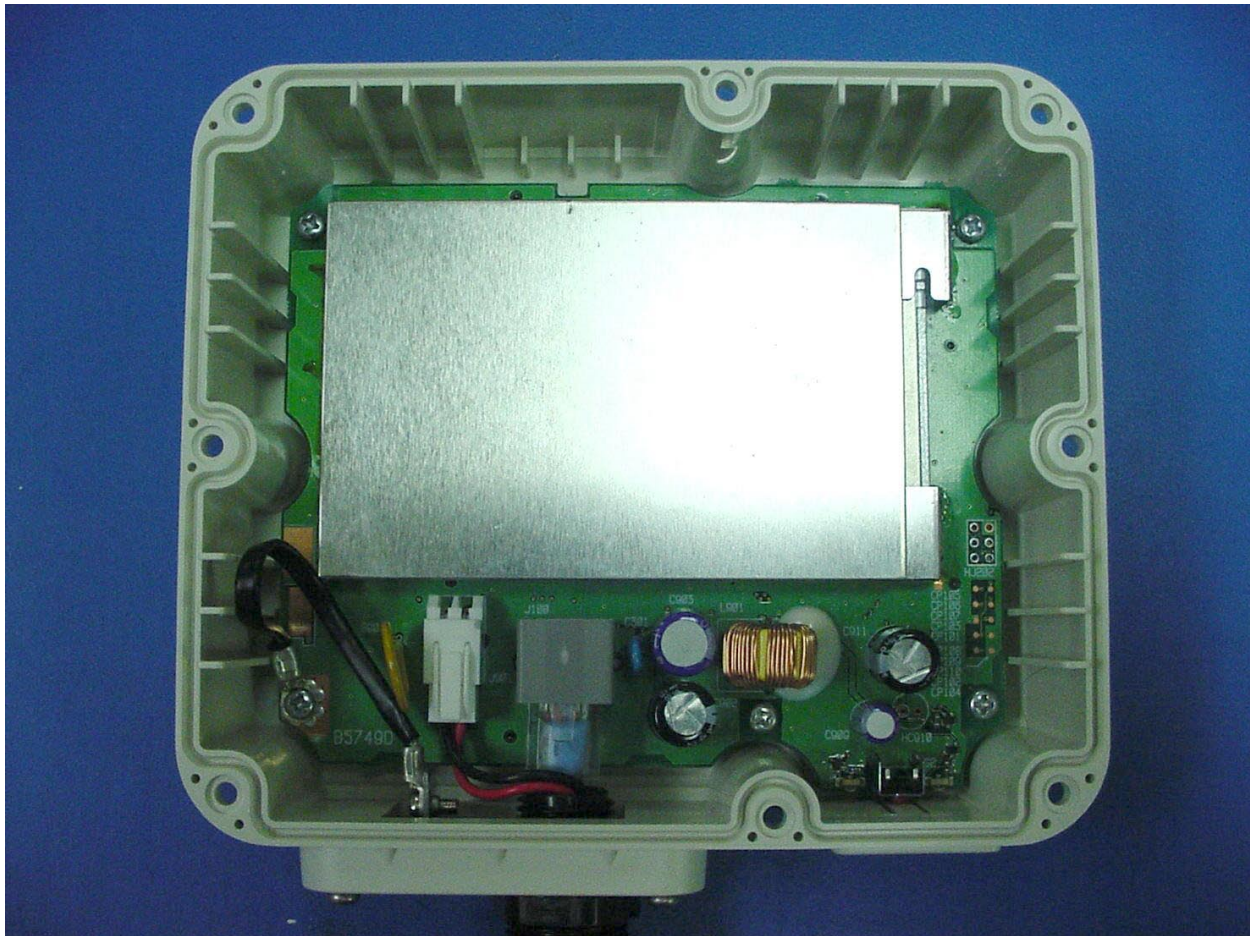
PHOTOGRAPH 16: TOP VIEW WITH COVER REMOVED
