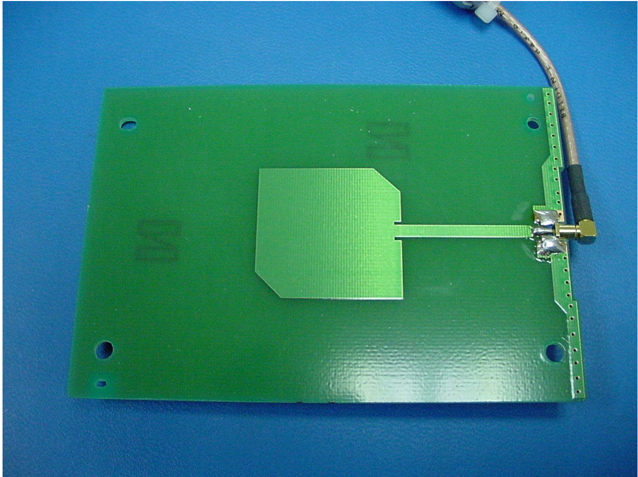
PHOTOGRAPH 15: TOP VIEW OF ANTENNA
