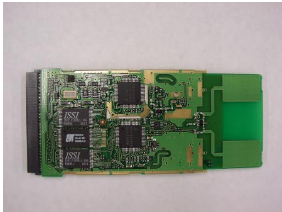
Bottom view of the board without cover
