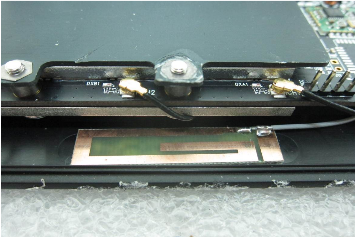
EUT 16 Z-WAVE antenna
