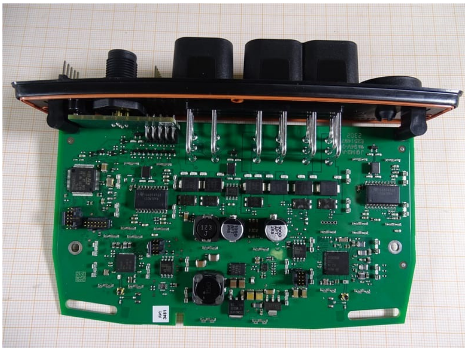
Photo 4: DUT - PCB w/o shielding
