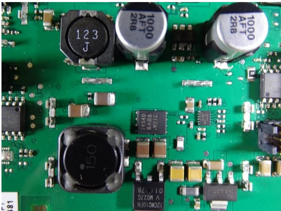
Photo 6: DUT - PCB w/o shielding
