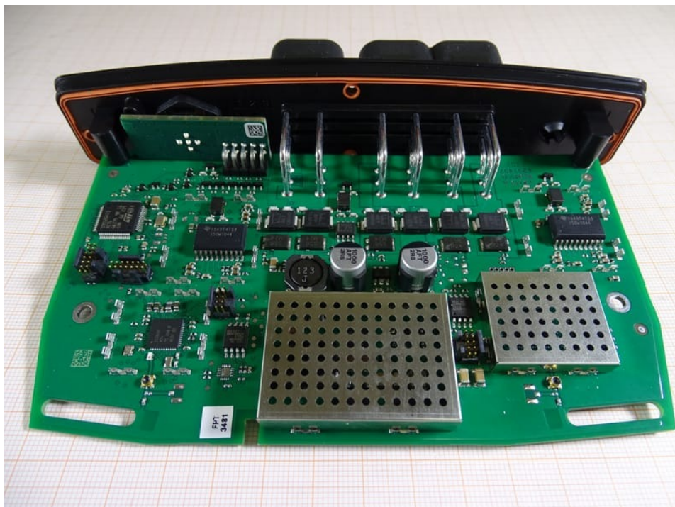
Photo 2: DUT - PCB view
