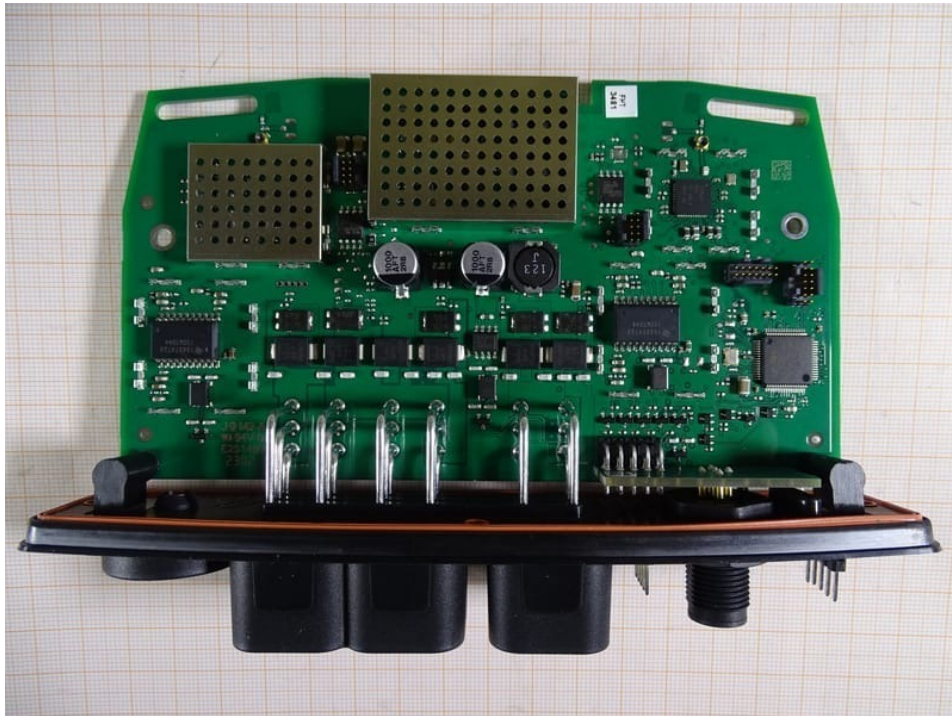
Photo 1: DUT - PCB view
