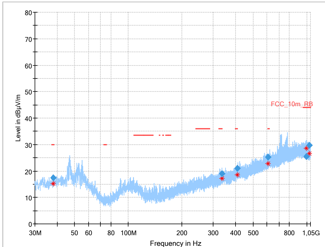
Plot 4: 30 MHz to 1 GHz, TX mode, 2404 MHz, vertical & horizontal polarization, 2 Msps
