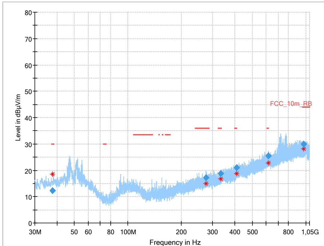
Plot 2: 30 MHz to 1 GHz, TX mode, 2440 MHz, vertical & horizontal polarization, 1 Msps
