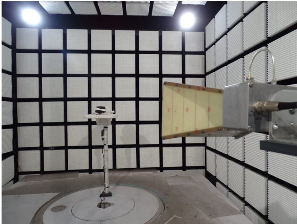
Photo 5: RSE setup 9 kHz to 30 MHz and > 1 GHz
