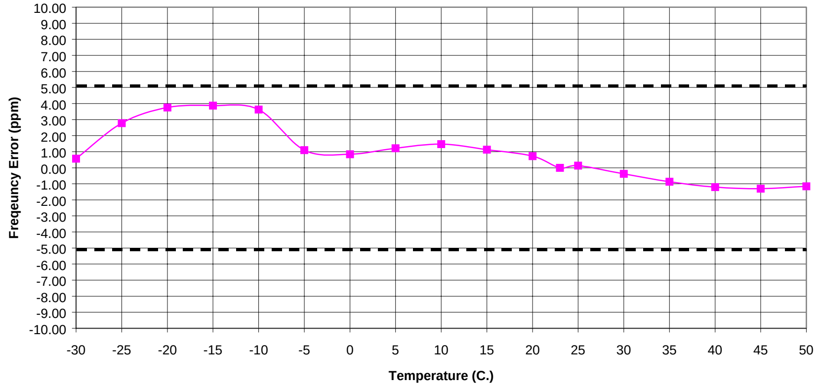
RQT-150 Frequency vs. Temperature
