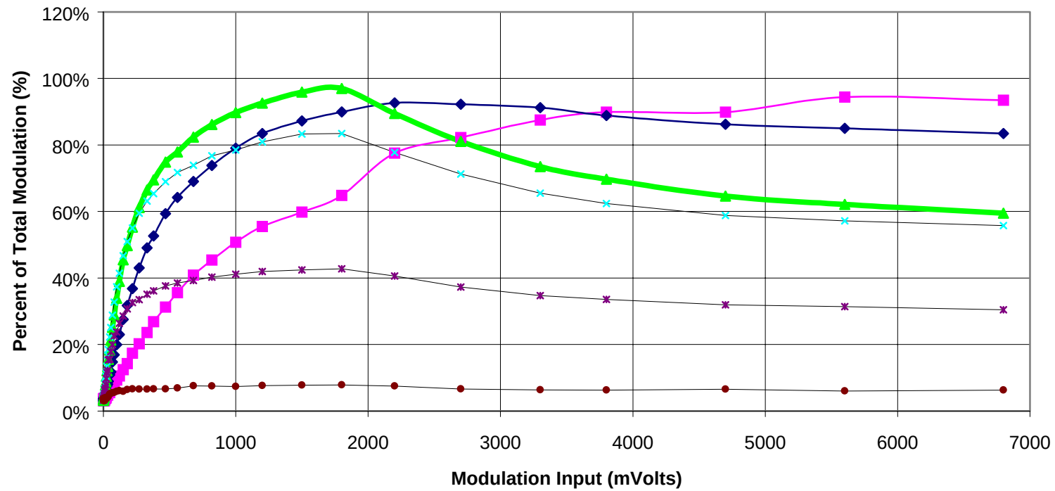
Percent of Modulation vs. Modulation Input Voltage
