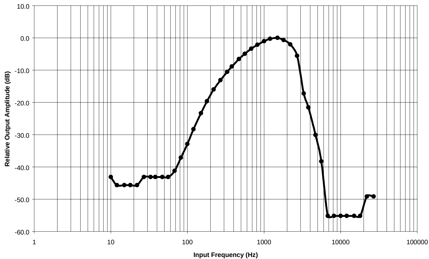
FCC ID: AIERIT10-450 Modulation Low Pass Filter Response
