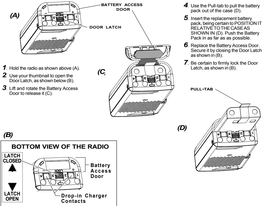
FIG-5: BATTERY ACCESS & INSTALLATION:
